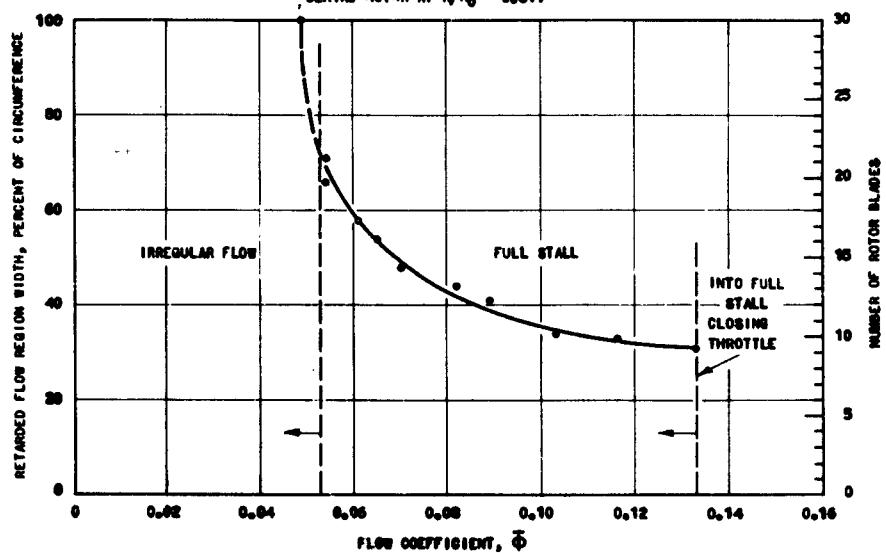
FIGURE 43 VARIATION OF RETARDED FLOW REGION WIDTH WITH FLOW COEFFICIENT ONE-STAGE SOLID BODY BLADING - 750 RPM BEHIND ROTOR AT R/R_0 = 0.611
