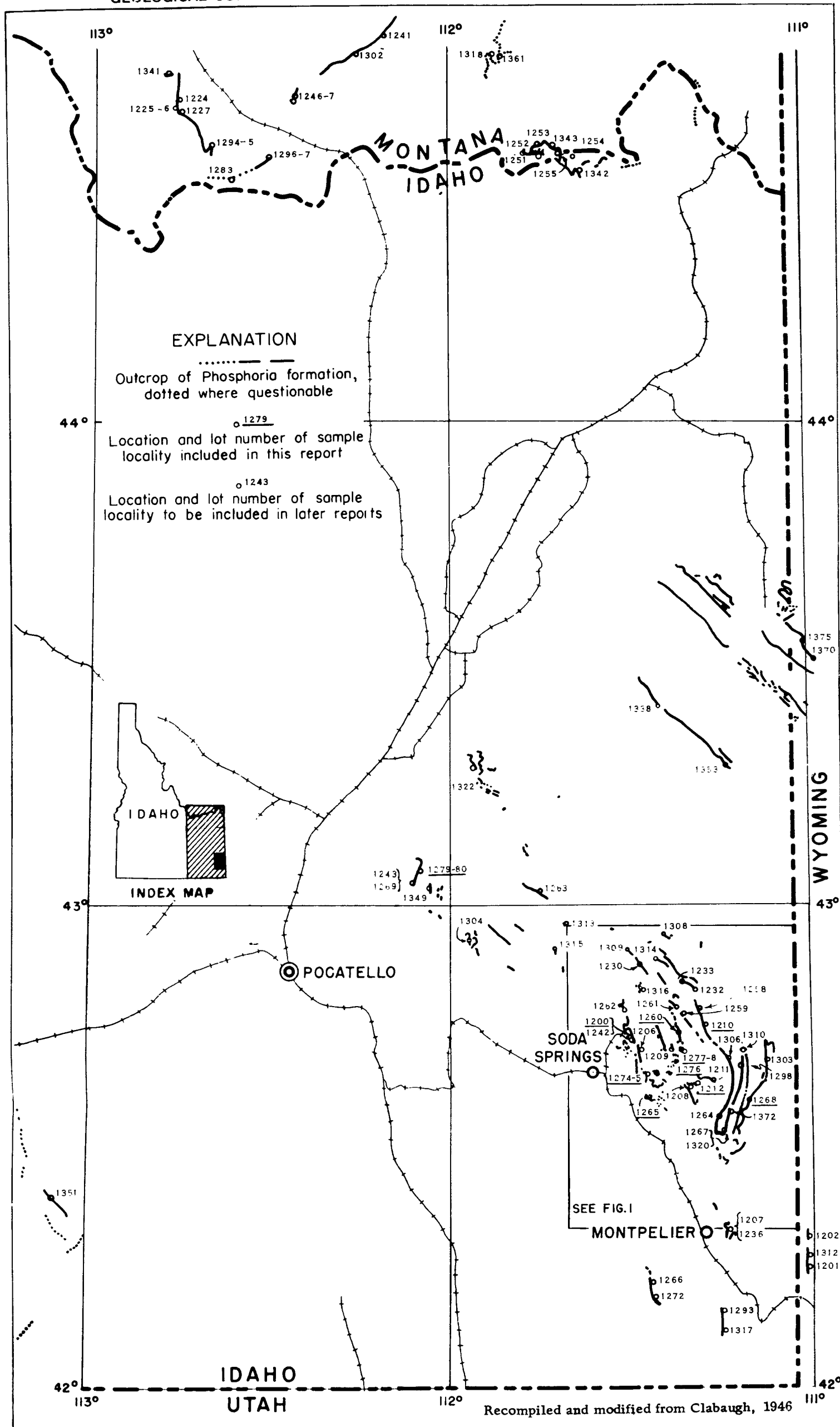
PHOSPHORIA FORMATION OUTCROPS IN IDAHO AND LOCALITIES SAMPLED FOR PHOSPHATE
