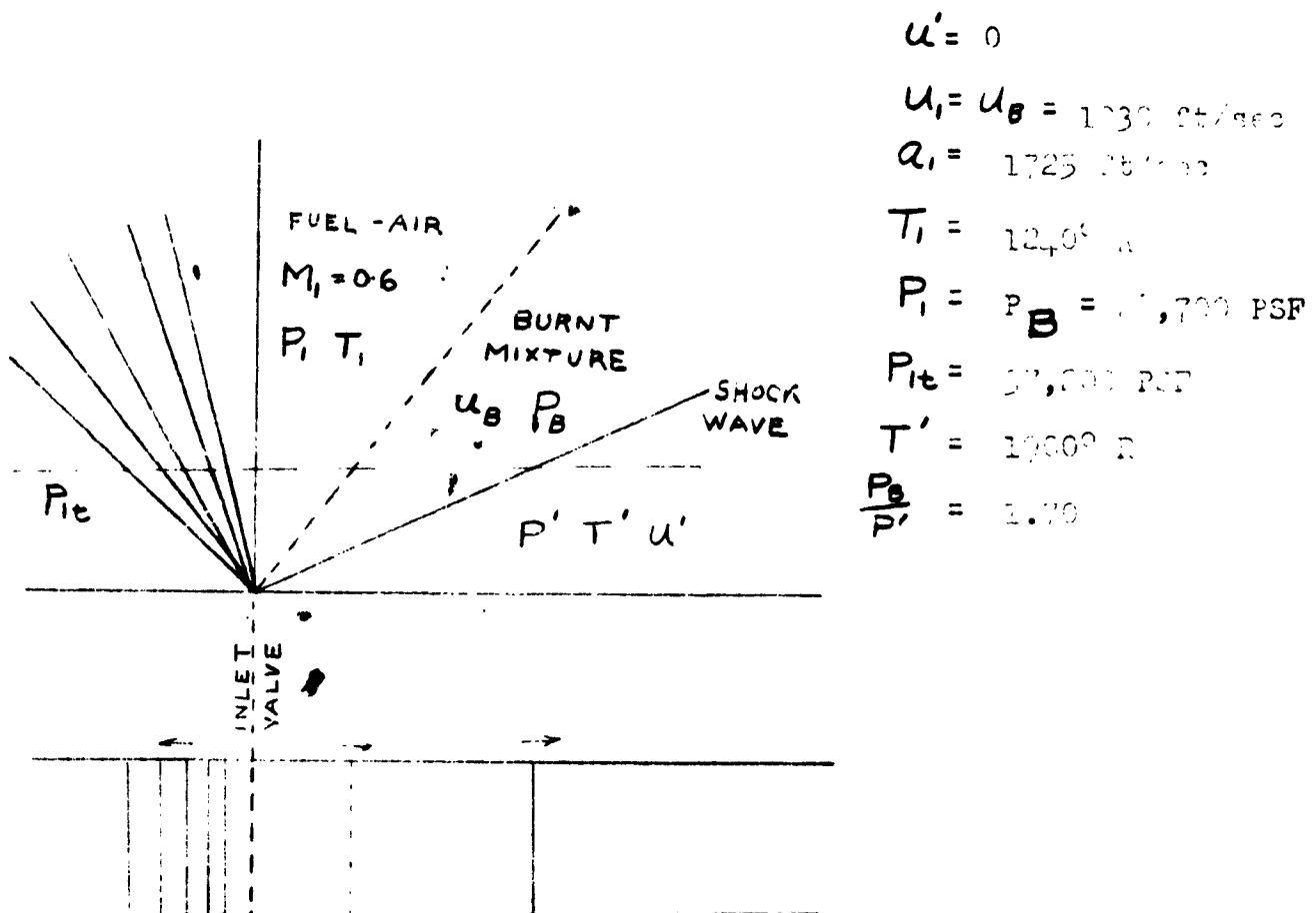
Fig. 52 Wave Configuration Produced when the Inlet Valve Opens
