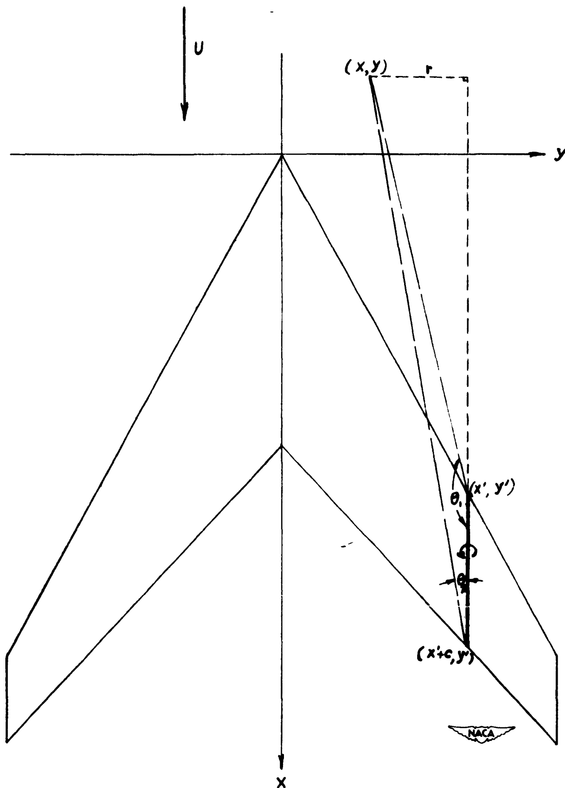
Figure 3.- Geometrical relationships for straight-line chordwise vortex segments that occur with spanwise-varying area loading.
