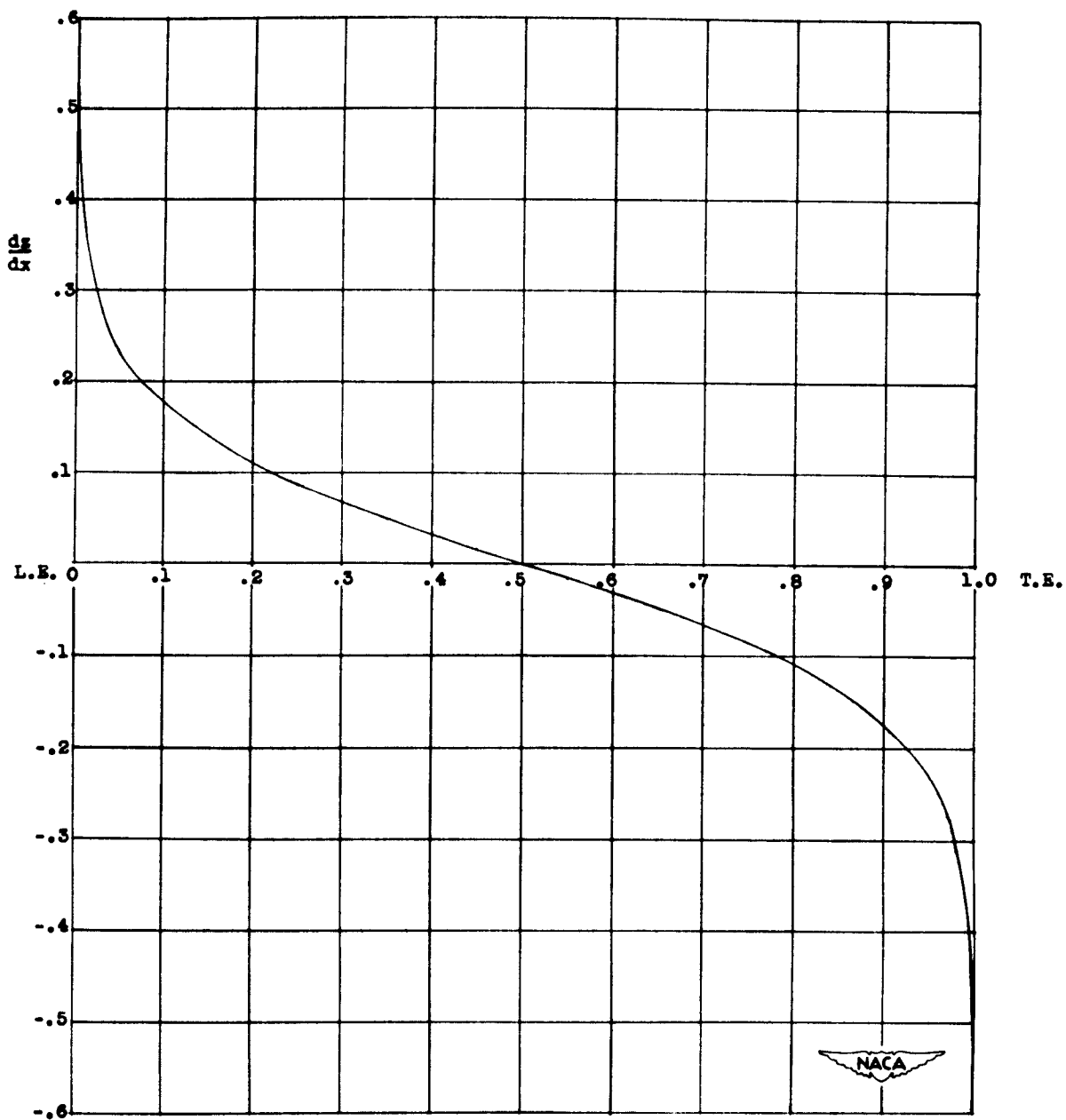
(b) Slopes along NACA a = 1.0 mean line, for c_l = 1.0 , from reference 3.
