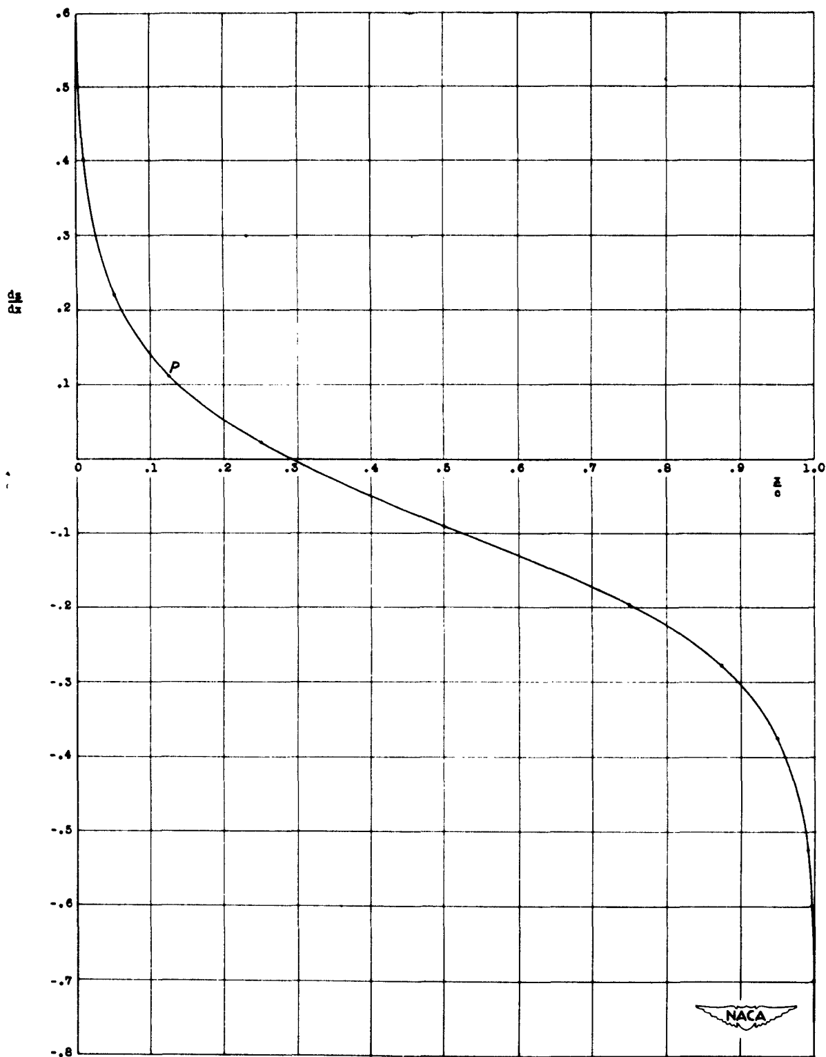
(a) Calculated slopes, example wing.
