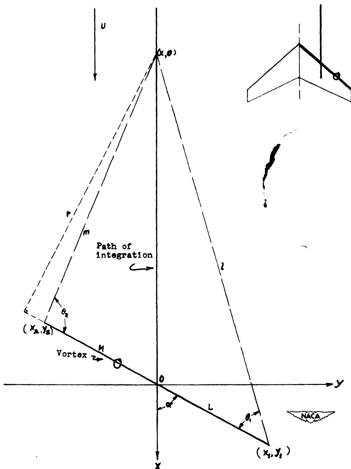
Figure 8.- Geometrical relationships for case I. Heavy lines in small sketch show relative positions of vortex segment and path of integration for this case.
