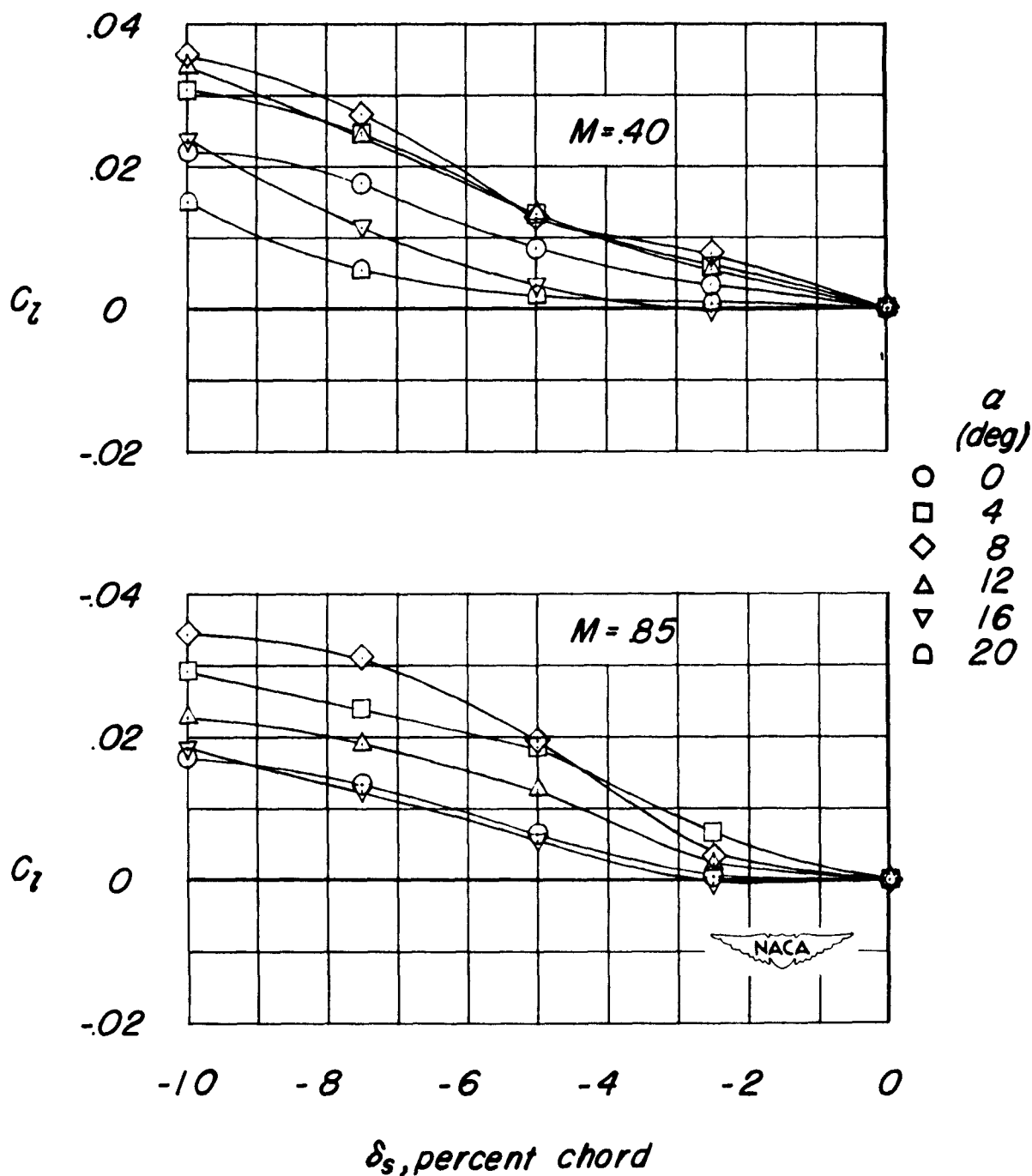
Figure 9.- Variation of rolling-moment coefficient with combined projections of deflector and spoiler in 1.0 to 1.0 ratio for the spoiler-slot-deflector combination. \delta_s = -\delta_d .
