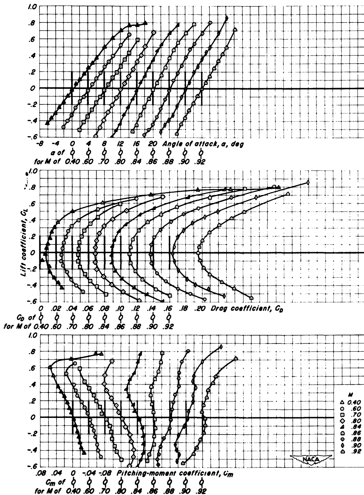
(b) Taper ratio 0.50. Figure 7.- Continued.
