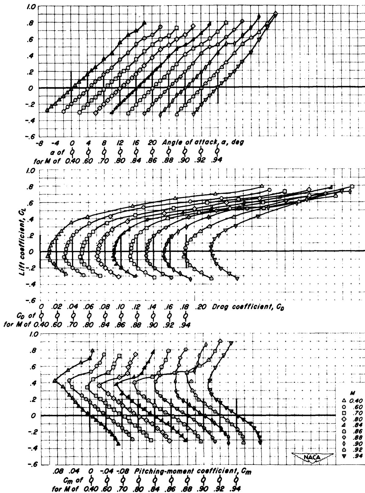
Figure 13- The lift, drag, and pitching-moment characteristics of the aspect ratio 2 wings in combination with the cylindrical body.
