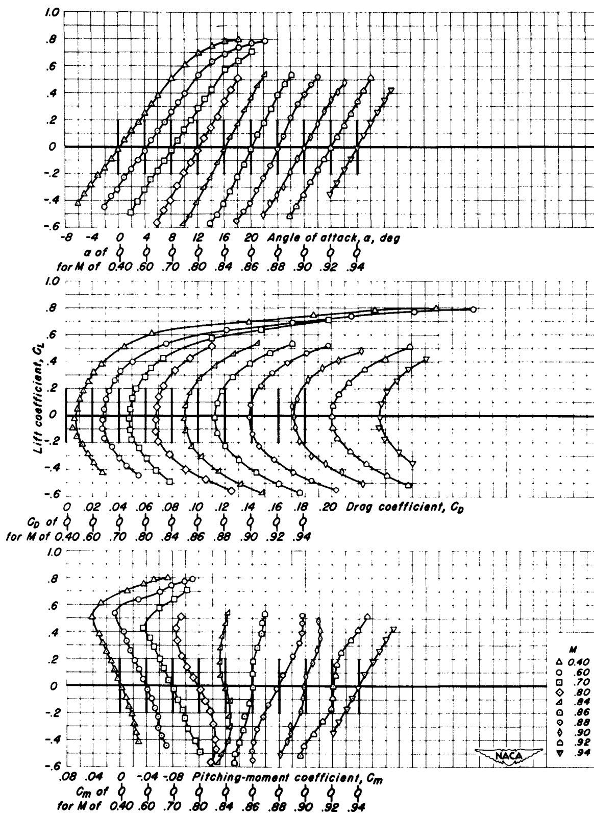
Figure 5.- The lift, drag, and pitching-moment characteristics of the aspect ratio 4 wings in combination with the small body having a fineness ratio of 9.
