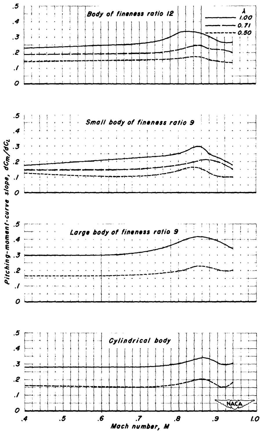
(c) Aspect ratio 2. Figure 19.- Concluded.
