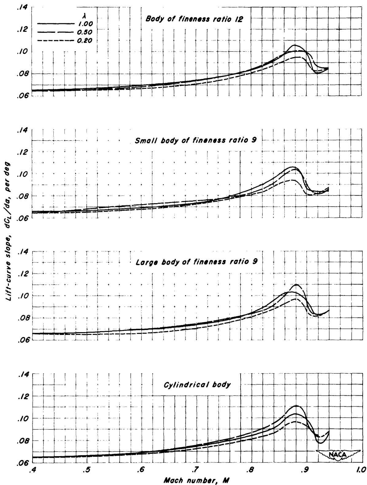
Figure 17.-The variation of lift-curve slope, at zero lift, with Mach number for the wing-body combinations.
