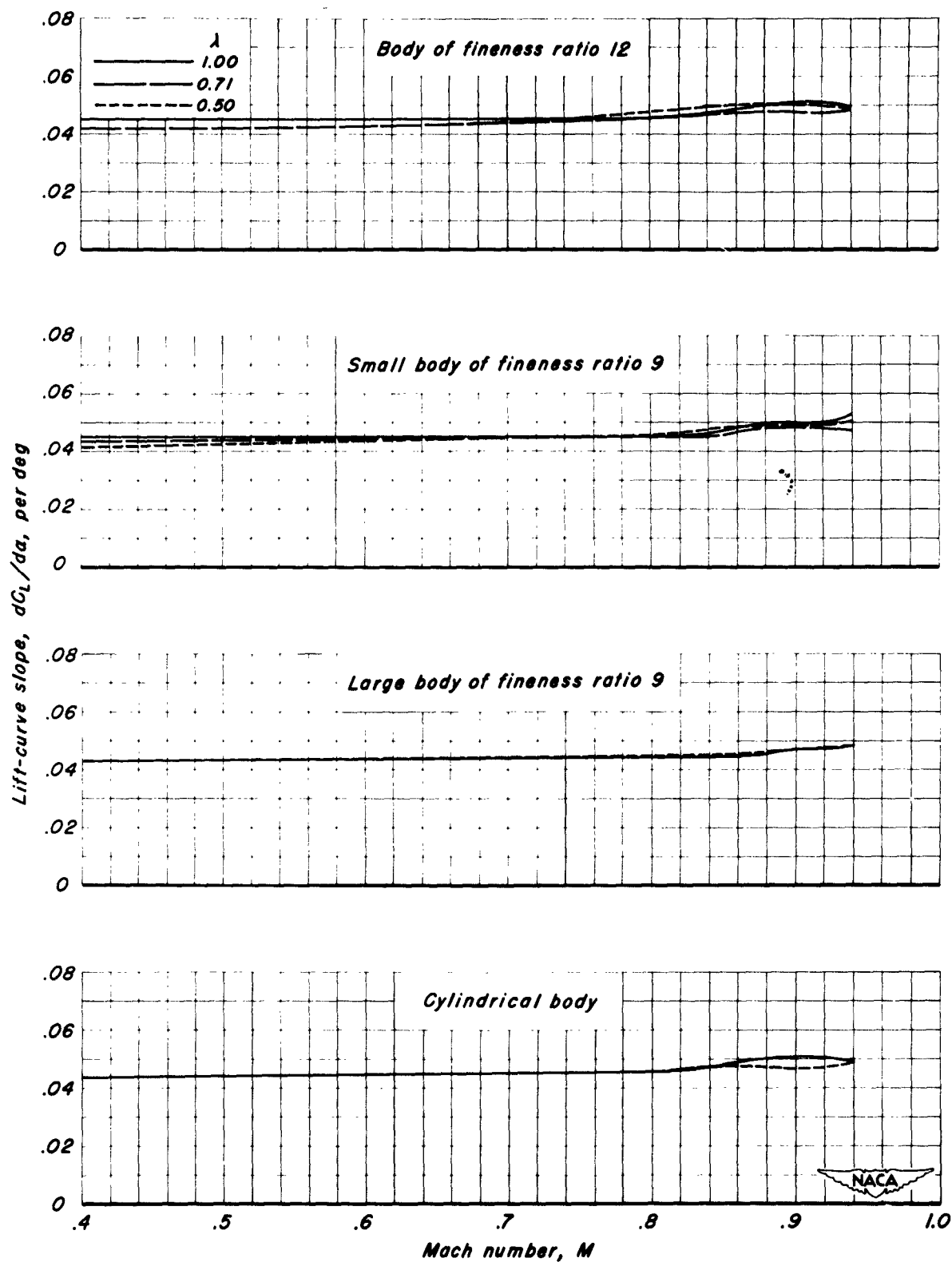
(c) Aspect ratio 2. Figure 17.- Concluded.
