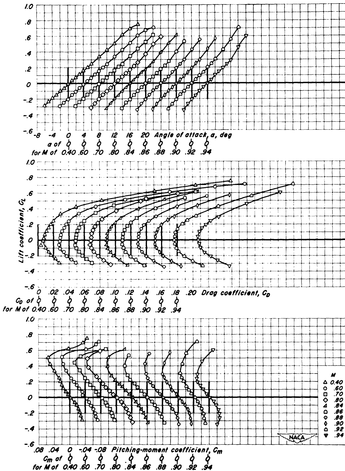
(b) Taper ratio 0.50. Figure 13.- Concluded.
