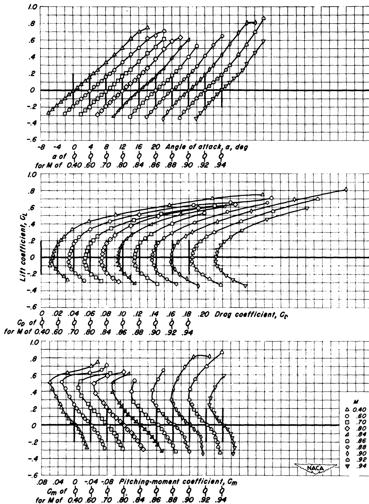
(b) Taper ratio 0.50. Figure 12.- Concluded.
