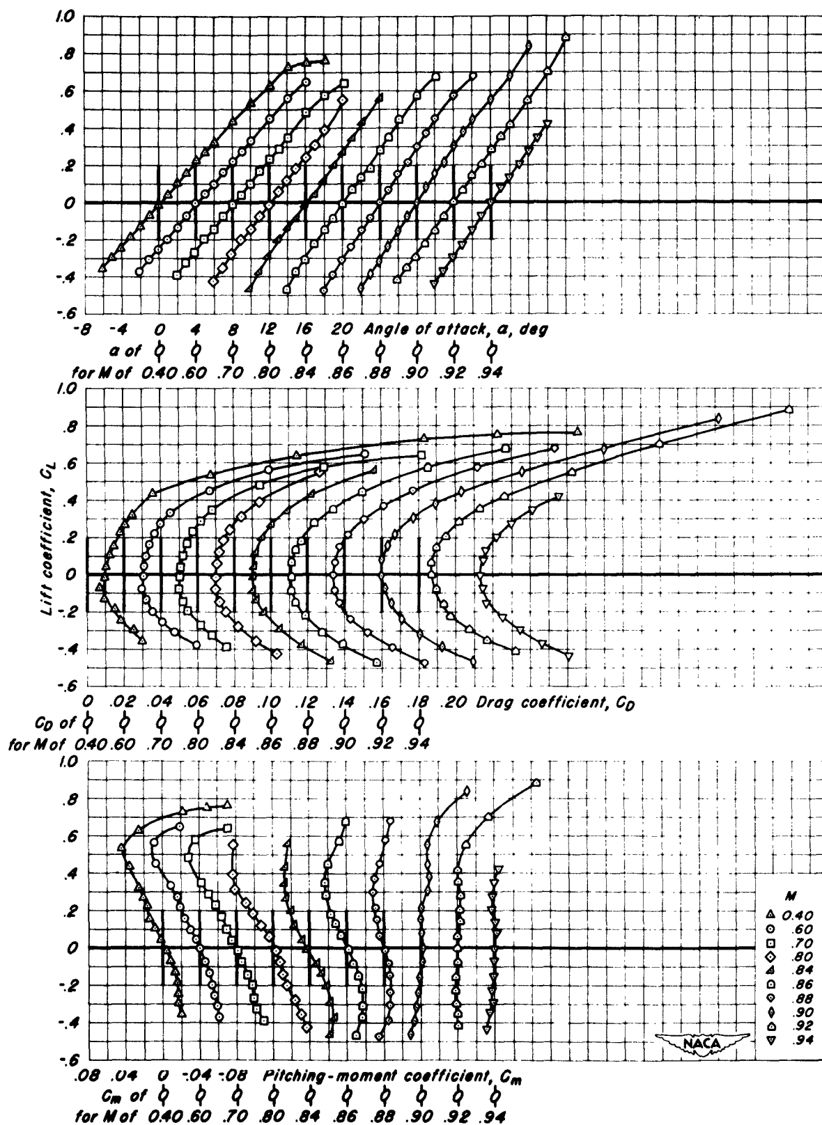
(c) Taper ratio 0.33. Figure 8.- Concluded.
