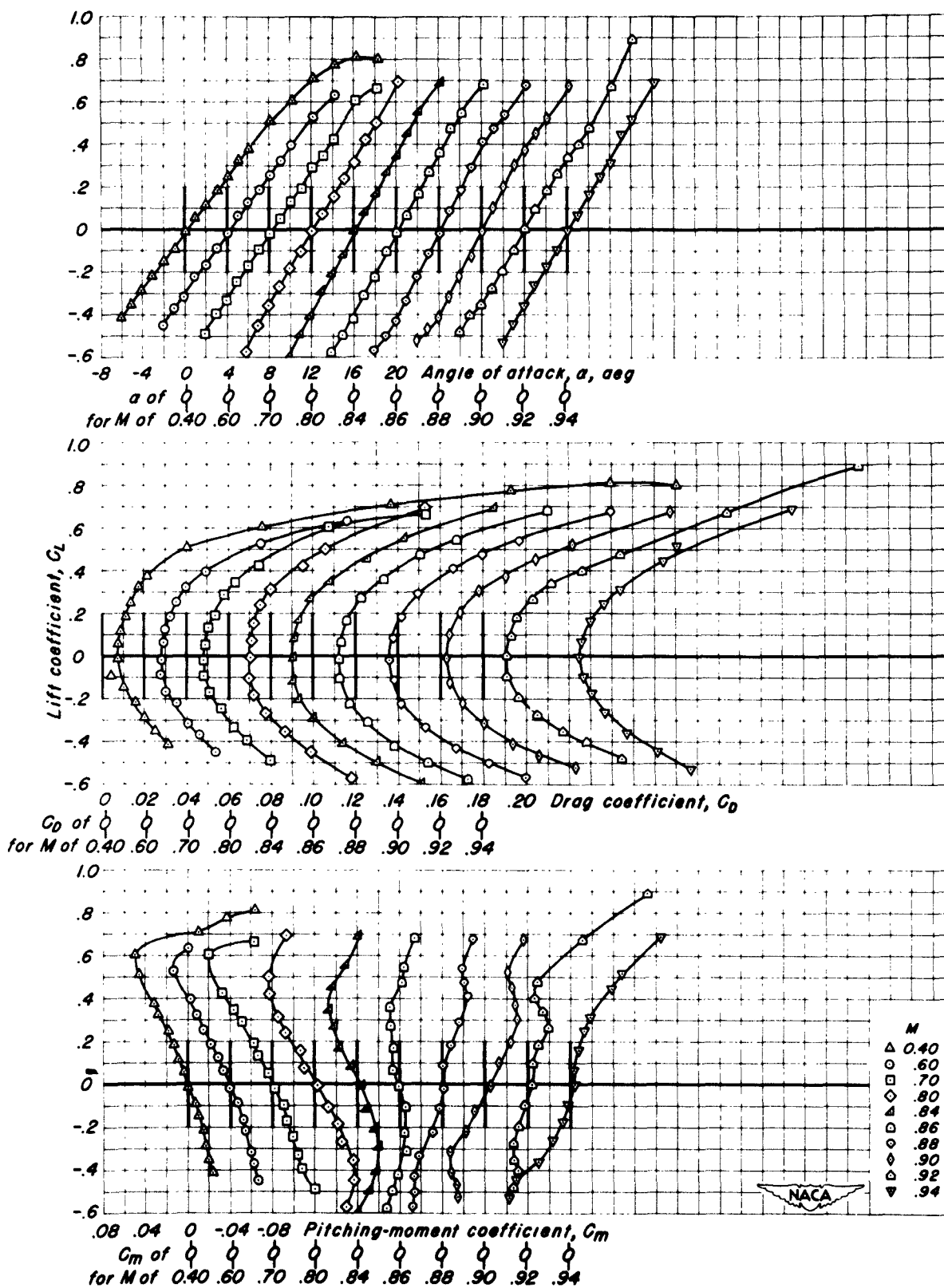
(b) Taper ratio 0.50. Figure 4.- Continued.
