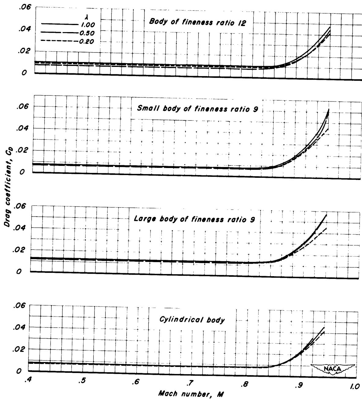
(a) Aspect ratio 4. Figure 14.- The variation of drag coefficient, at zero lift, with Mach number for the wing-body combinations.
