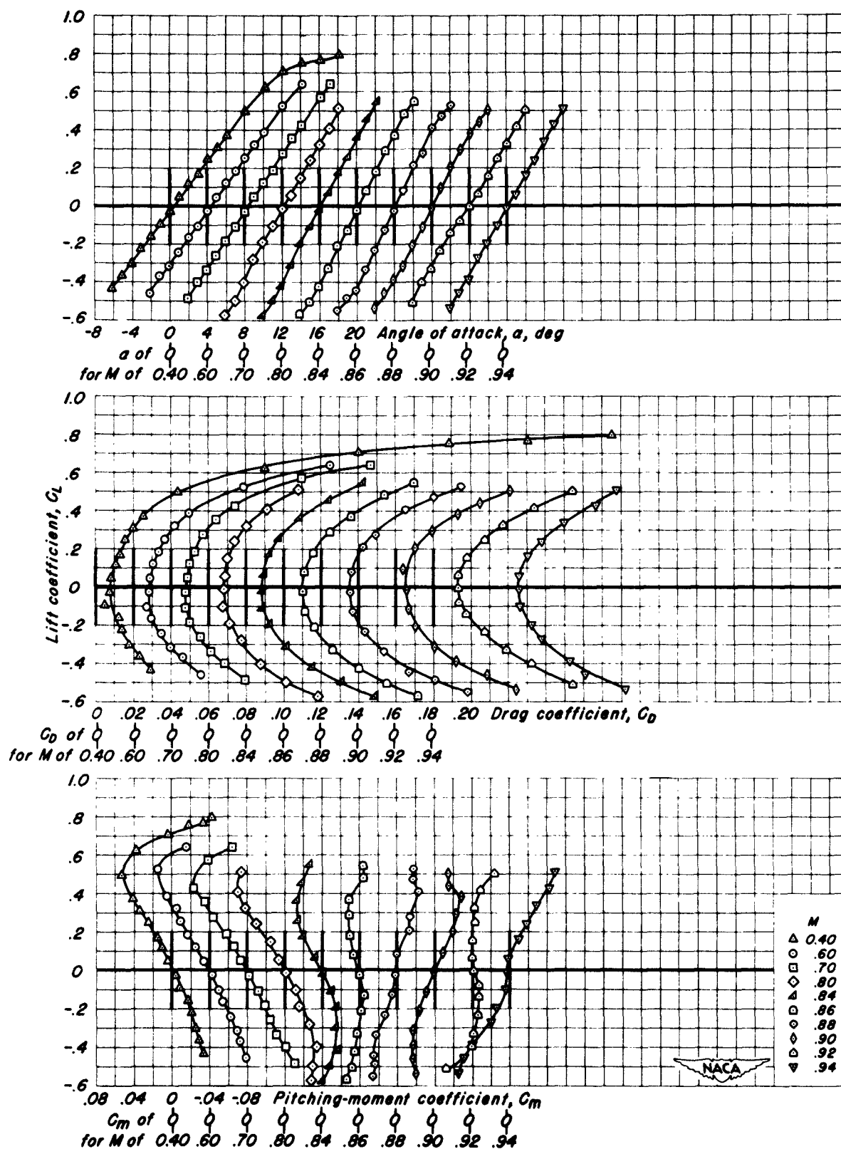
Figure 7.- The lift, drag, and pitching-moment characteristics of the aspect ratio 4 wings in combination with the cylindrical body.
