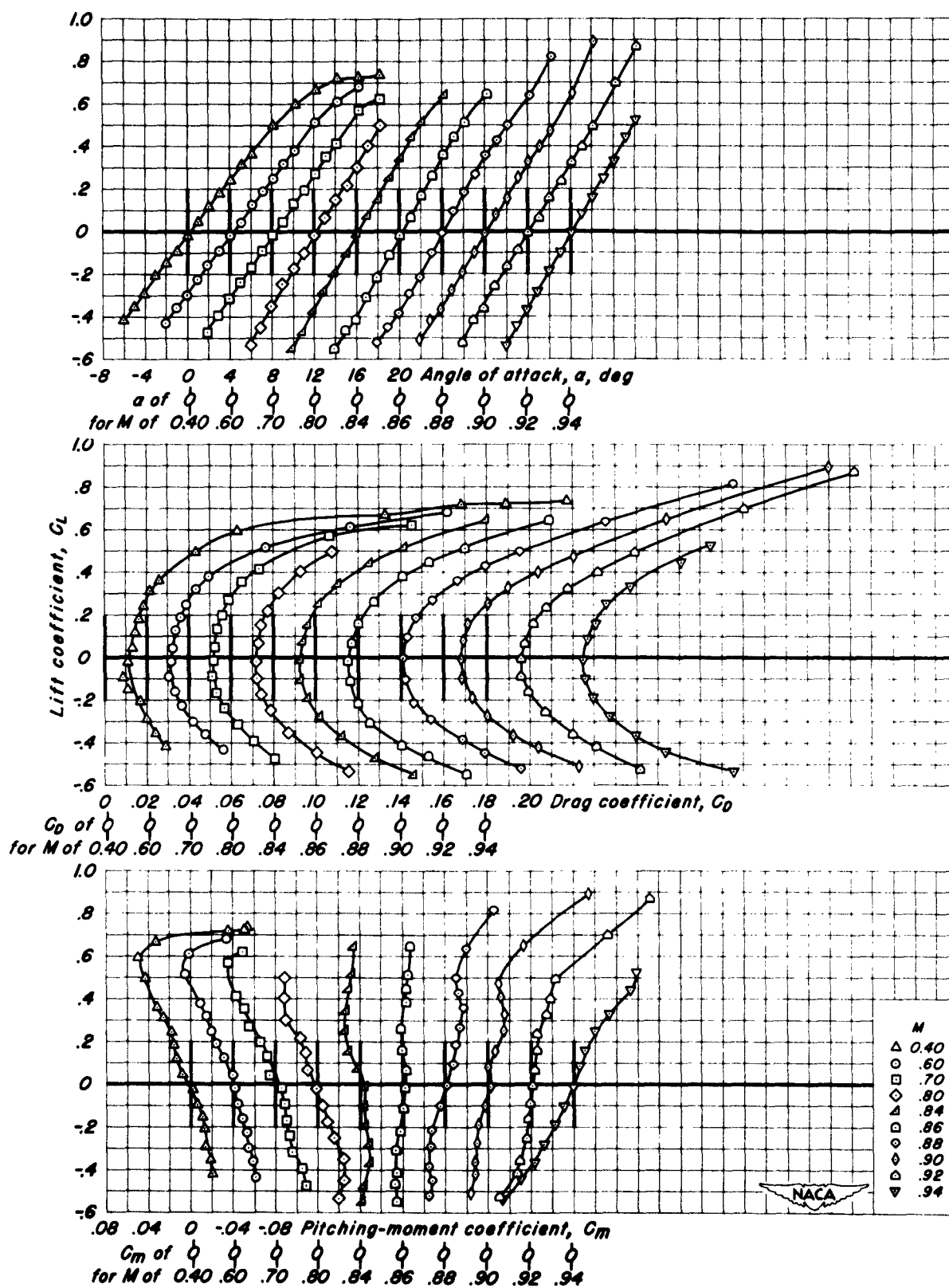
(c) Taper ratio 0.20. Figure 6.- Concluded.
