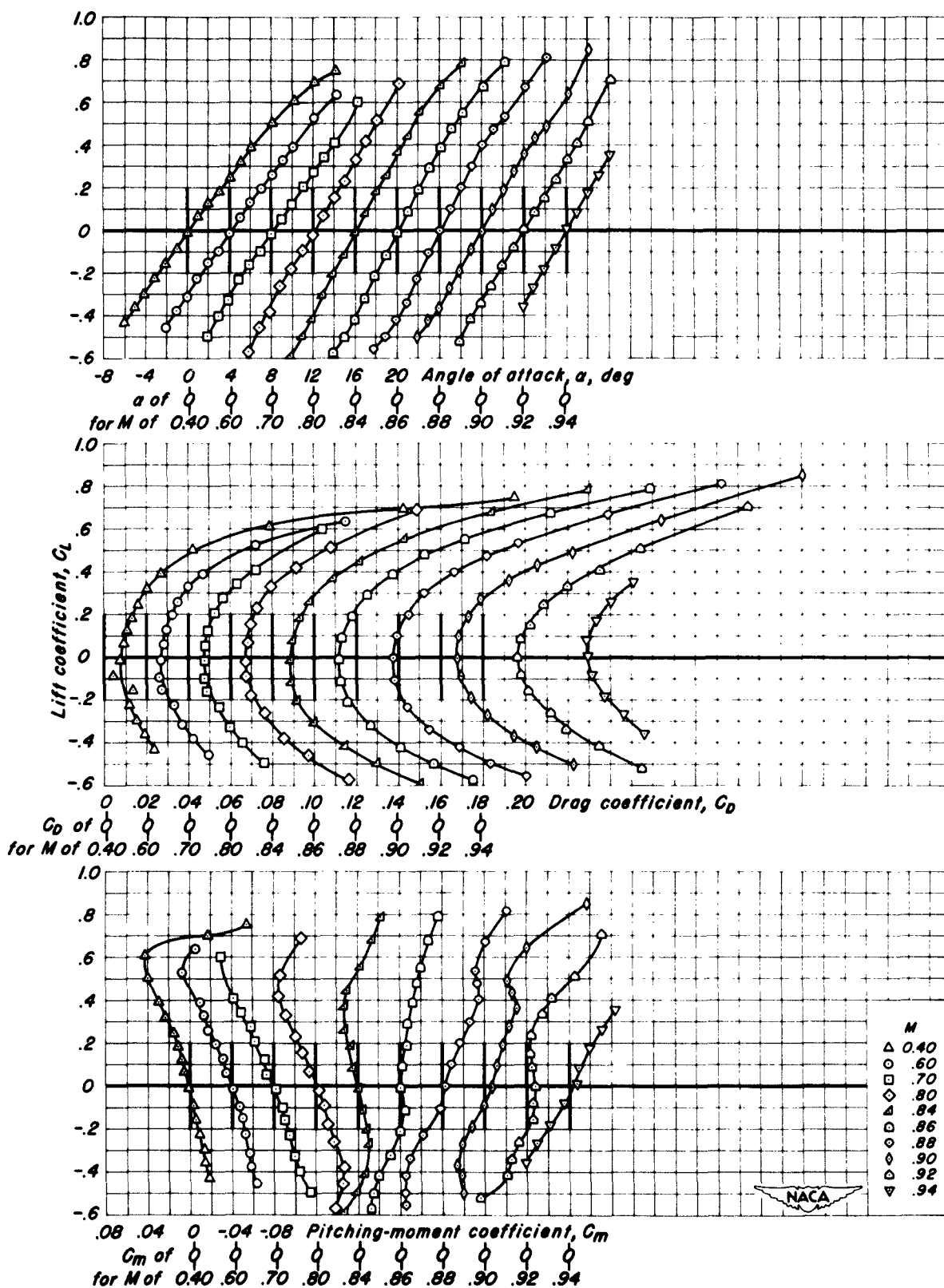
(b) Taper ratio 0.50. Figure 5.- Continued.
