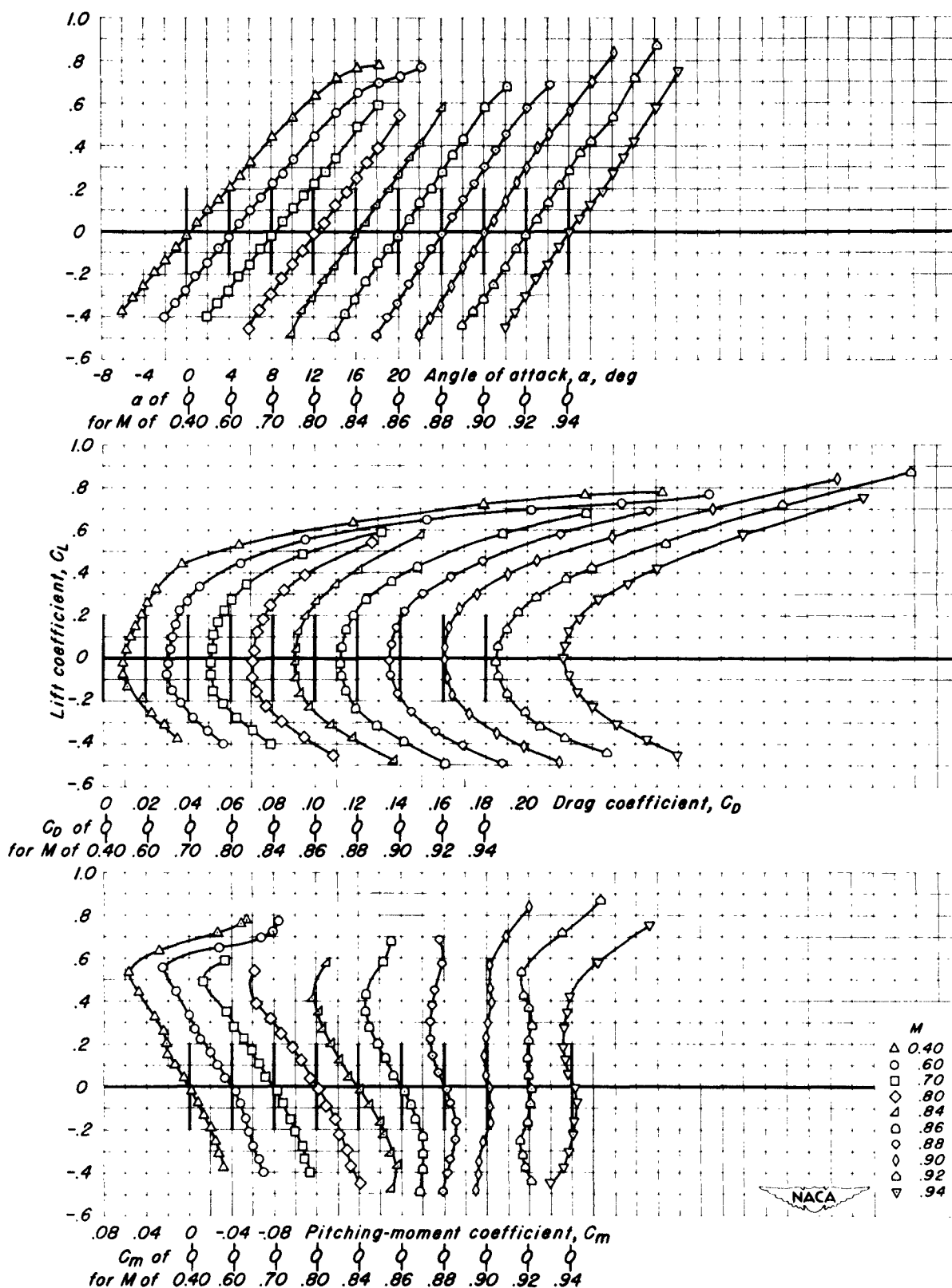
(b) Taper ratio 0.60. Figure 8.- Continued.
