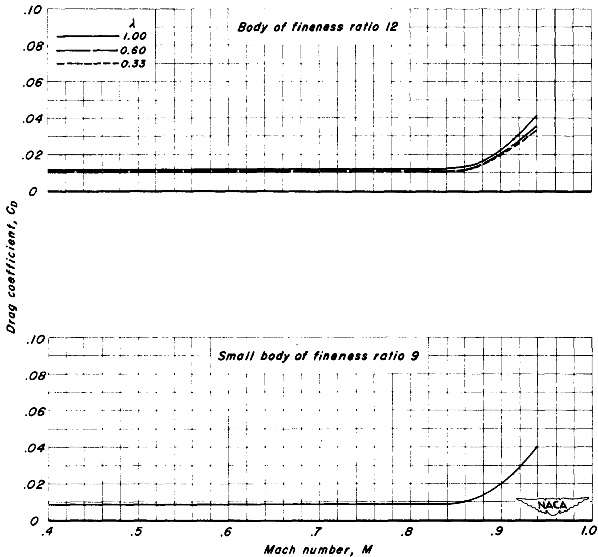
(b) Aspect ratio 3. Figure 14.- Continued.
