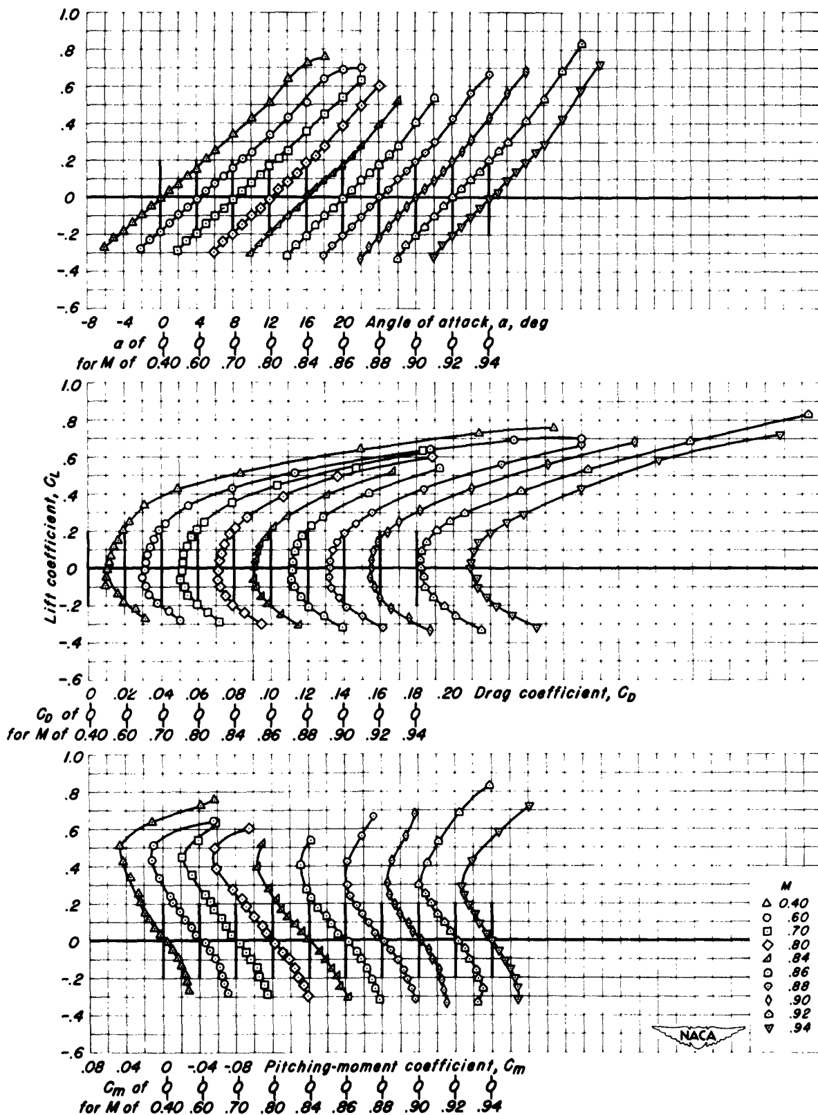
(c) Taper ratio 0.50. Figure 10.- Concluded.
