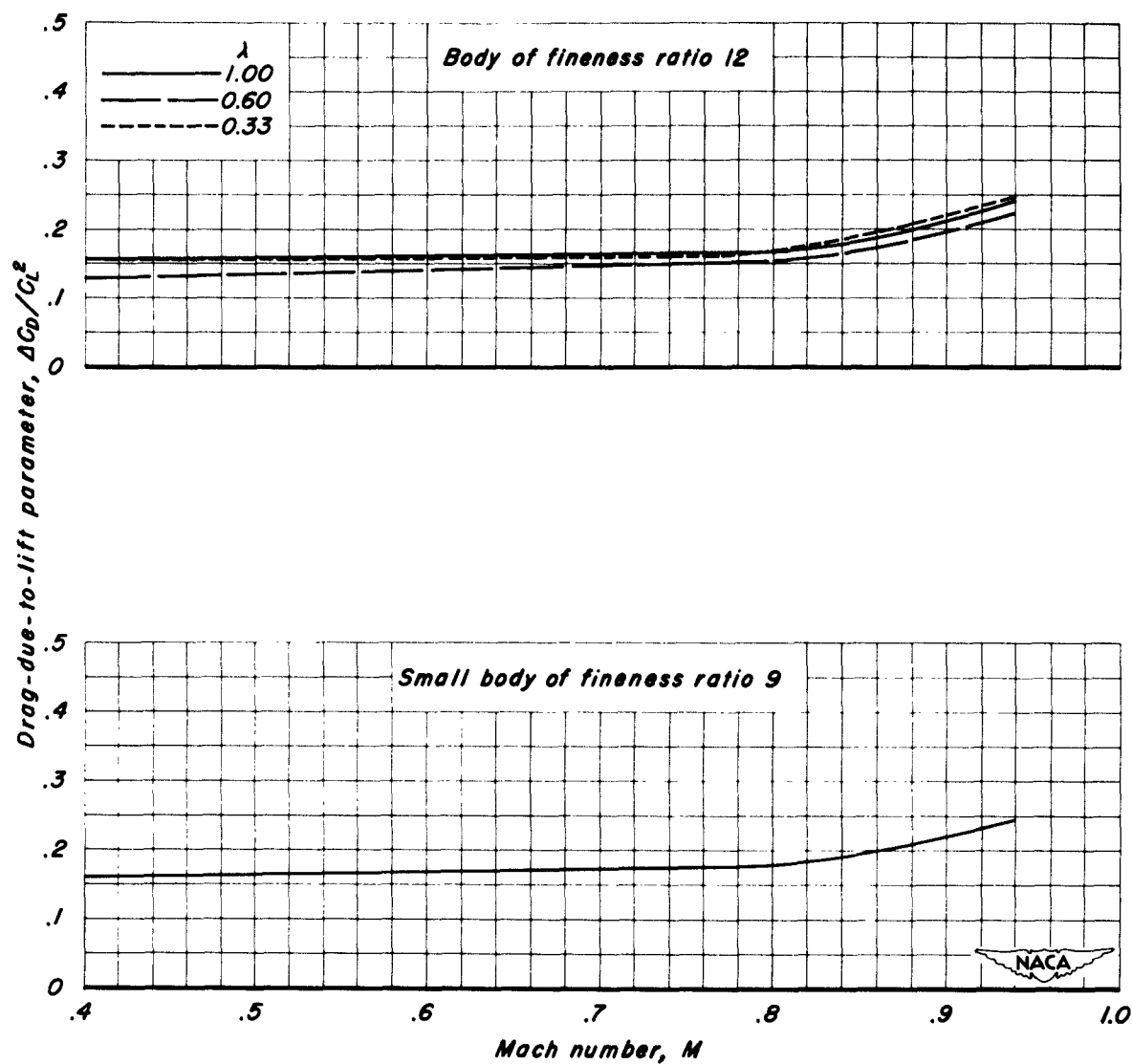
(b) Aspect ratio 3. Figure 16.- Continued.
