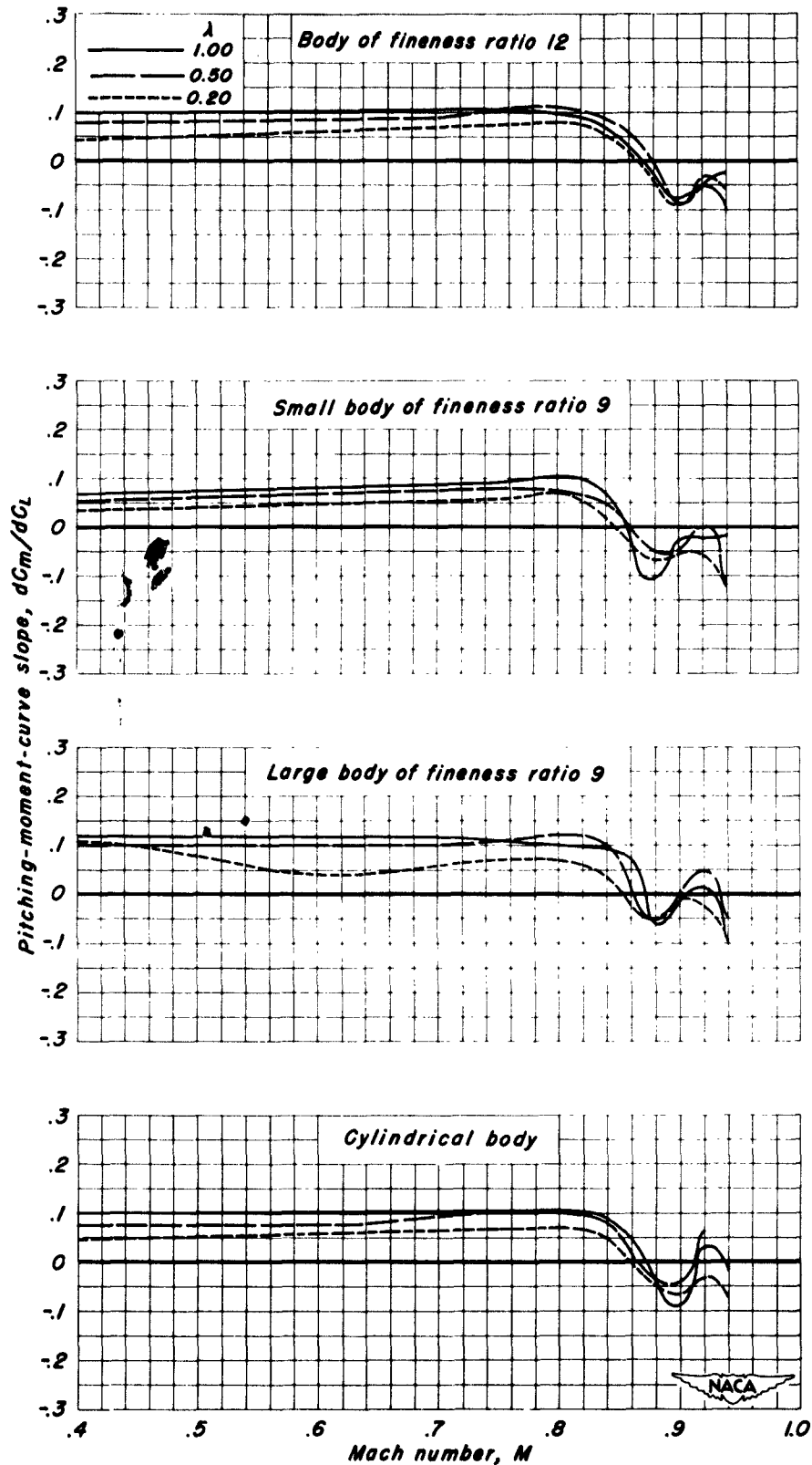
Figure 19.— The variation of pitching-moment-curve slope, at zero lift, with Mach number for the wing-body combinations.
