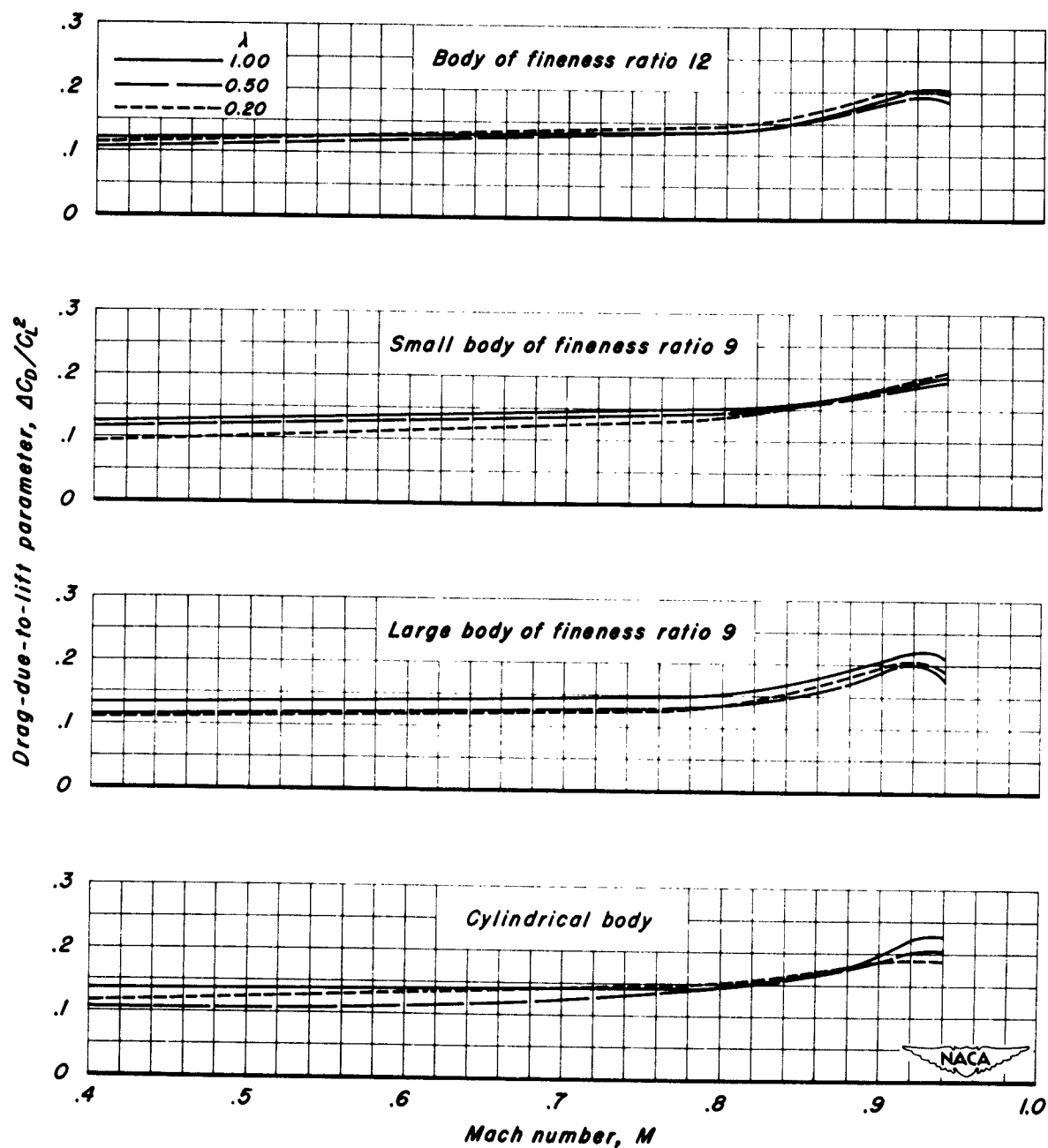
Figure 16.- The variation of drag due to lift parameter with Mach number.
