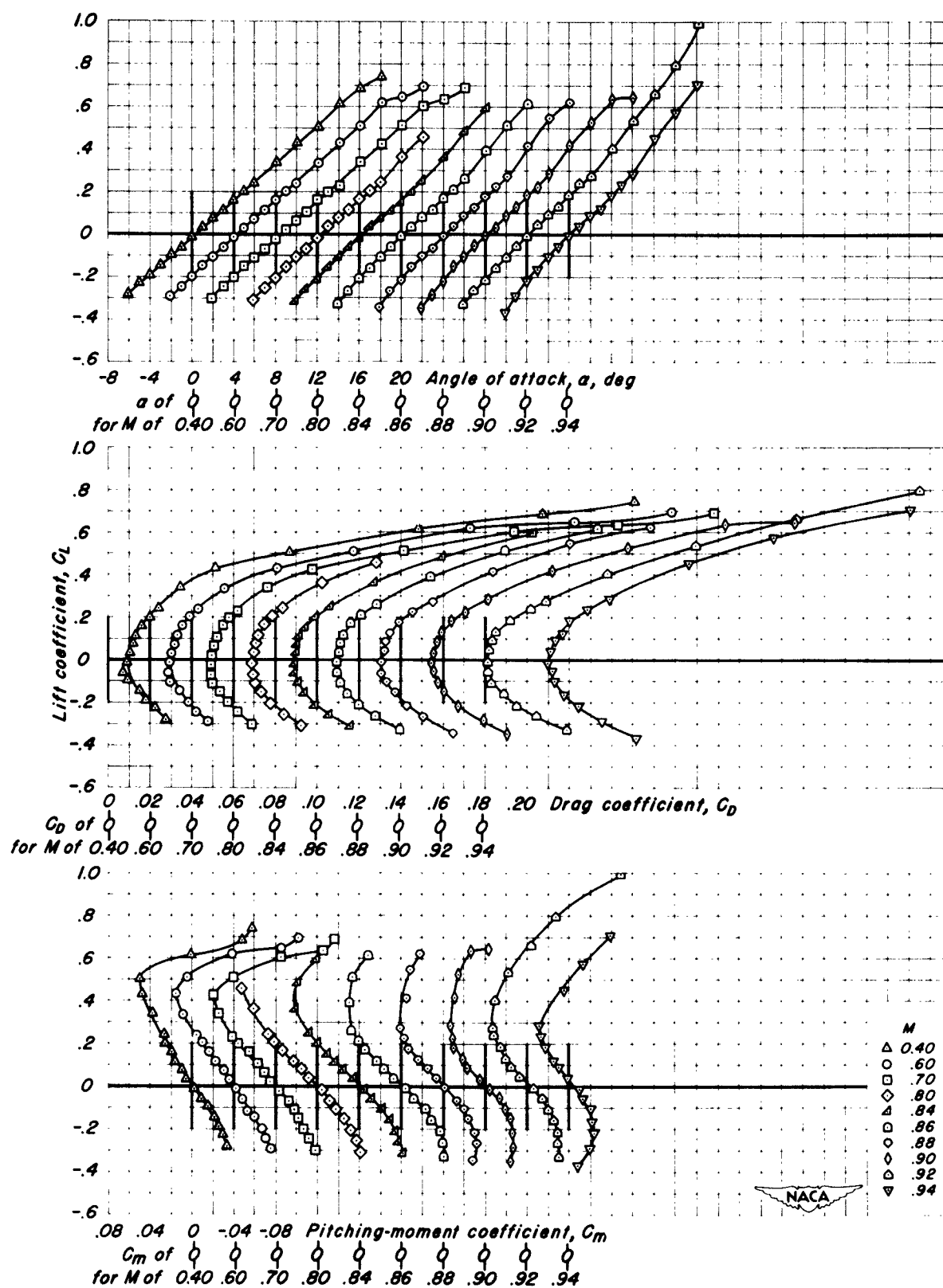
(b) Taper ratio 0.71. Figure 11.- Continued.
