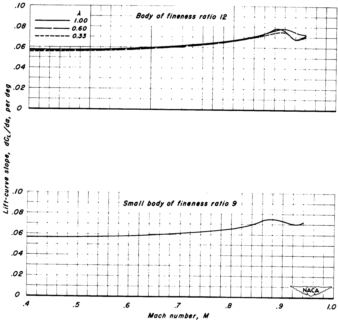
(b) Aspect ratio 3. Figure 17.- Continued.
