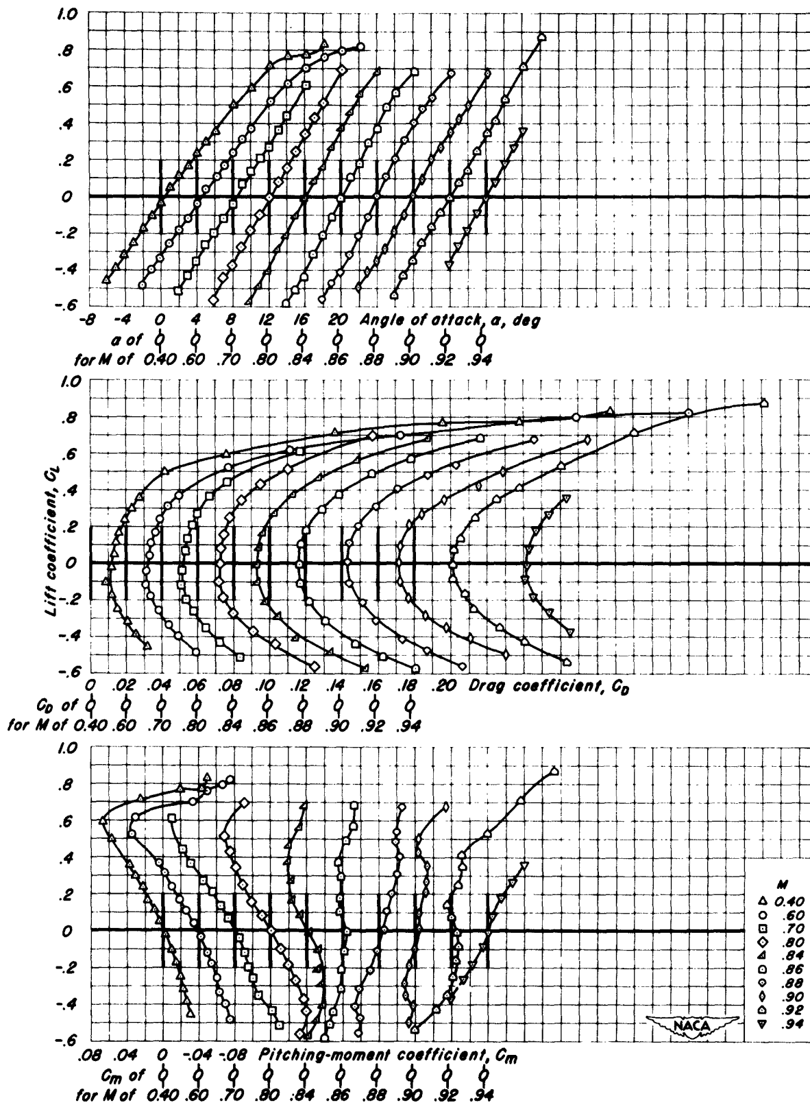
(b) Taper ratio 0.50. Figure 6.- Continued.
