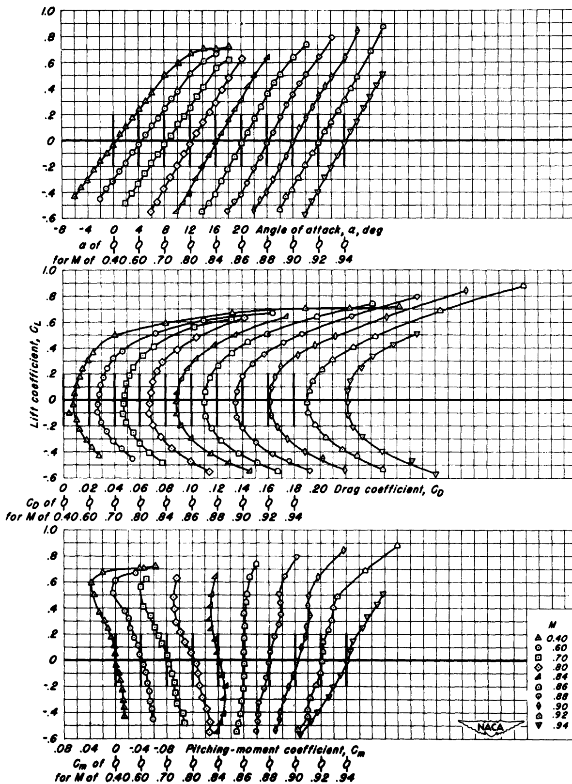
(c) Taper ratio 0.20. Figure 7.- Concluded.
