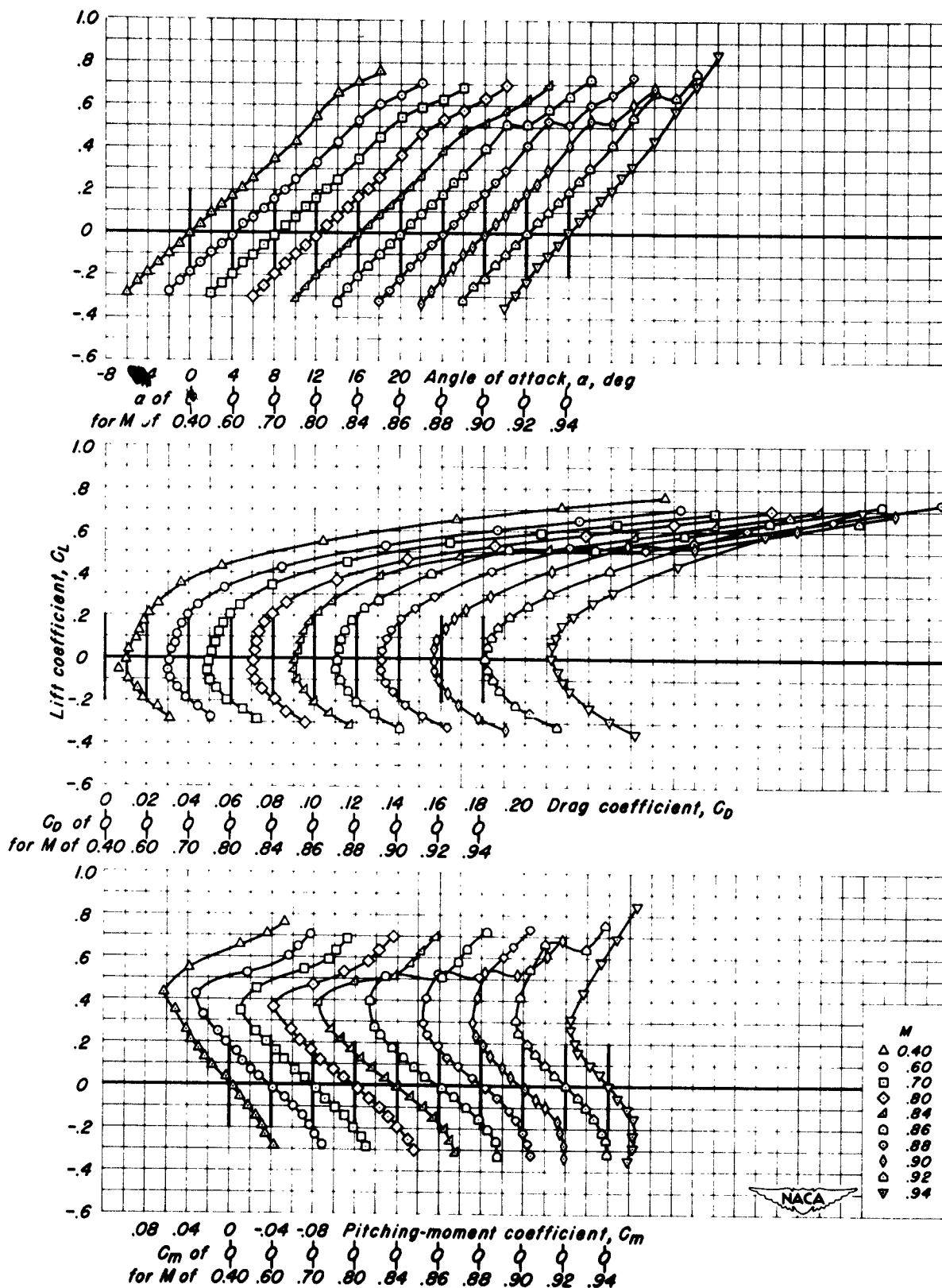
Figure 11.-The lift, drag, and pitching-moment characteristics of the aspect ratio 2 wings in combination with the small body having a fineness ratio of 9.
