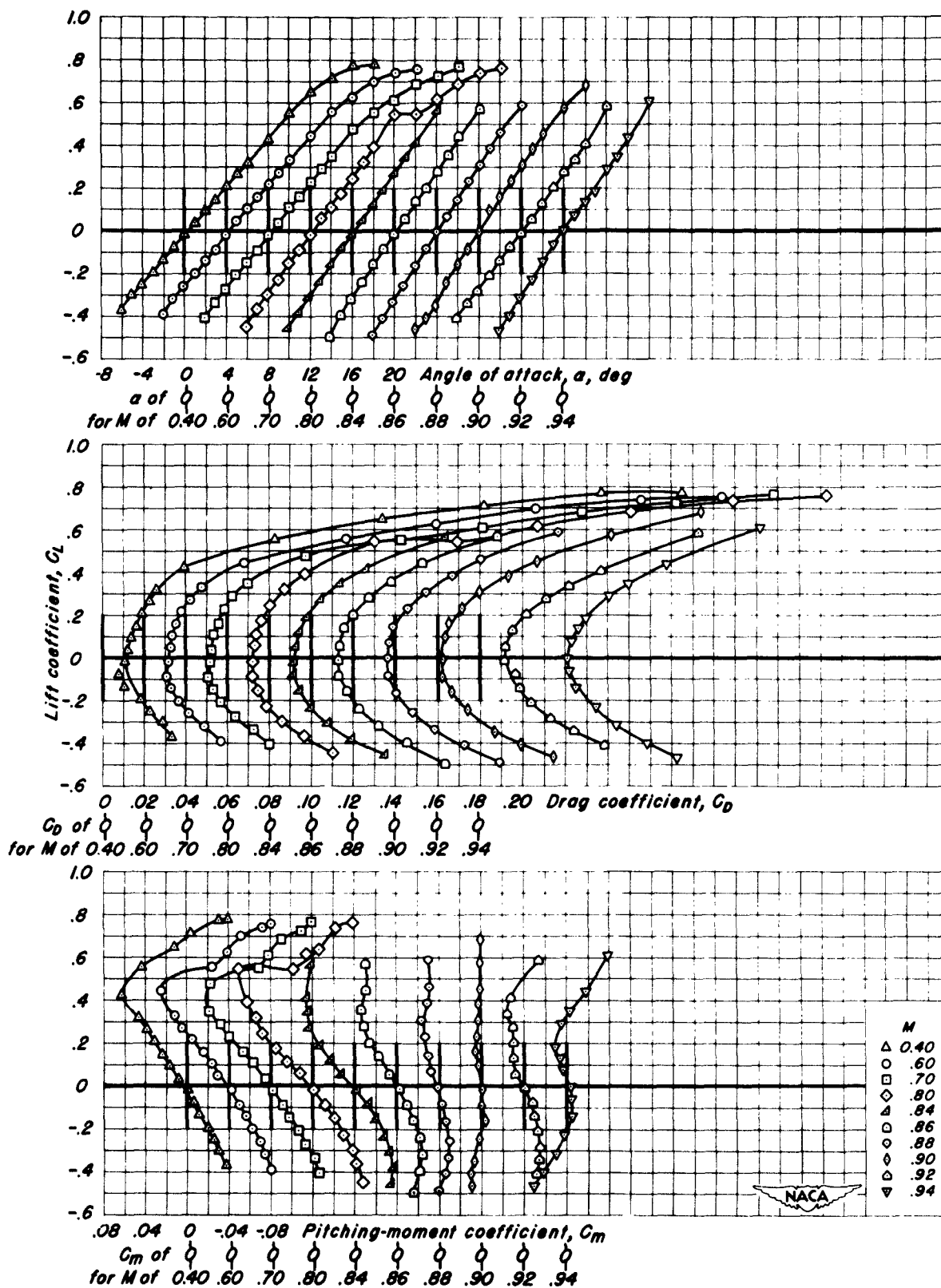
Figure 8.- The lift, drag, and pitching-moment characteristics of the aspect ratio 3 wings in combination with the body having a fineness ratio of 12.
