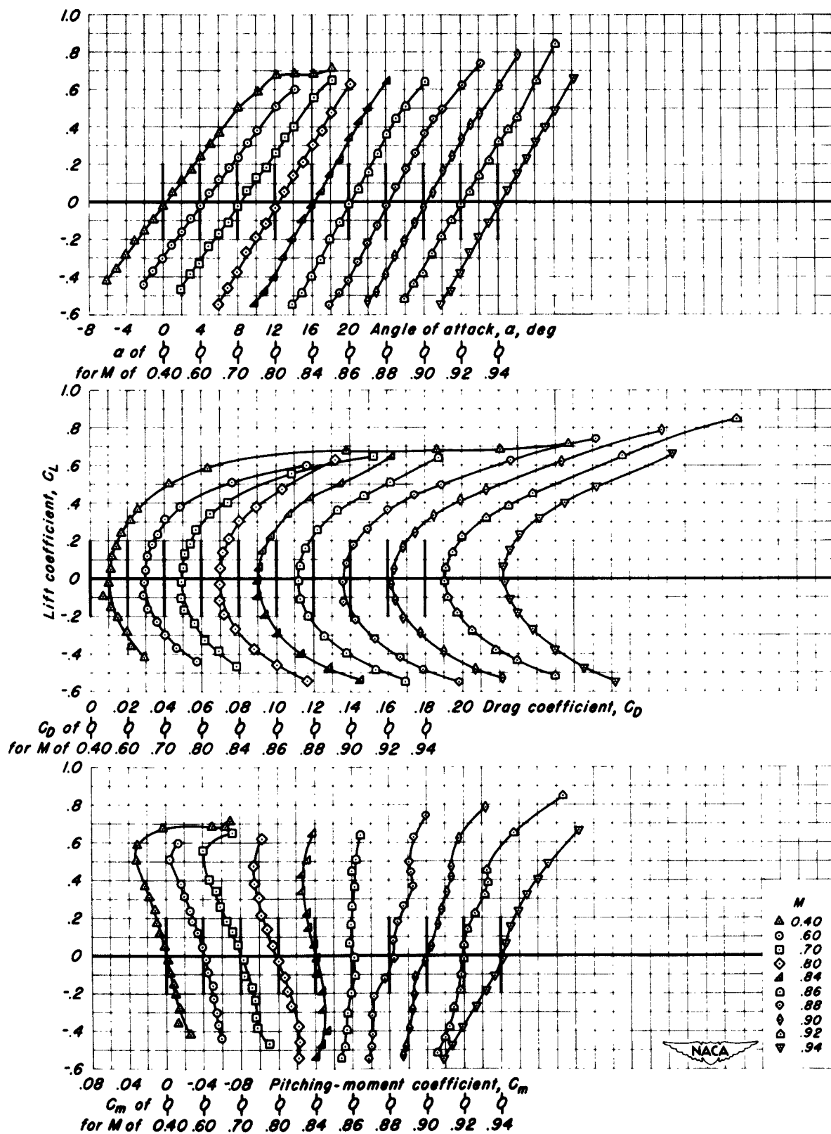
(c) Taper ratio 0.20. Figure 4.- Concluded.
