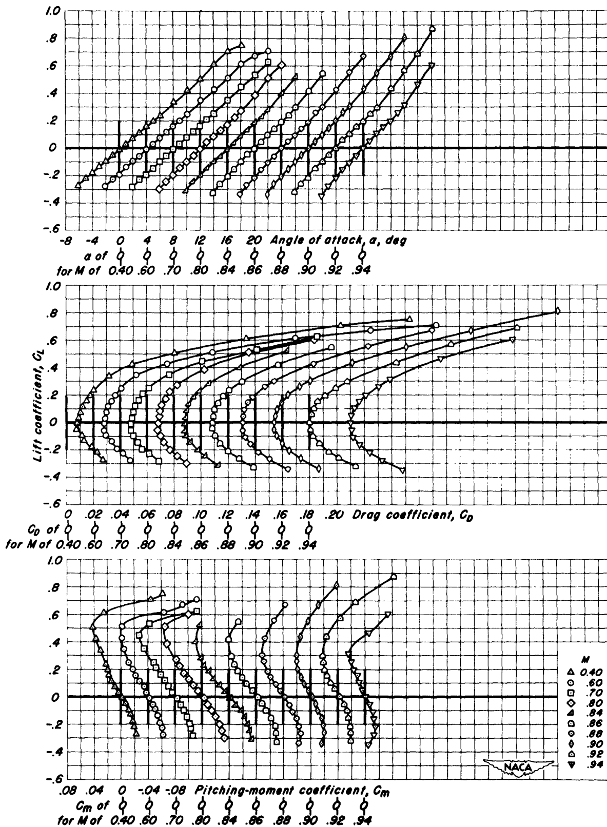
(c) Taper ratio 0.50. Figure 11.- Concluded.
