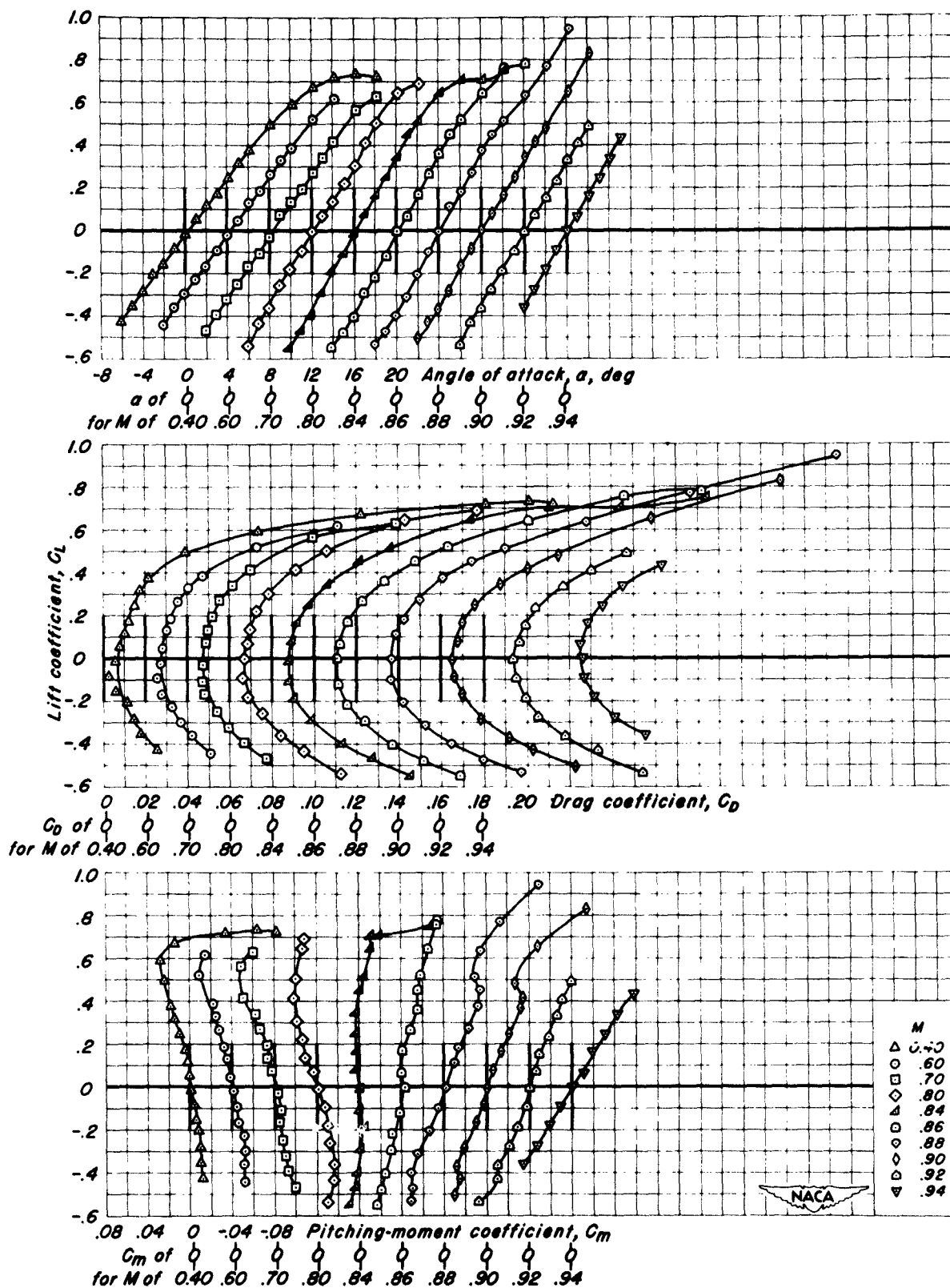
(c) Taper ratio 0.20. Figure 5.- Concluded.
