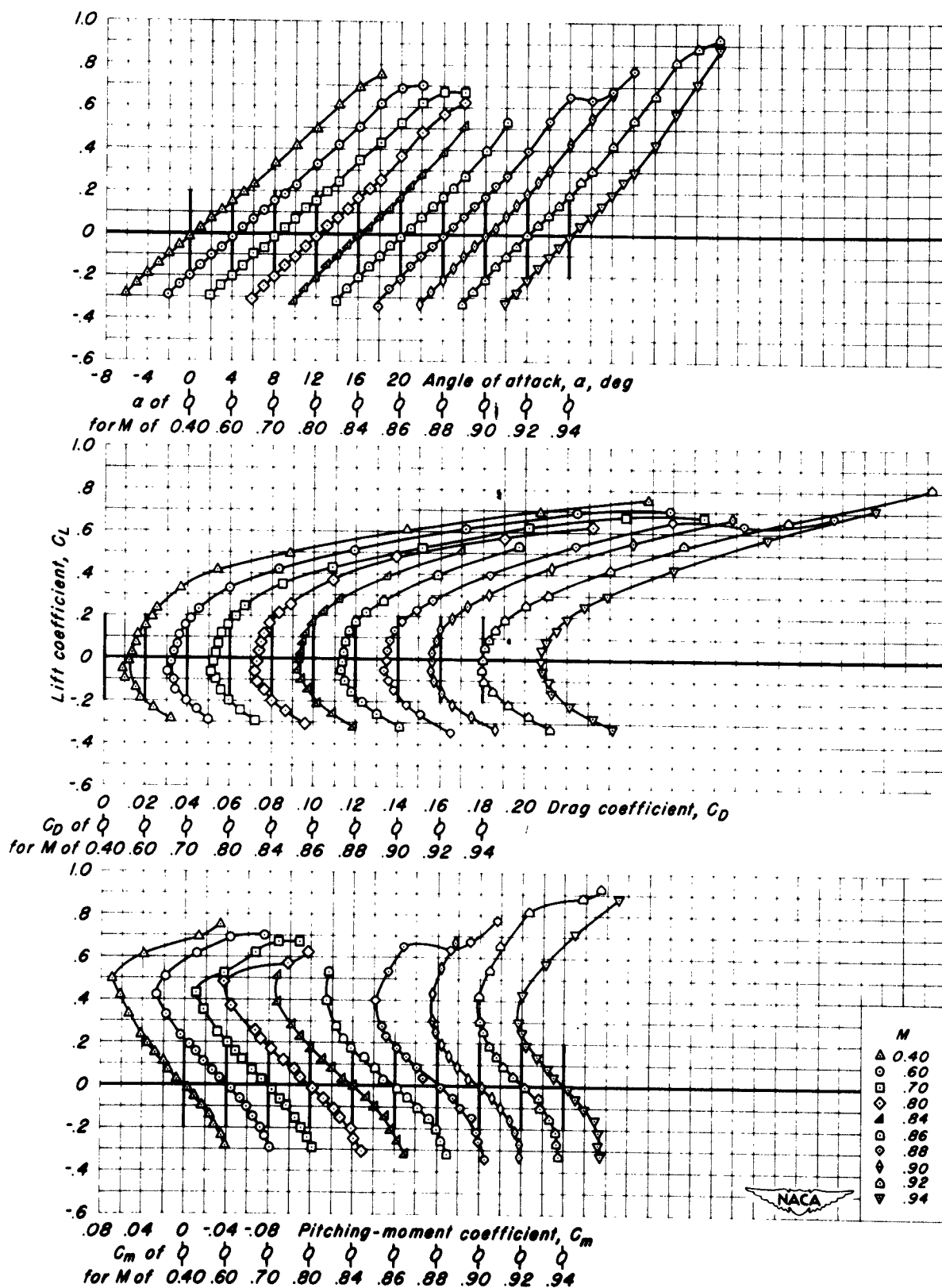
(b) Taper ratio 0.71. Figure 10.- Continued.
