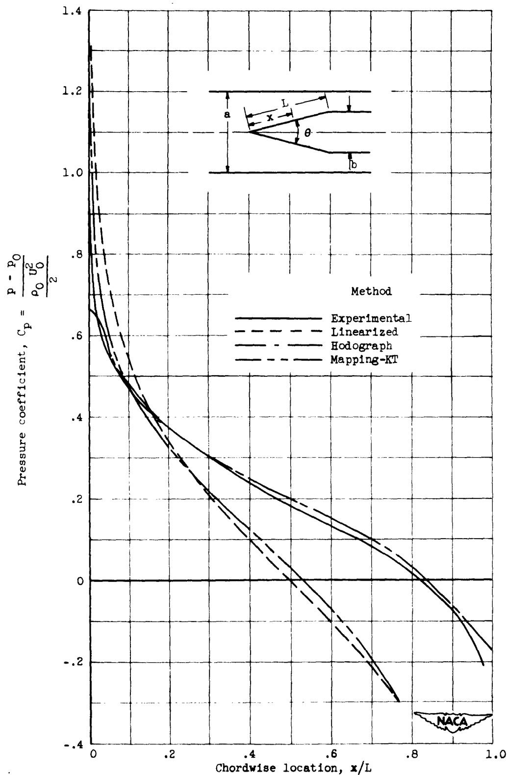
(c) Wedge angle, 20^\circ ; upstream Mach number, 0.892.
