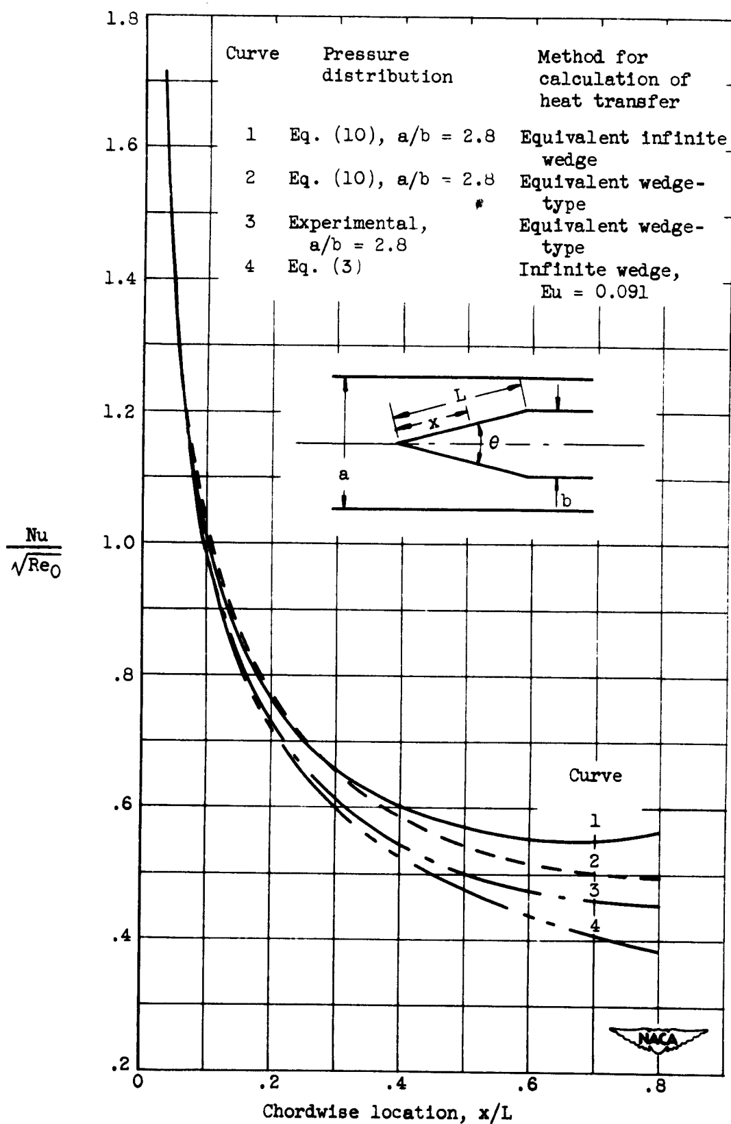
Figure 8. - Predicted heat transfer to 30^\circ wedge. Upstream Mach number, 0.
