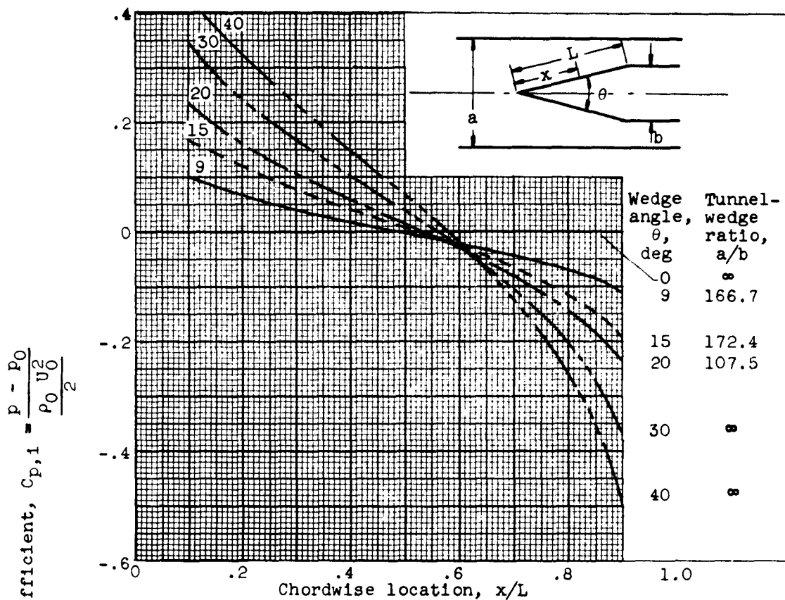
(a) Computed pressure coefficient against chordwise location.
