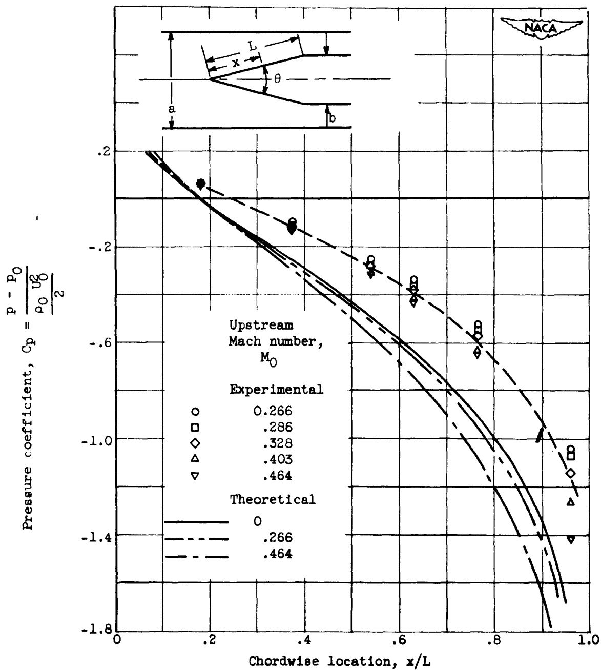
Figure 10. - Comparison of experimental and theoretical pressure coefficients for 30^\circ wedge with tunnel-wedge ratio of 2.8.
