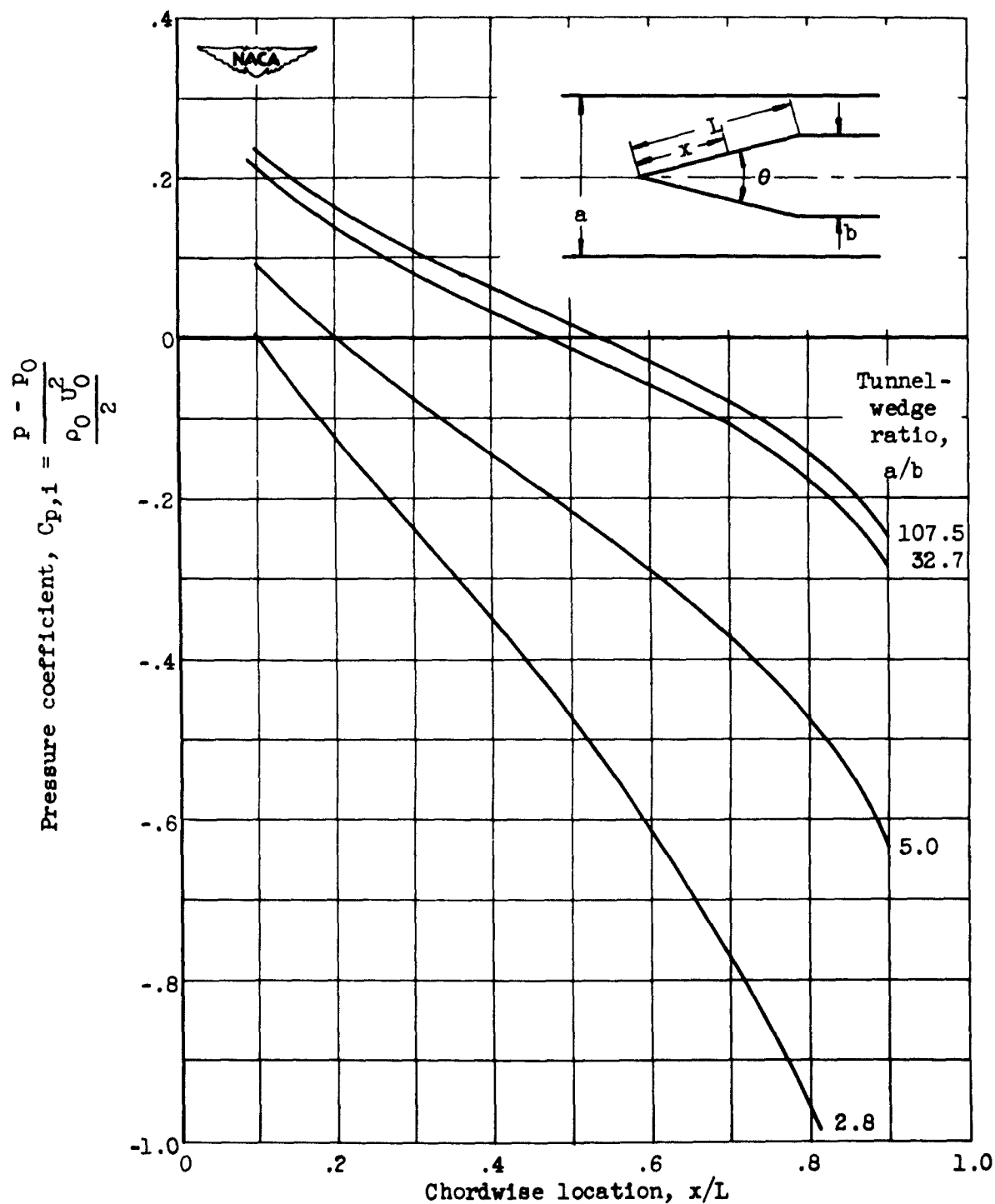
(a) Computed pressure coefficient against chordwise location.
