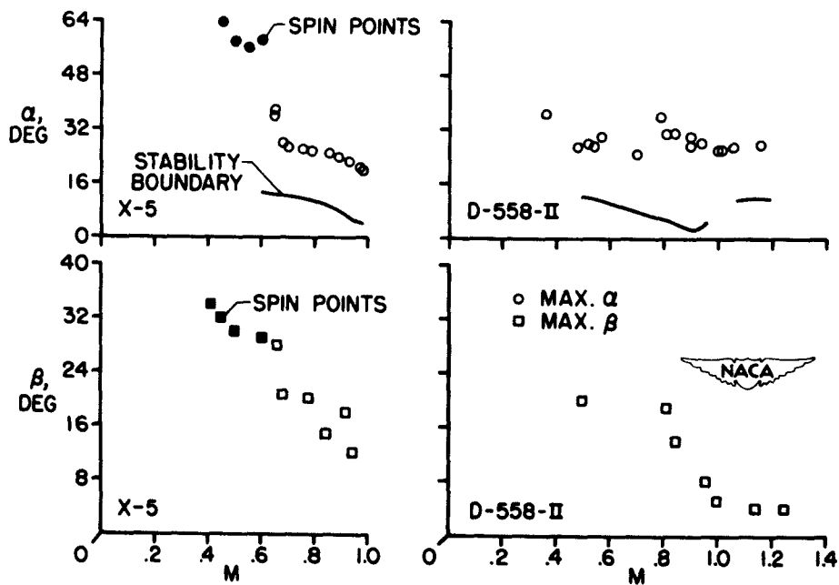
Figure 2.- Variations with Mach number of maximum angles of attack \alpha and sideslip \beta measured during inadvertent maneuvers.
