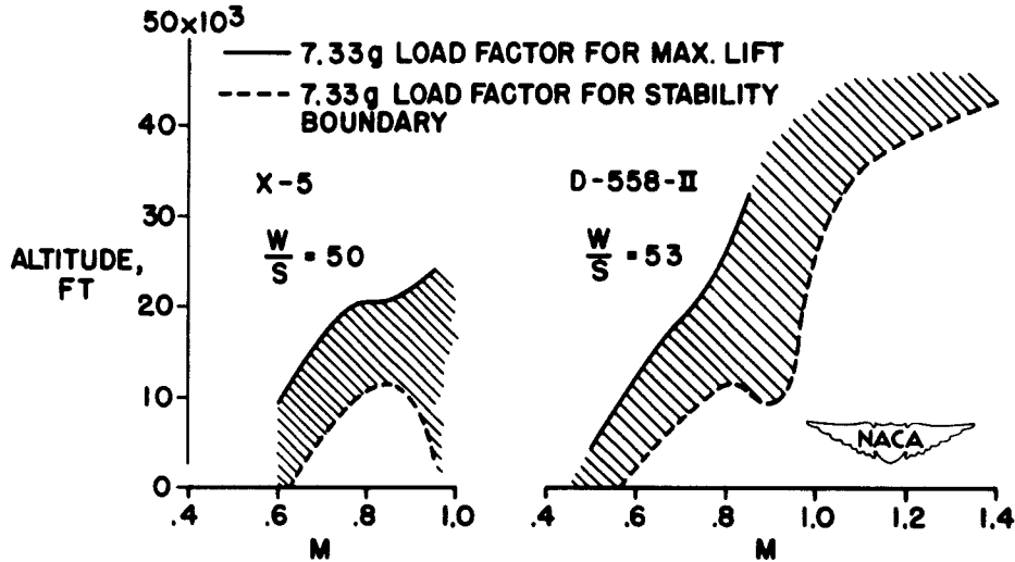
Figure 5.- Variation with Mach number of altitudes at which limit load factor may be inadvertently exceeded as a result of instability.
