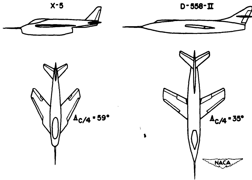
Figure 1.- General arrangements of X-5 and D-558-II research airplanes.
