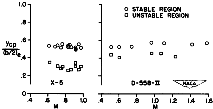
Figure 6.- Variation with Mach number of lateral center-of-pressure location, in terms of percentage of exposed-wing semispan, in the stable and unstable regions of flight.
