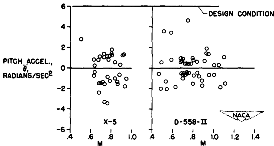
Figure 3.- Variation with Mach number of pitching acceleration \ddot{\theta} measured during pitch-up and recovery.
