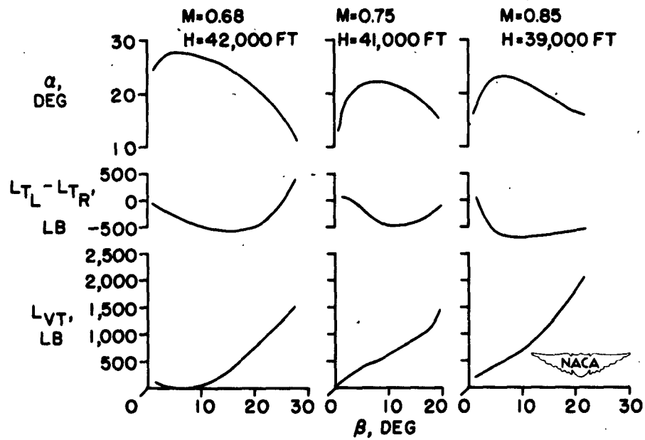
Figure 7.- Variations with angle of sideslip of angle of attack, unsymmetrical horizontal-tail load L_{TL} - L_{TR} , and aerodynamic vertical-tail load L_{VT} at high lift during directional divergences of the X-5 airplane.
