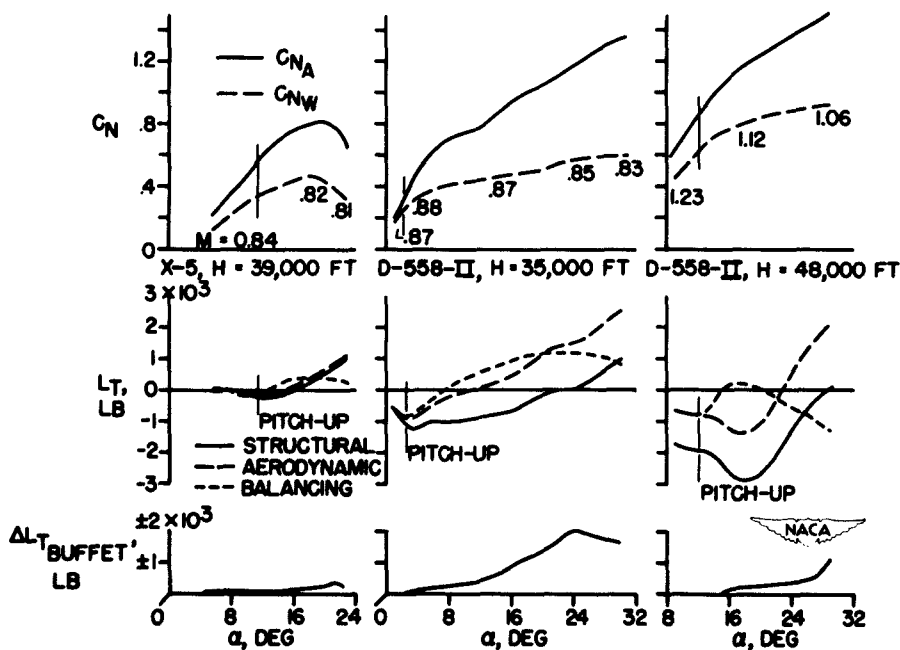
Figure 4.- Variations with angle of attack of airplane and wing normal-force coefficients C_{N_A} and C_{N_W} , horizontal-tail load L_T , and horizontal-tail buffet loads \Delta L_{T\_buffet} during pitch-ups experienced at subsonic and supersonic speeds.
