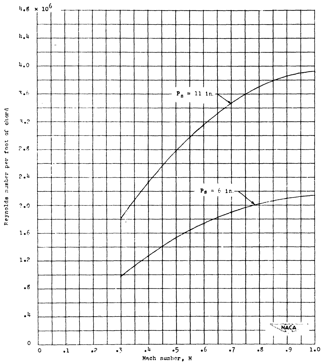
Figure 1.- Variation of Reynolds number per foot of chord with Mach number for various stagnation pressures P_s in inches of mercury and a stagnation temperature T_s of 70^\circ F.
