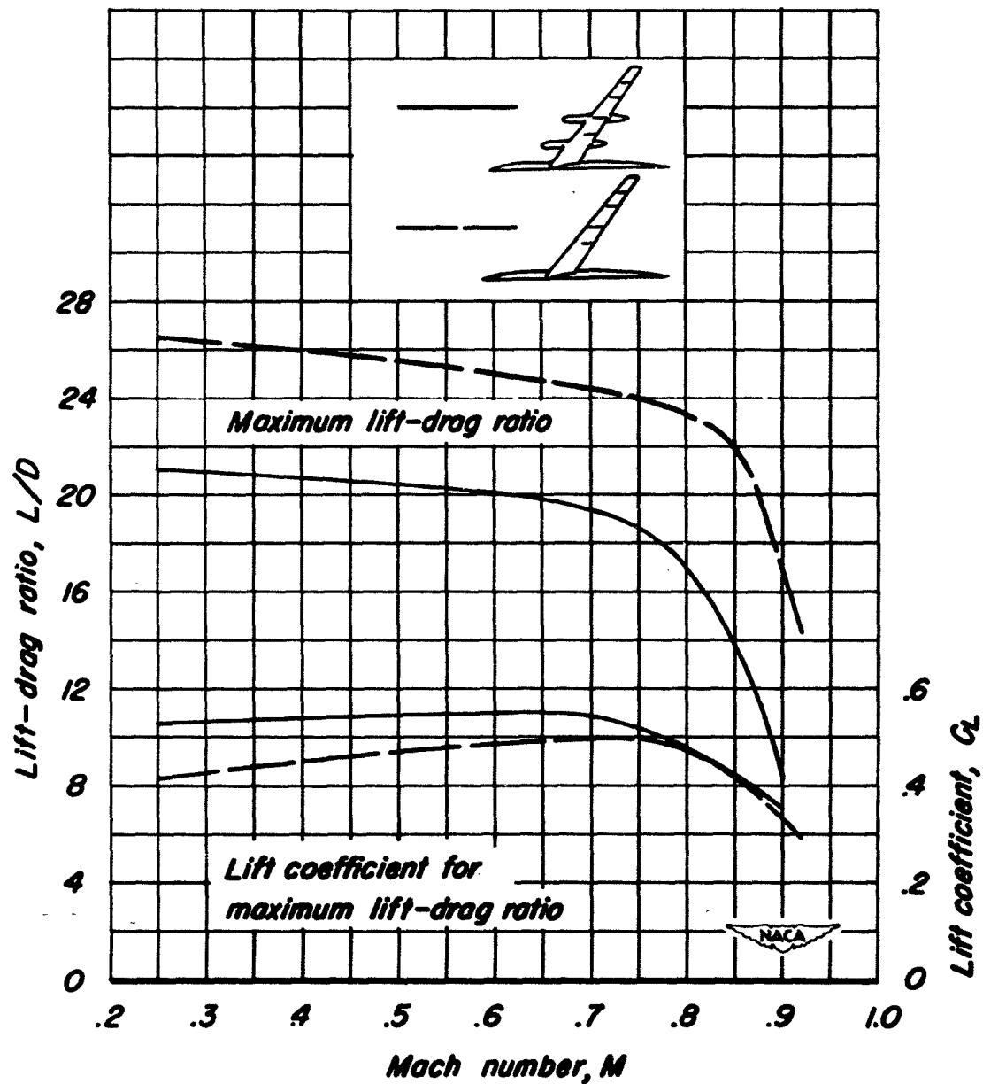
Figure 7.- The effect of nacelles on the variation of maximum lift-drag ratio and of lift coefficient for maximum lift-drag ratio with Mach number. R = 2,000,000 .
