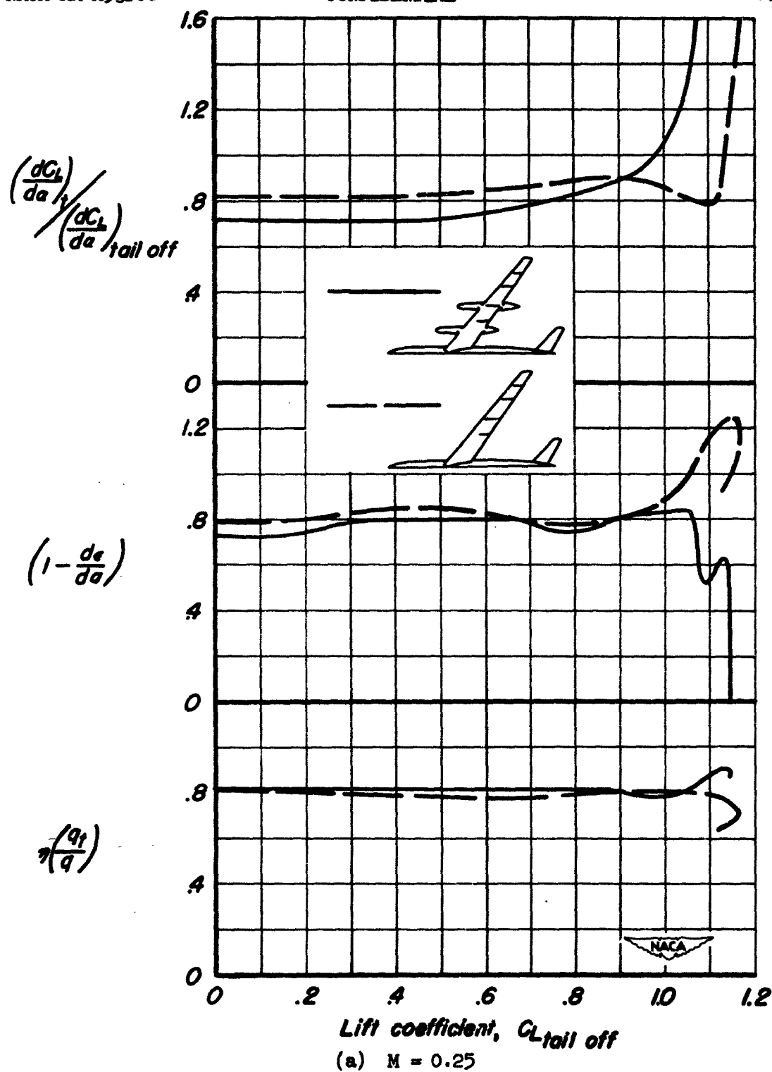
Figure 11.- The effect of the nacelles on the variation with lift coefficient of the factors affecting the stability contribution of the horizontal tail. R = 2,000,000 .
