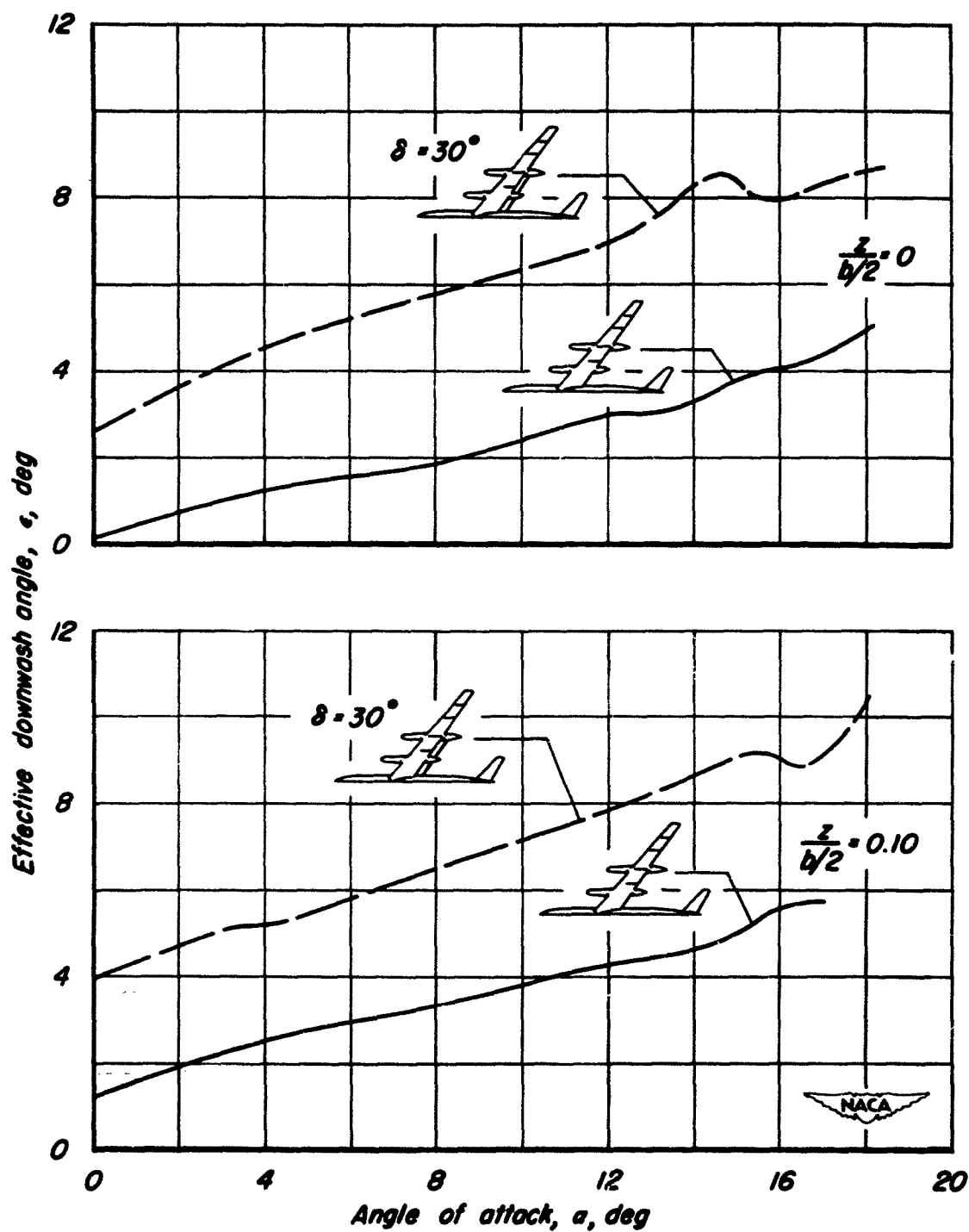
Figure 16.- The effect of the flaps on the effective downwash angle for two tail heights. M = 0.082 , R = 4,000,000 .
