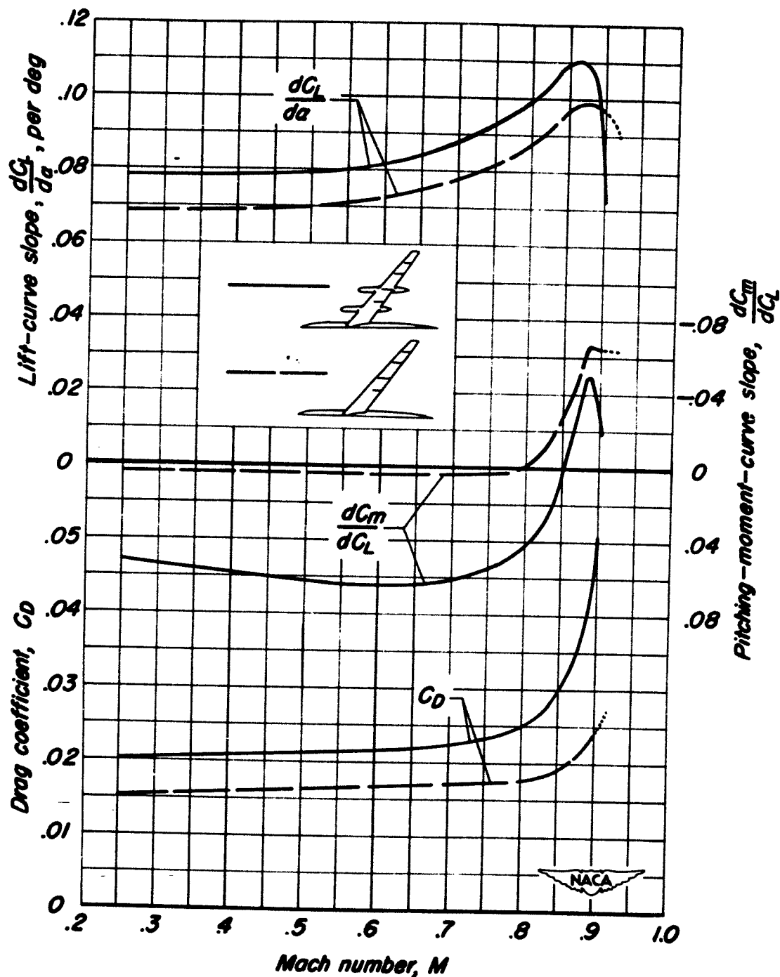
Figure 6.- The effect of the nacelles on the variation with Mach number of the lift-curve slope, the pitching-moment-curve slope, and the drag coefficient. C_L = 0.4 , R = 2,000,000 .
