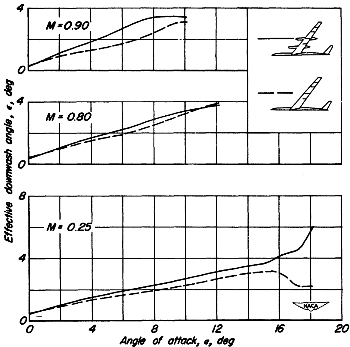
Figure 10.- The effect of the nacelles on the effective downwash angle.
