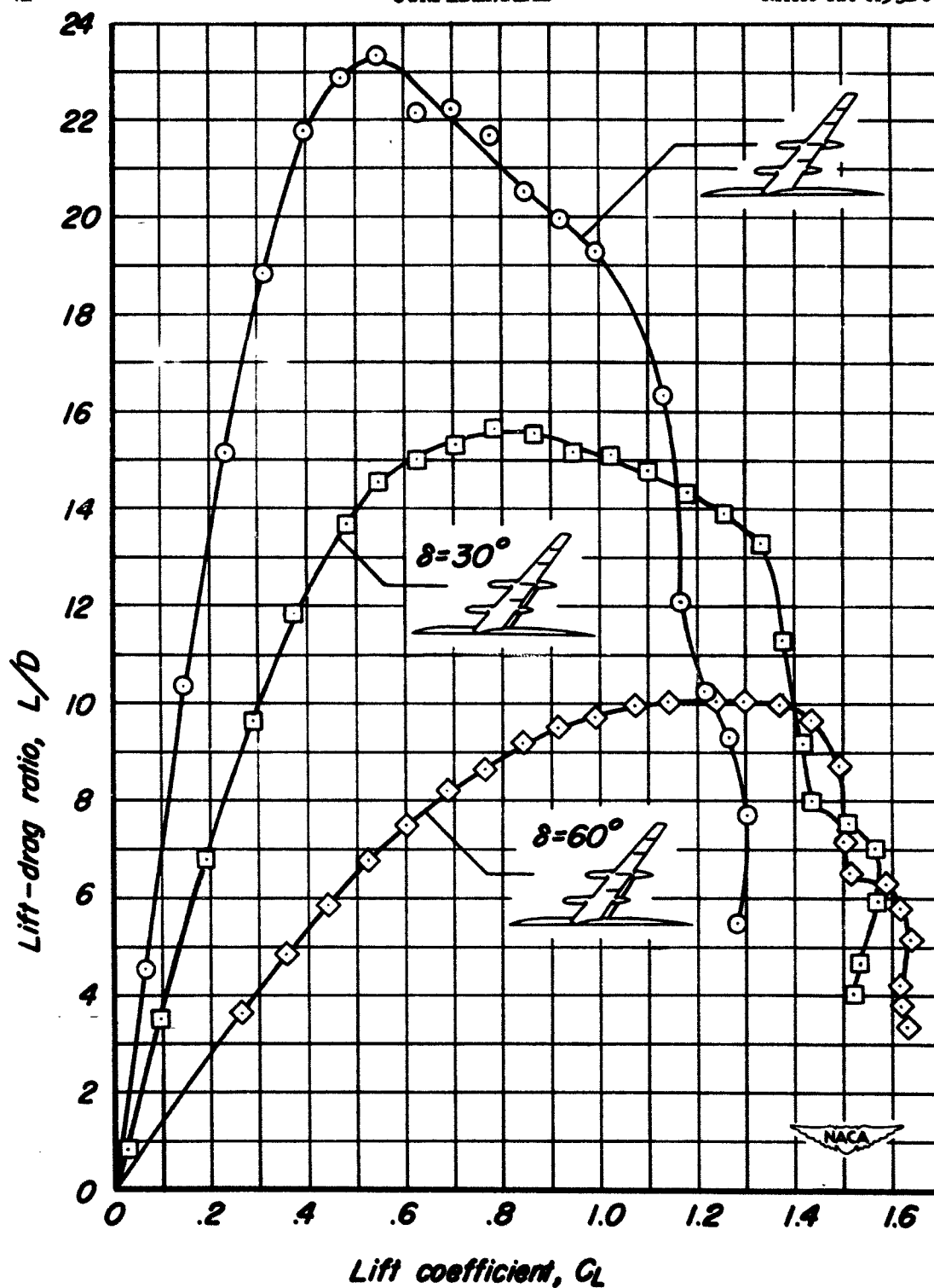
Figure 13.- The effect of flaps on the lift-drag ratio. M = 0.082 , R = 4,000,000 .
