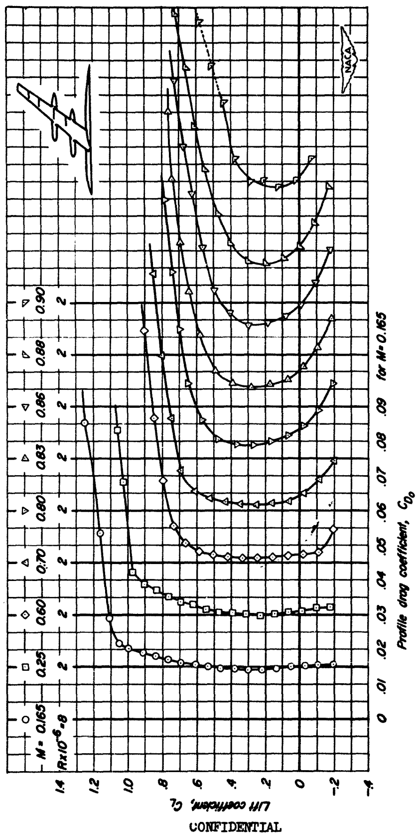
(c) C_{D0} vs C_L Figure 3.- Concluded.
