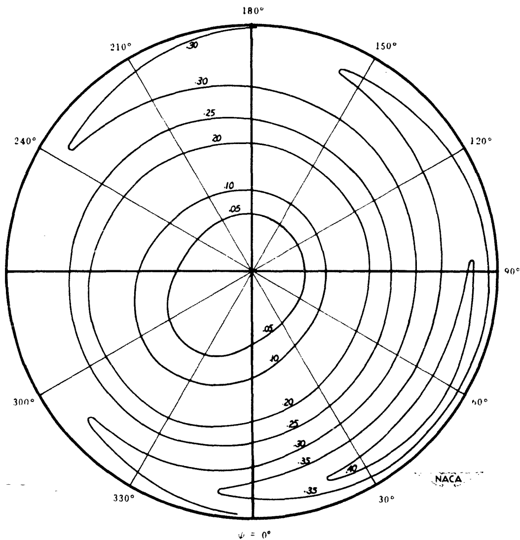
Figure 34.- Curves of constant aerodynamic loading in pounds per inch. Profile, NACA 0015; speed, 800 rpm; \xi = 0 ; \mu = 0.50 ; \theta = 8^\circ ; \alpha = -5^\circ ; C_T/\sigma = 0.076 .
