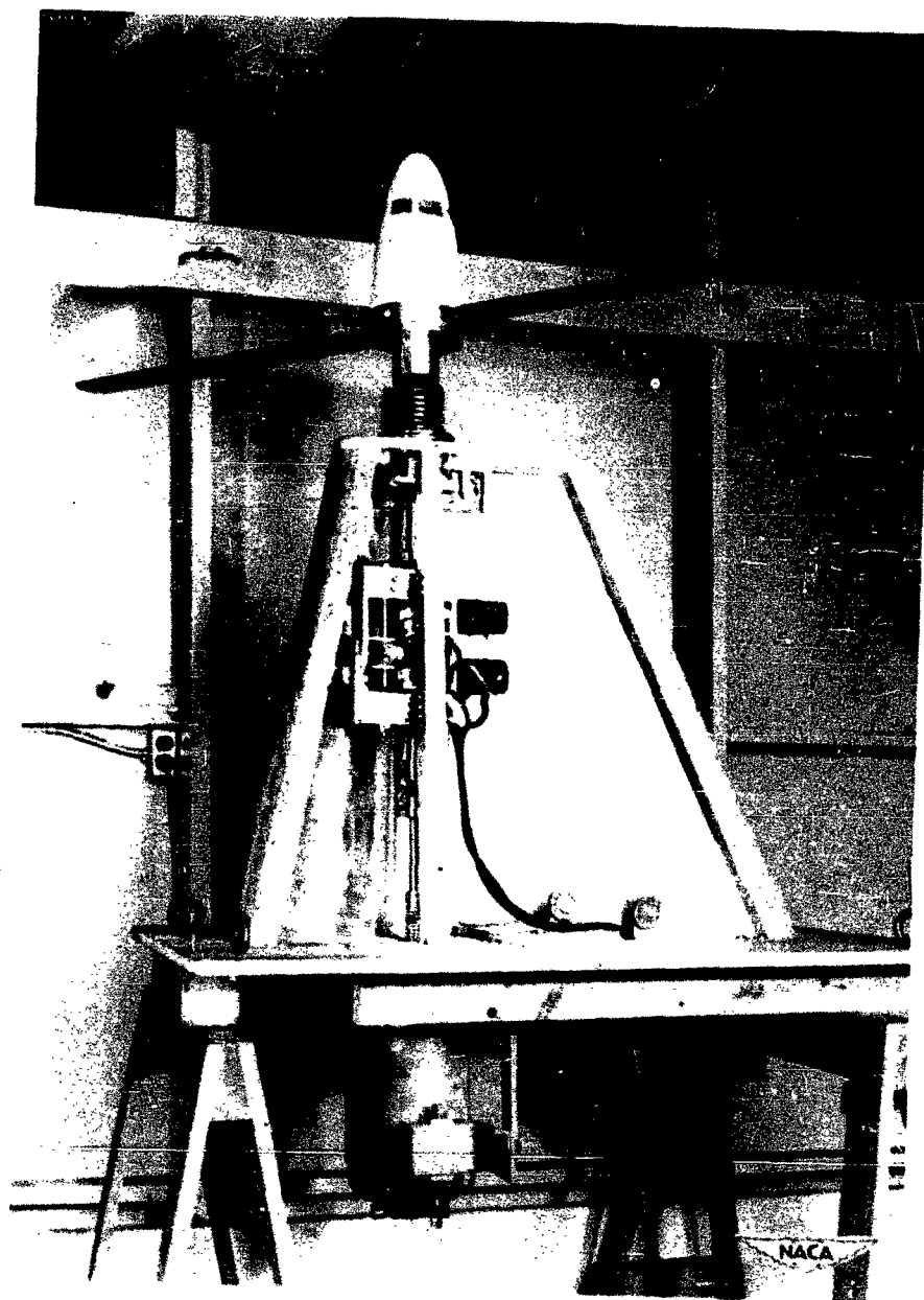
Figure 9.- Wind-tunnel mount.
