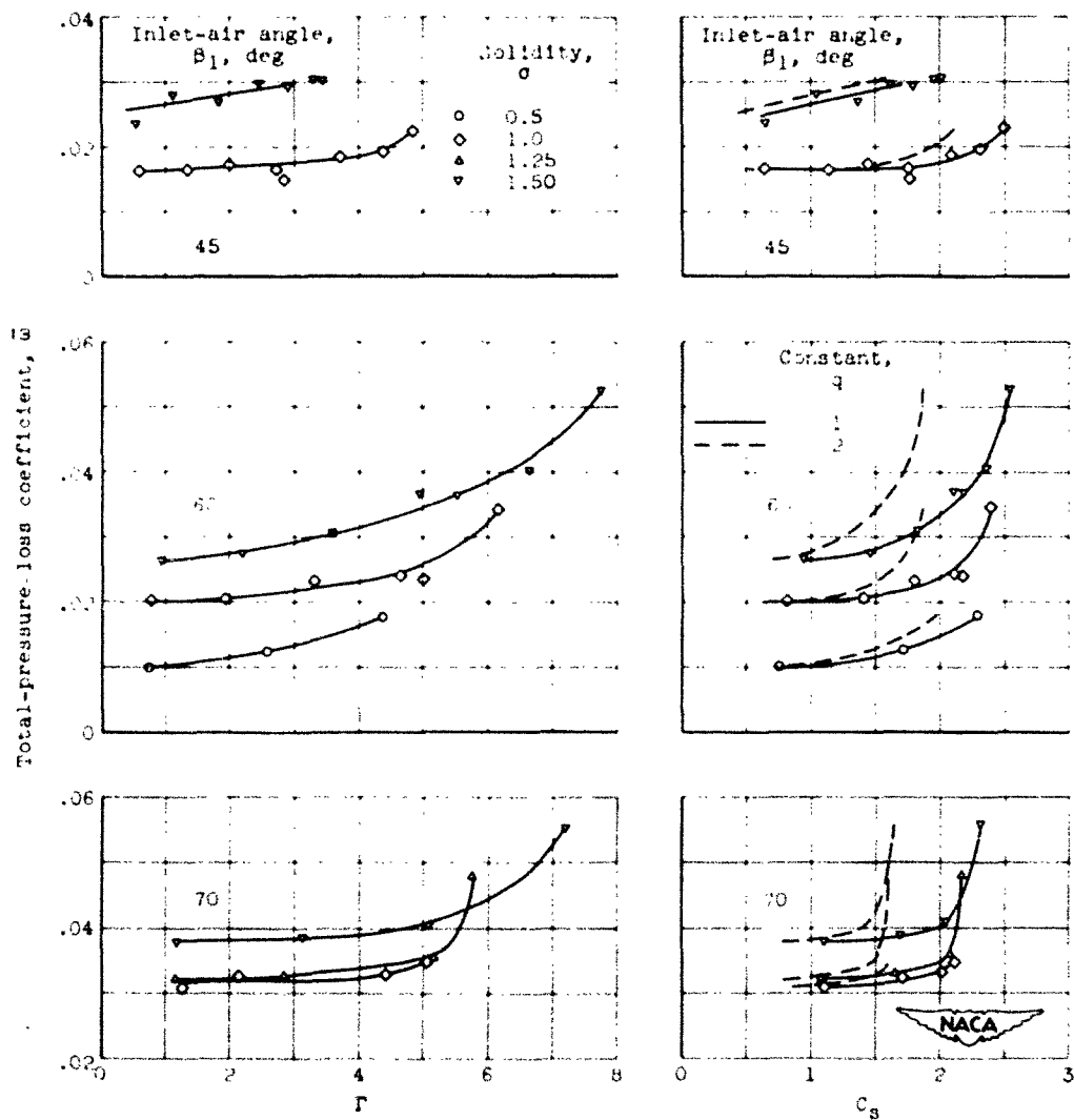
Figure 3. - Continued. Variation of total-pressure loss coefficient at design angle of attack with various blade-loading parameters for NACA 65-series blade sections in two-dimensional low-speed cascade.
