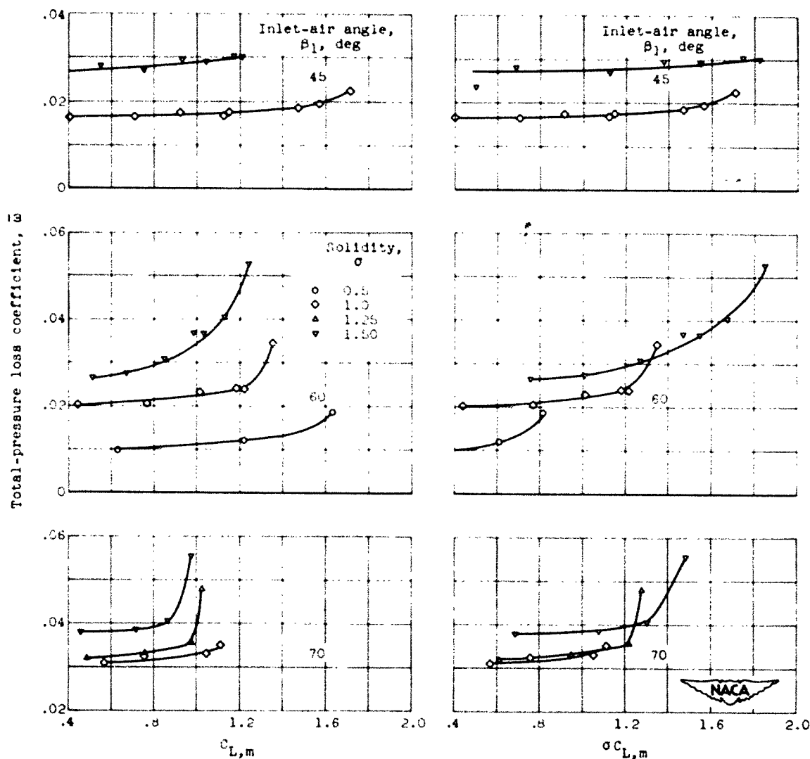
(a) Lift coefficient based on vector-mean velocity.
