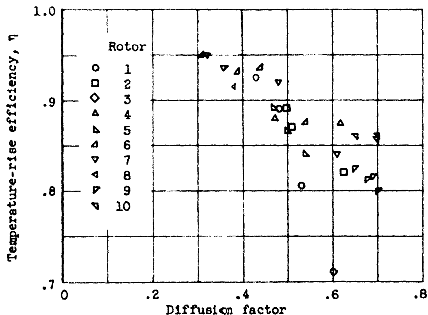
Figure 9. - Variation of maximum blade-element temperature-rise efficiency with diffusion factor in tip region of axial-flow single-stage rotors.
