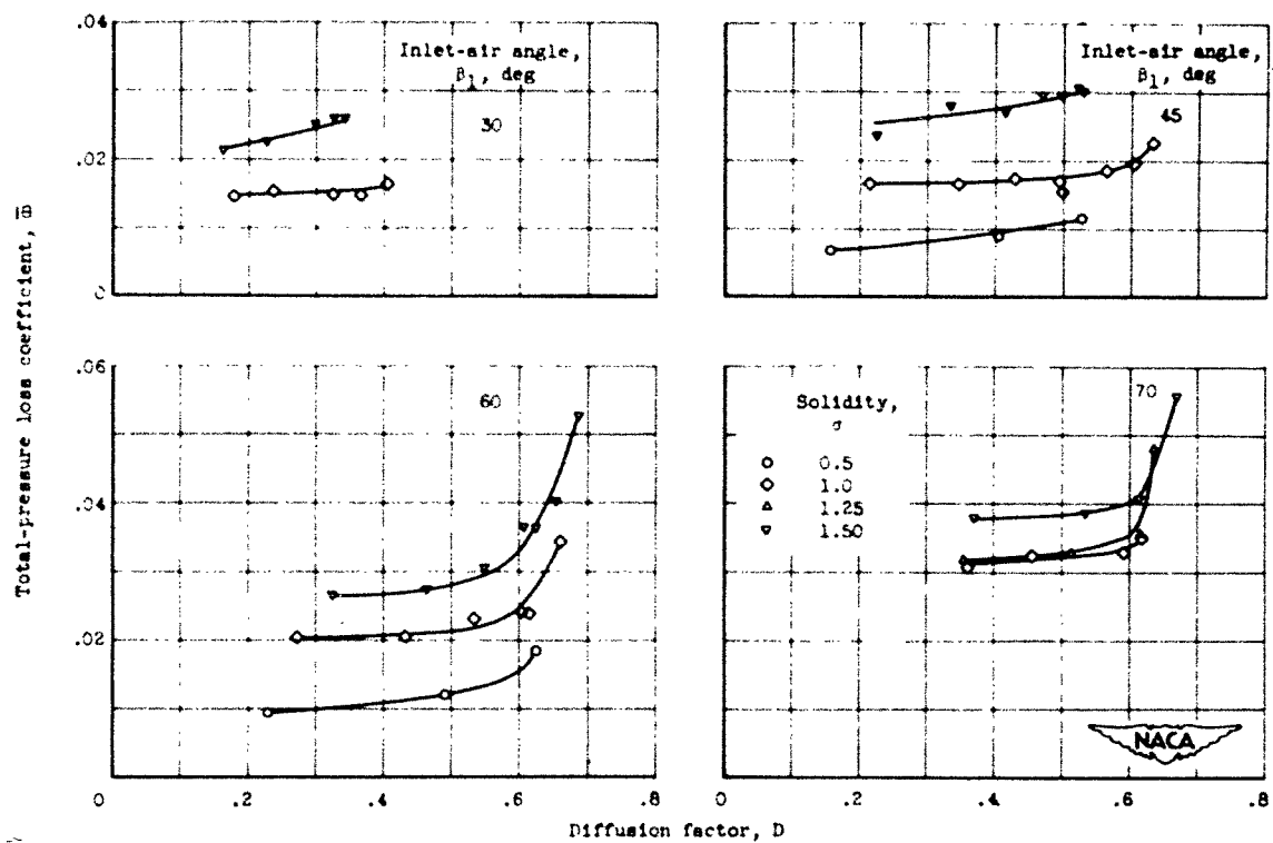
Figure 3. - Concluded. Variation of total-pressure-loss coefficient at design angle of attack with various blade-loading parameters for NACA 65-series blade sections in two-dimensional low-speed cascade.
