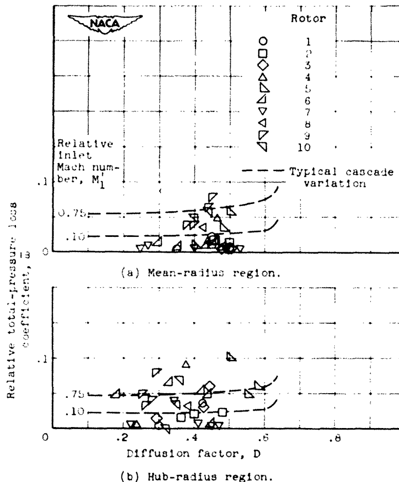
Figure 6. - Variation of minimum (design) blade-element relative total-pressure loss coefficient with diffusion factor for axial-flow single-stage rotors.
