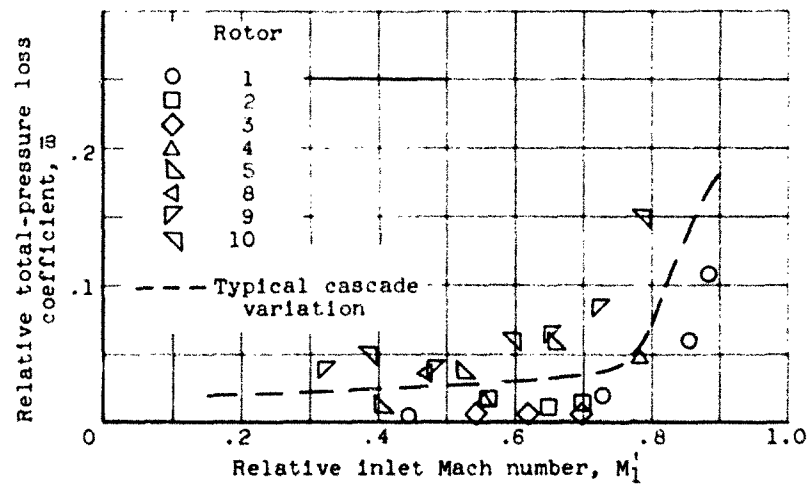
Figure 7. - Variation of minimum (design) blade-element relative total-pressure loss coefficient with relative inlet Mach number at mean radius for 65-series rotor blades.
