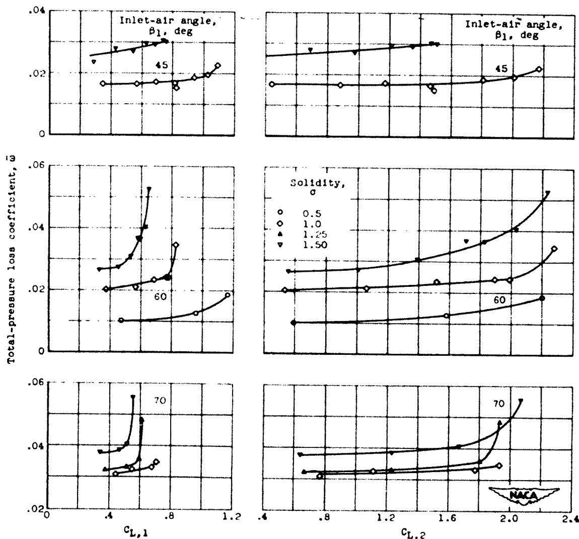
(c) Lift coefficient based on inlet velocity.
