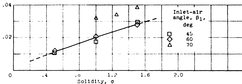
(a) Solidity for diffusion factor of 0.5 (fig. 3(t)).
