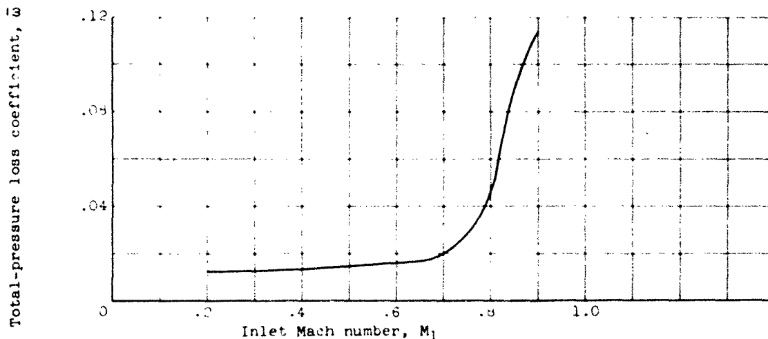
(b) Inlet Mach number for NACA 65-(12)10 blade. Solidity, 1.0; inlet-air angle, 45^\circ (ref. 11).
