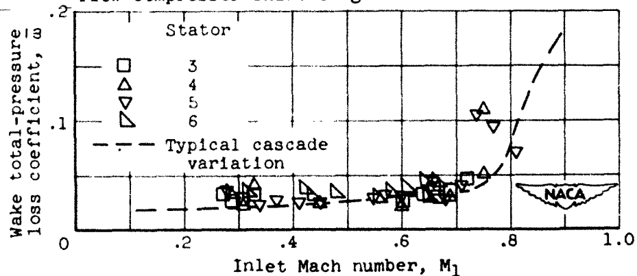
Figure 13. - Variation of minimum wake total-pressure loss coefficient with inlet Mach number at hub, mean, and tip regions of stators with 65-series profiles.
