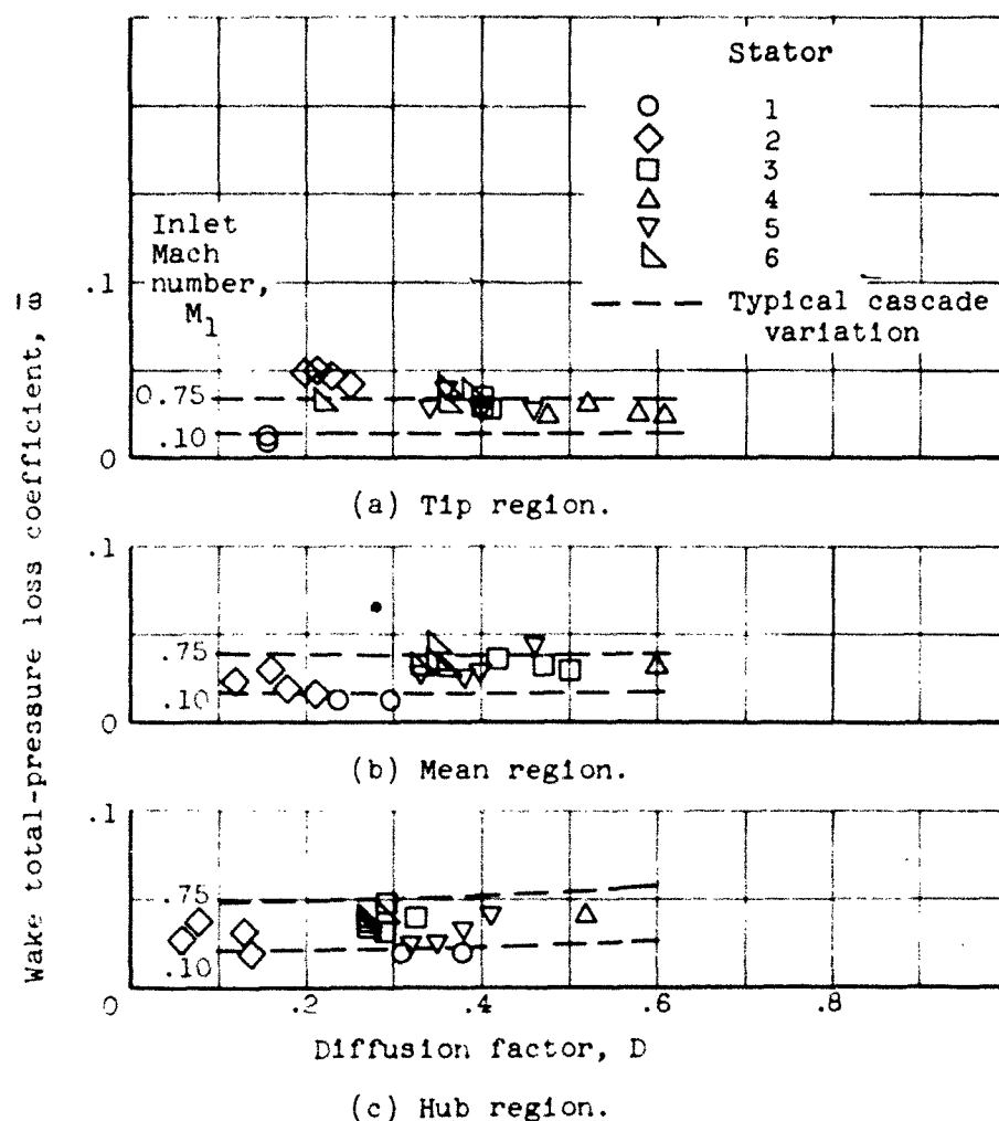
Figure 12. - Variation of minimum wake total-pressure loss coefficient with diffusion factor for axial-flow compressor inlet-stage stators.
