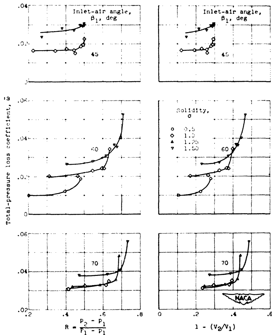
Figure 3. - Continued. Variation of total-pressure loss coefficient at design angle of attack with various blade-loading parameters for NACA 65-series blade sections in two-dimensional low-speed cascade.
