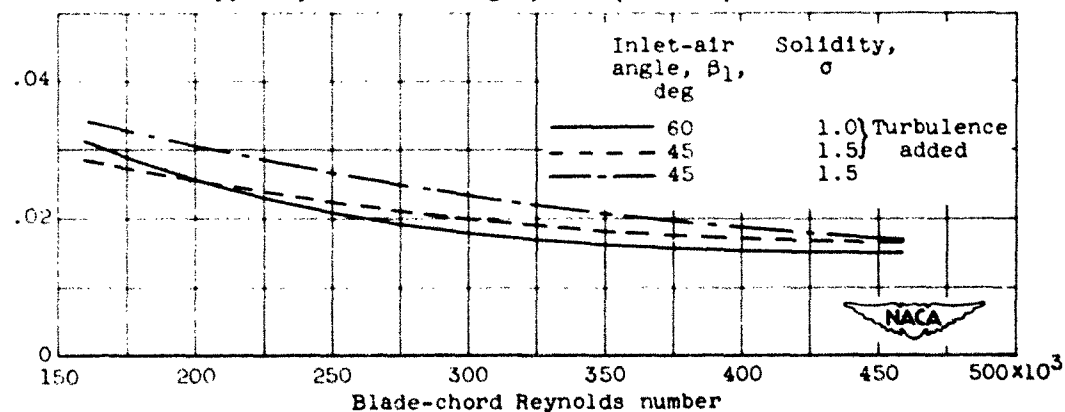
(c) Reynolds number for 65-(12)10 blade (ref. 3).
