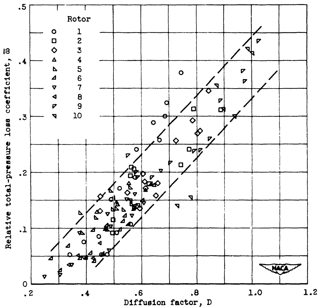
Figure 10. - Variation of blade-element relative total-pressure loss coefficient with diffusion factor in tip region of axial-flow single-stage rotors. All data points in positive incidence range from region of minimum loss to region of drop in efficiency of about 0.10.
