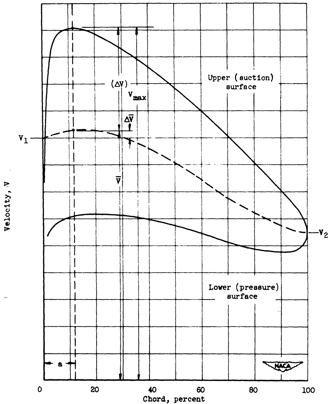
Figure 1. - Typical distribution of velocity along surfaces of compressor-cascade blade section in range of design angle of attack.
