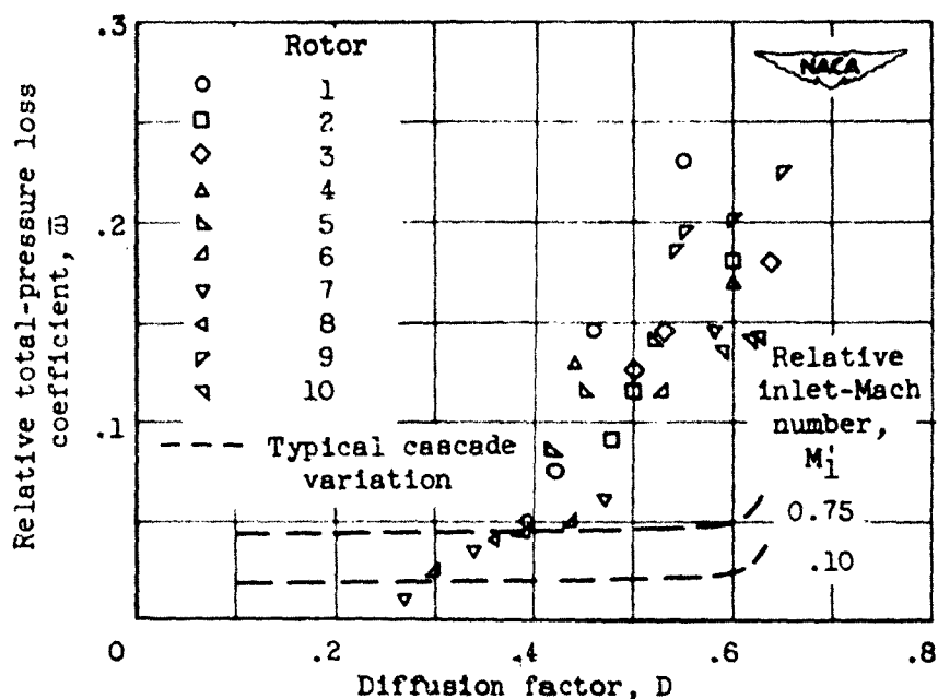
Figure 8. - Variation of minimum (design) blade-element relative total-pressure loss coefficient with diffusion factor in tip region of axial-flow single-stage rotors.
