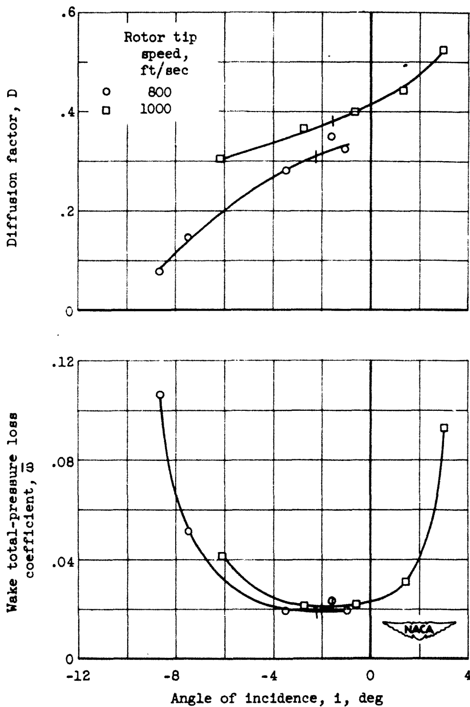
Figure 11. - Example of variation of wake total-pressure loss coefficient and diffusion factor with angle of incidence in hub region of stator (stator 1). Bars indicate points of minimum loss.
