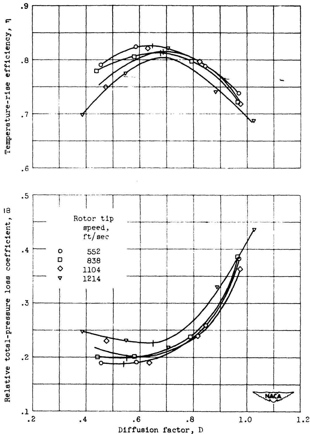
Figure 5. - Example of variation of blade-element temperature-rise efficiency and relative total-pressure loss coefficient with diffusion factor in tip region of rotor (rotor 9). Bars indicate minimum or maximum values.
