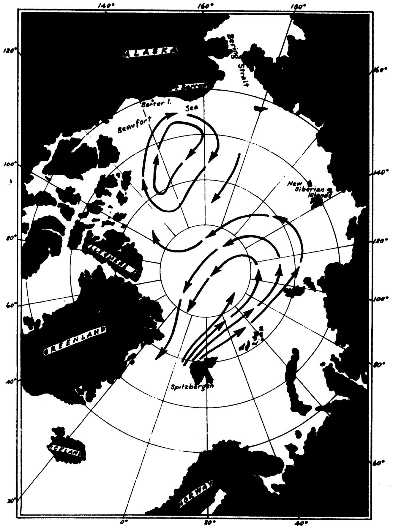
Fig. 12 Subsurface circulation in the North Polar Basin.
