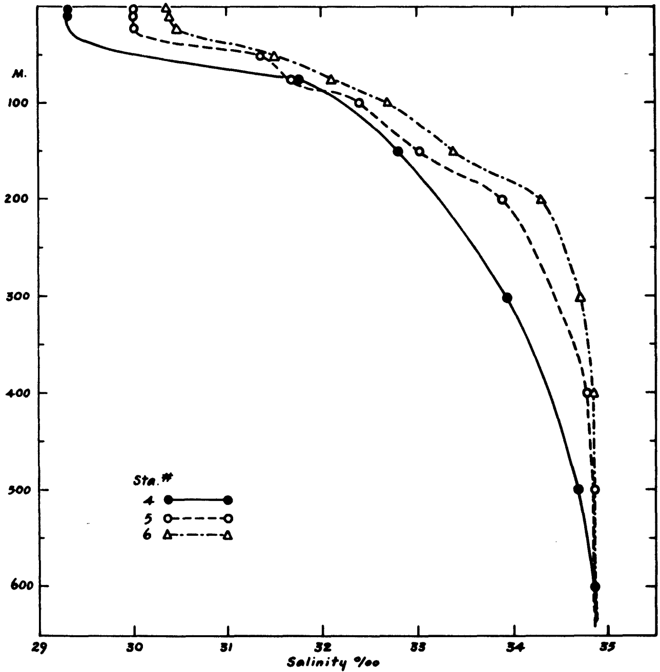
Fig. 13 Salinity-depth curves for SKIJUMP stations.
