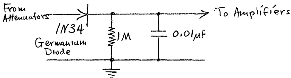
Fig. 2 Integrating circuit
