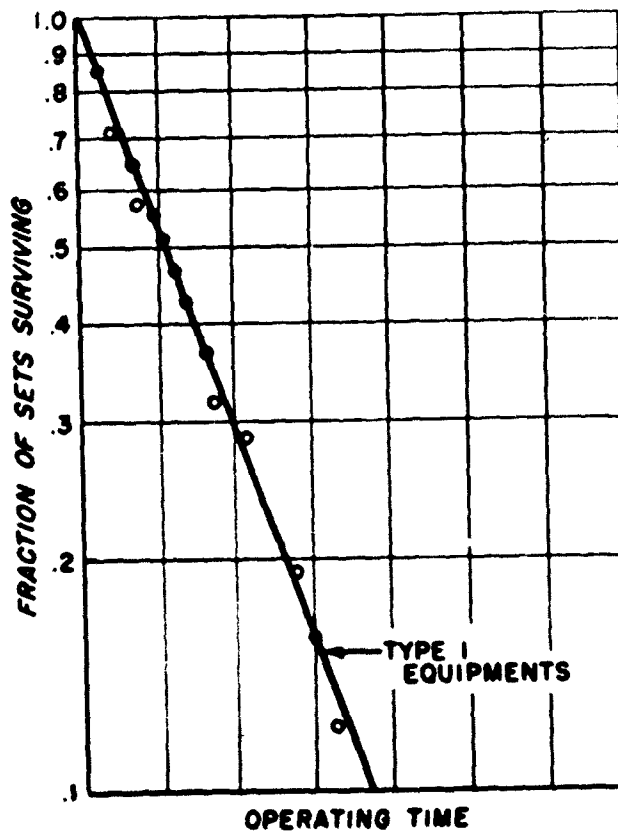
Fig. 7—Failure in Type 1 Airborne Radar Equipments
