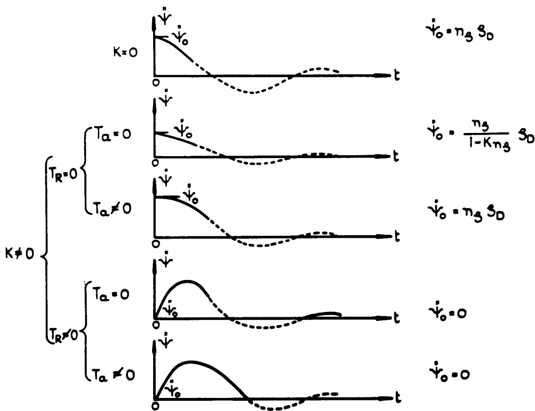
(b) ANGULAR ACCELERATION RESPONSES TO A STEP IN CONTROL SURFACE DEMAND s_d .
