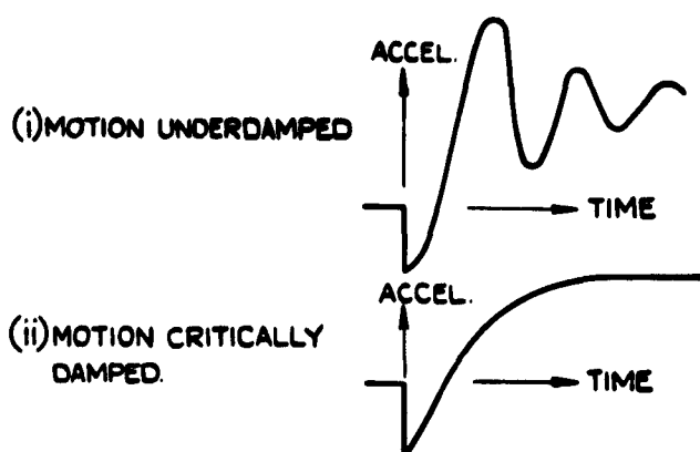
(a) THE FORM OF THE ACCELERATION RESPONSE OF THE MISSILE TO A STEP MOTION OF THE CONTROL SURFACE SHOWING THE REVERSE KICK.
