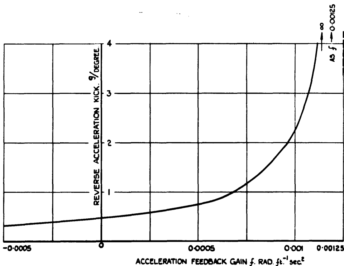
(b) THE REVERSE ACCELERATION KICK AS A FUNCTION OF THE ACCELERATION FEEDBACK GAIN.
