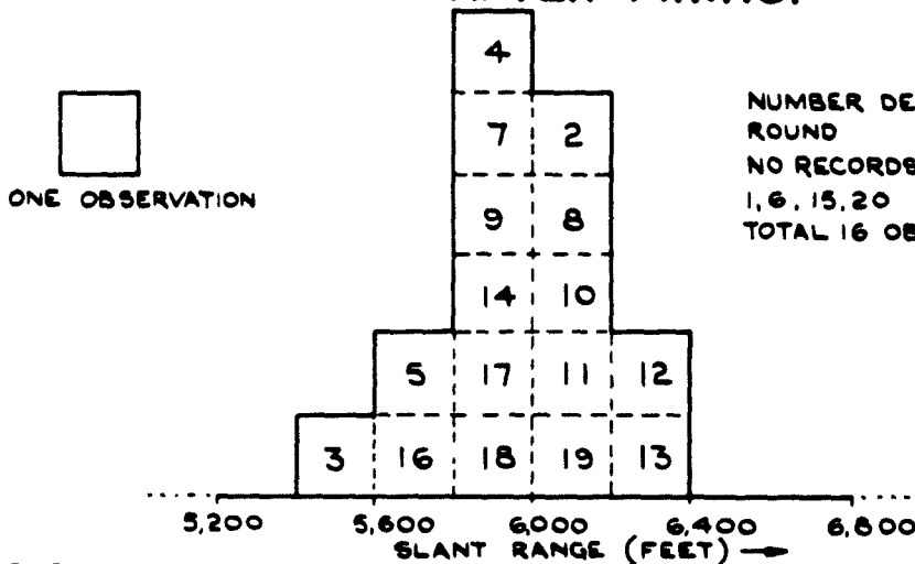
FIG. 23 SLANT RANGE OF ROUND 5 SECONDS AFTER FIRING.
