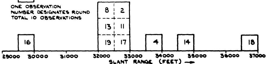
FIG. 39 SLANT RANGE OF MISSILE 25 SECONDS AFTER FIRING.
