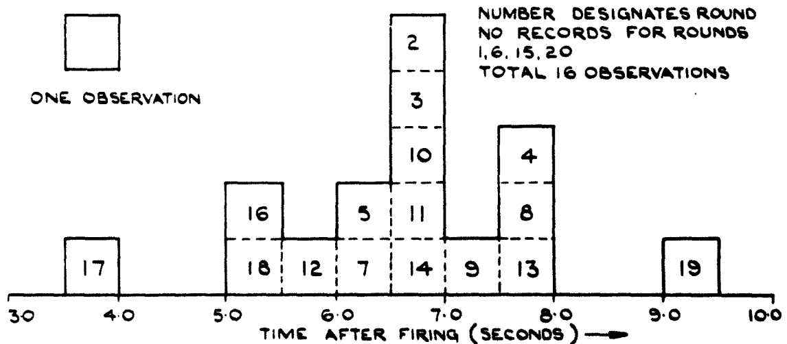
FIG.30 TIME WHEN GUIDANCE BEAM STEADIES.
