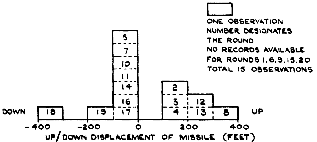
MEASURED FROM LINE ELEVATION 19 DEGREES, BEARING 355 DEGREES FIG.14 U/D DISPLACEMENT OF MISSILE 6 SECS AFTER FIRING.
