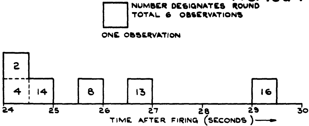
FIG. 43 TIME AFTER FIRING WHEN MOTOR THRUST CEASES.
