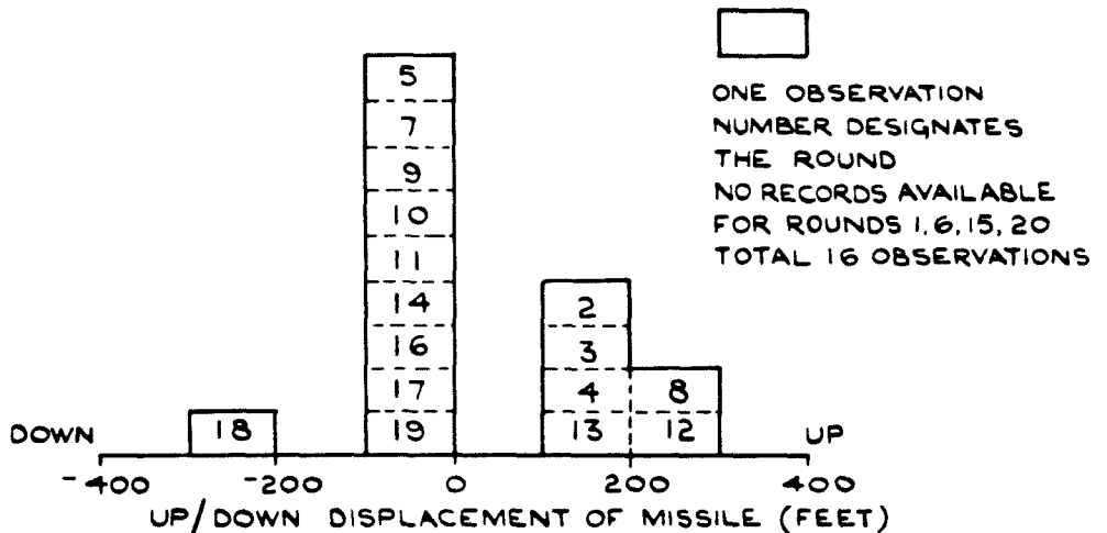
MEASURED FROM LINE ELEVATION 19 DEGREES, BEARING 355 DEGREES FIG.13 U/D DISPLACEMENT OF MISSILE 5 SECS AFTER FIRING.
