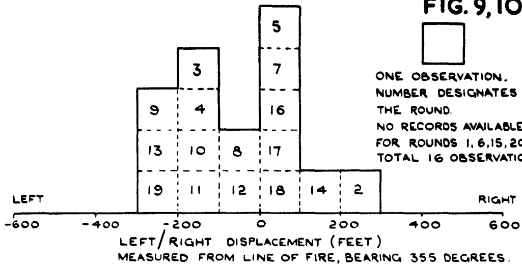
FIG. 9 L/R DISPLACEMENT OF MISSILE 4 SECS AFTER FIRING.
