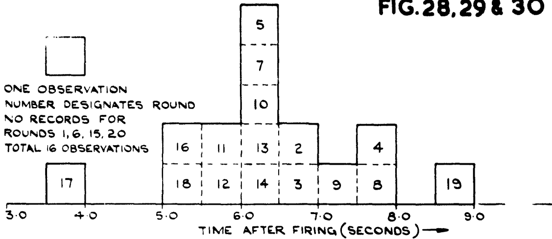
FIG.28 TIME WHEN ELEVATION OF GUIDANCE BEAM STEADIES.
