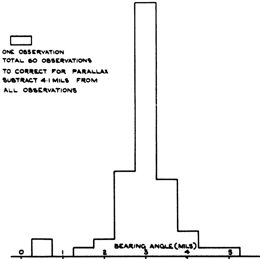
FIG. 46 BEARING OF BEAM RIDING DIRECTION RELATIVE TO THE AXIS OF THE FIXED REFERENCE TELESCOPE.
