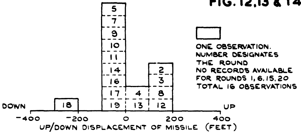
MEASURED FROM LINE ELEVATION 19 DEGREES, BEARING 355 DEGREES. FIG.12 U/D DISPLACEMENT OF MISSILE 4 SECS AFTER FIRING.
