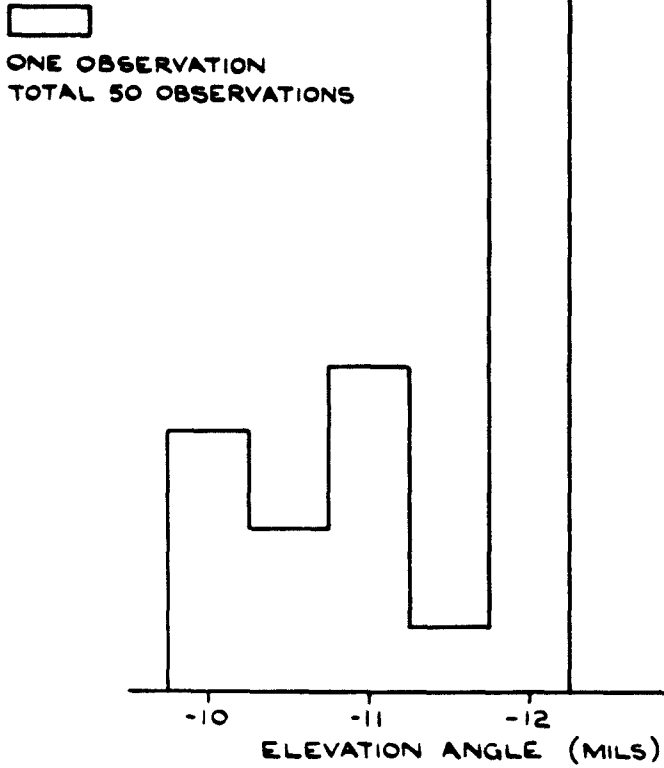
FIG.47 ELEVATION OF MOVABLE REFERENCE TELESCOPE RELATIVE TO FIXED REFERENCE TELESCOPE.
