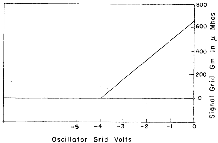
FIGURE 5 IDEALIZED CHARACTERISTIC CURVES FOR LINEAR CONVERTER OPERATION
