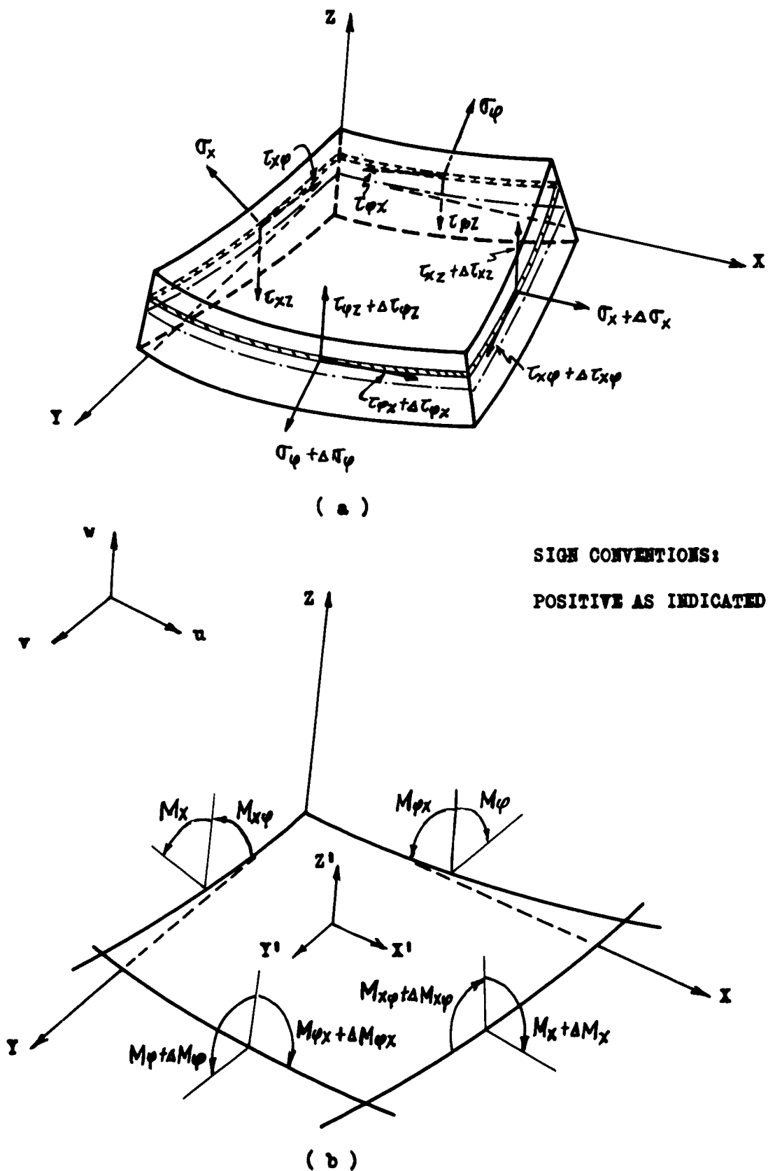
SHELL ELEMENT
