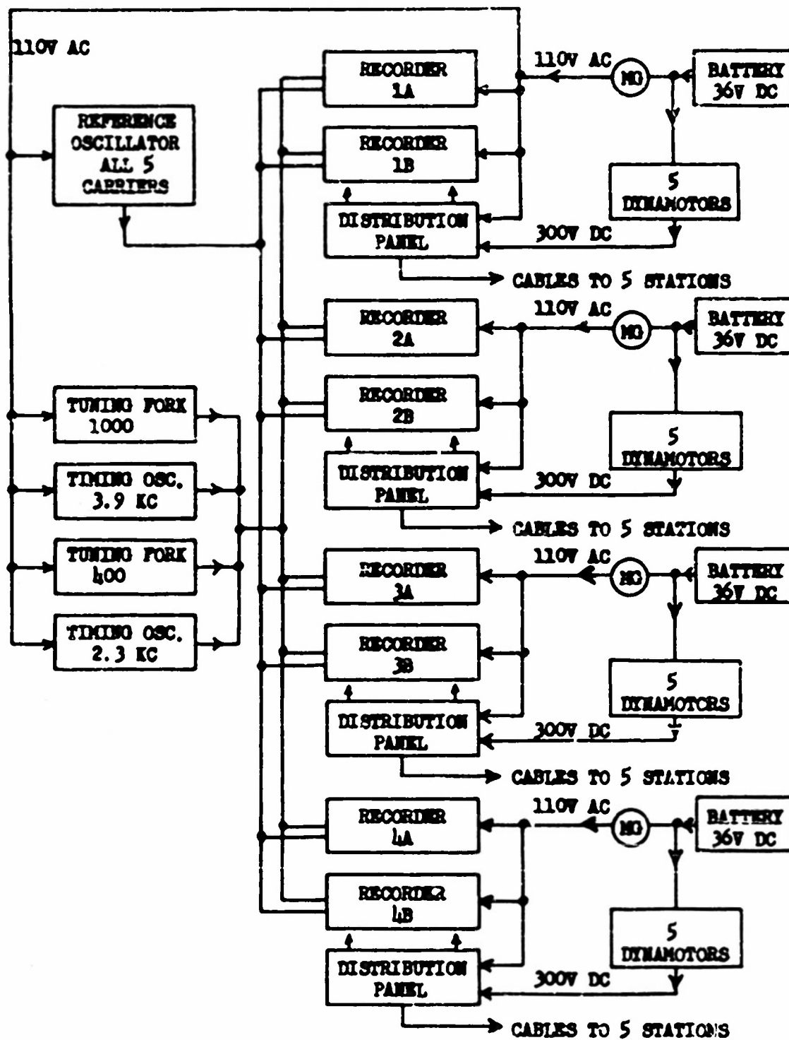
FIG. 5.4 OVER-ALL RECORDING SYSTEM
