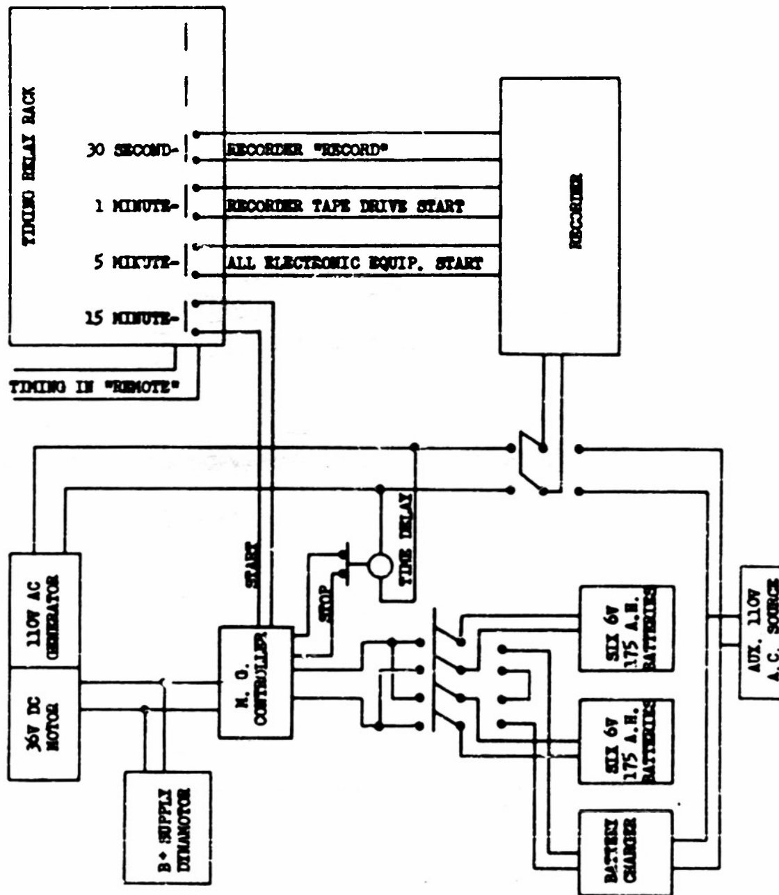
FIG. 5.27 POWER CONTROLS FOR TYPICAL BANK
