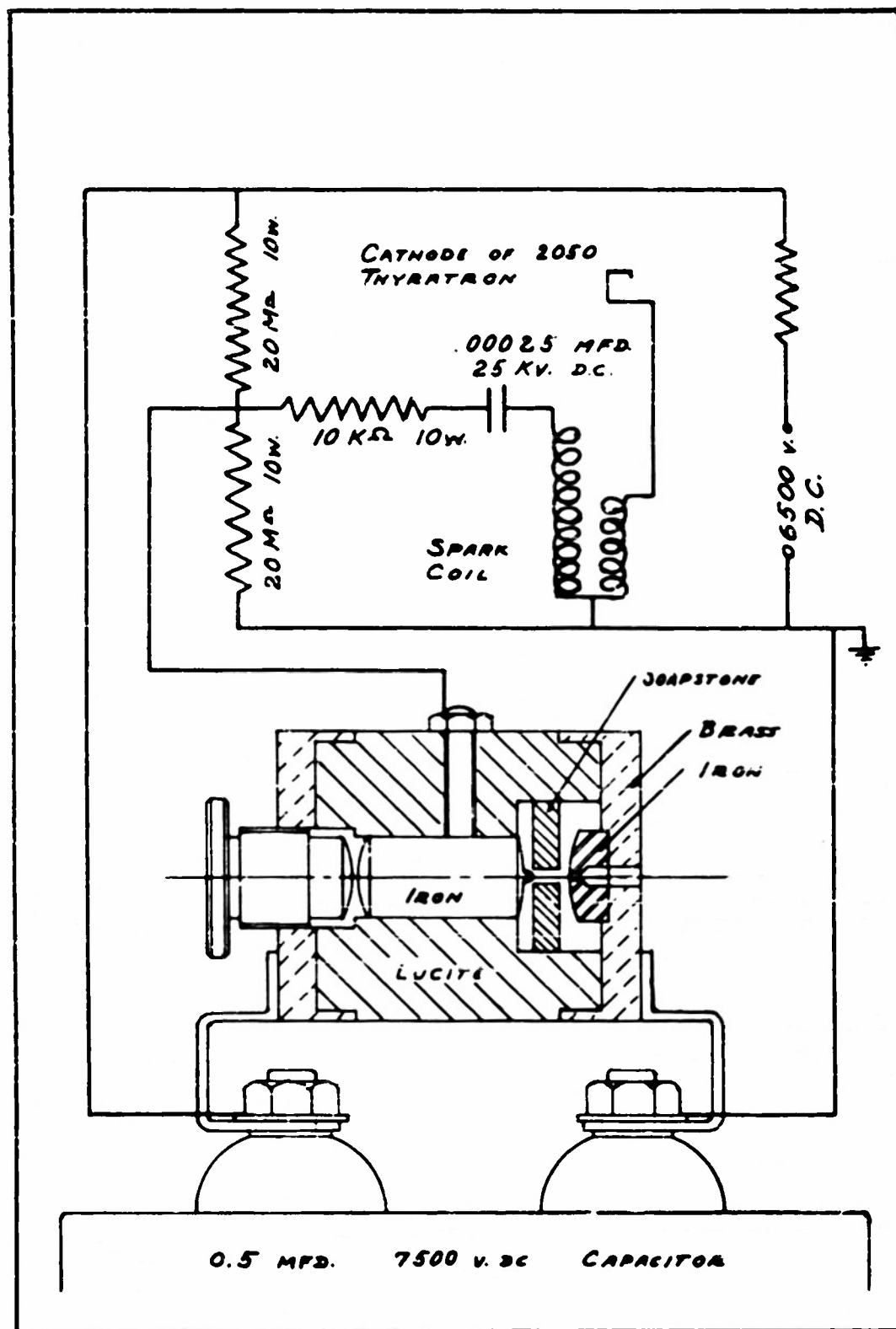
SPARK ASSEMBLY
