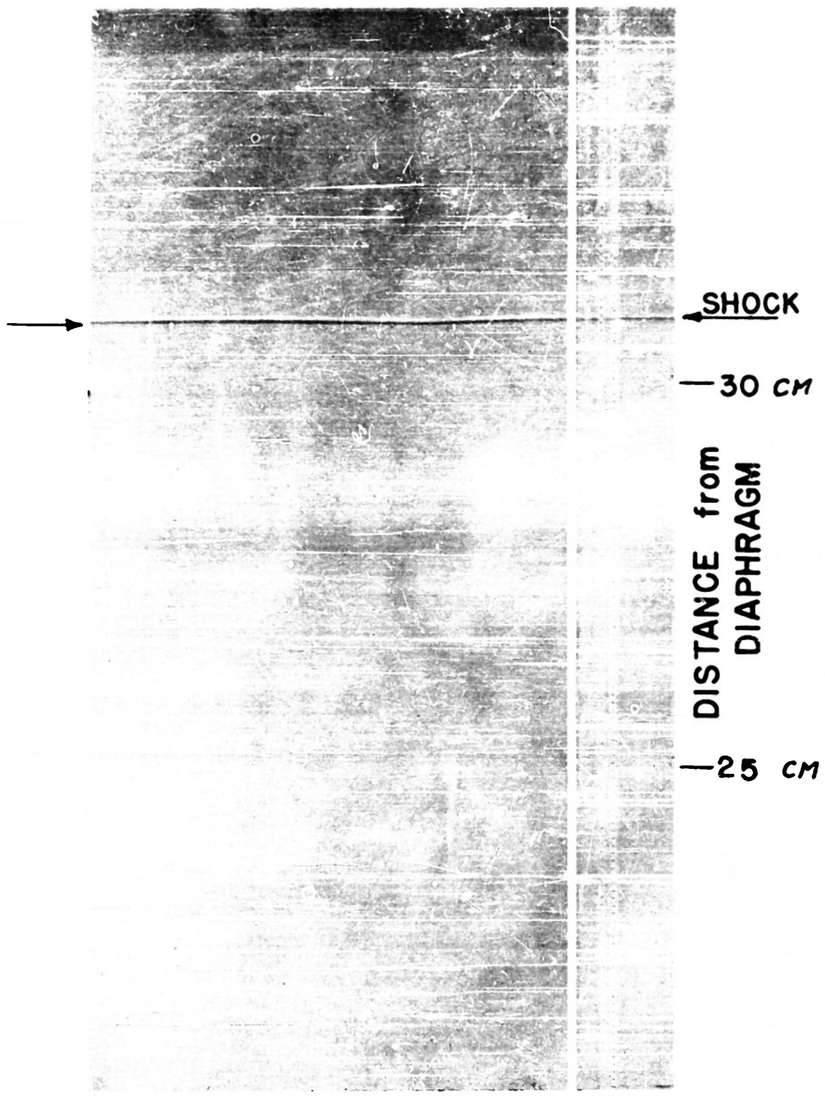
FIG. 5 SHADOWGRAPH
