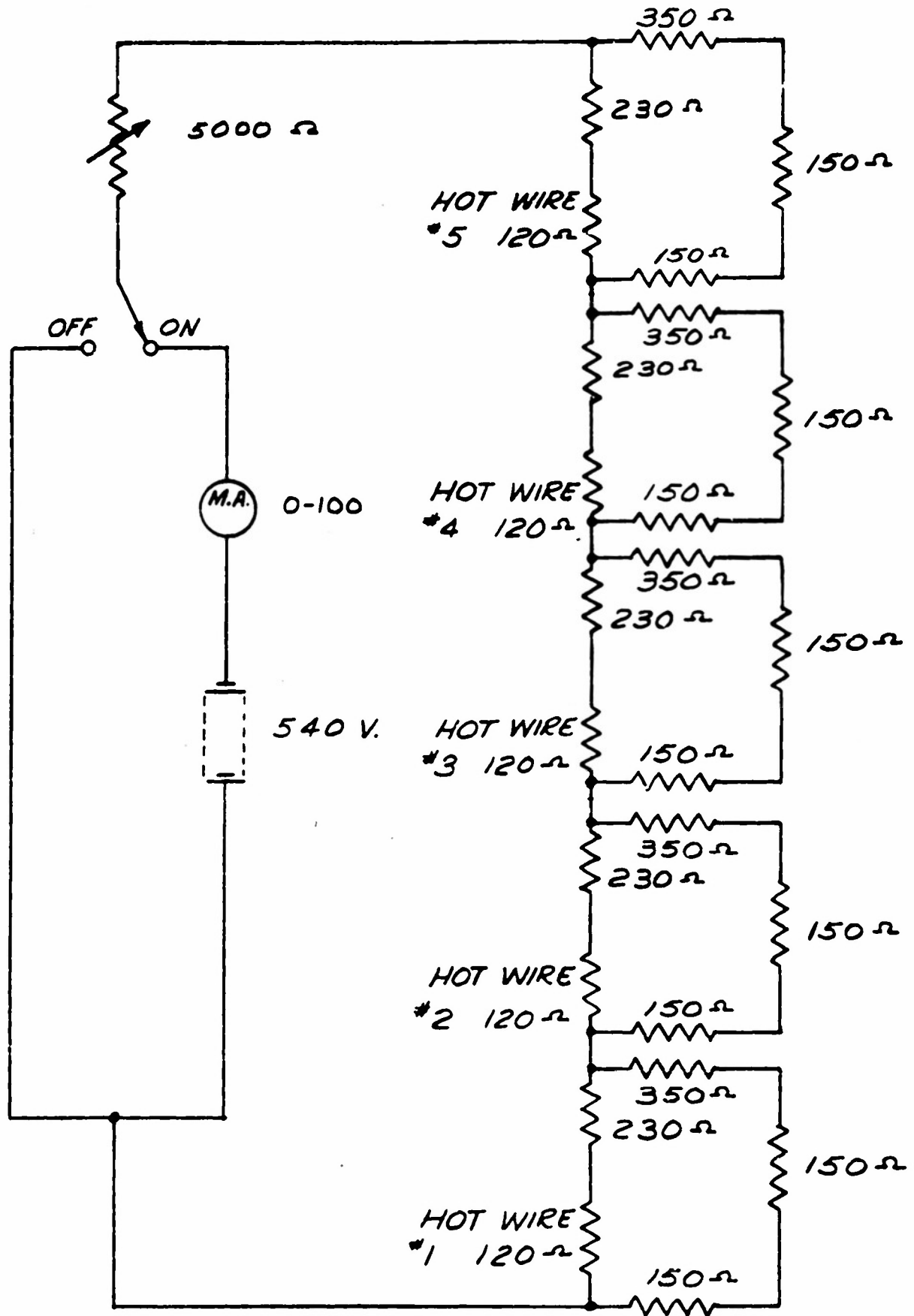
FIG. 6 DC CIRCUIT SCHEMATIC
