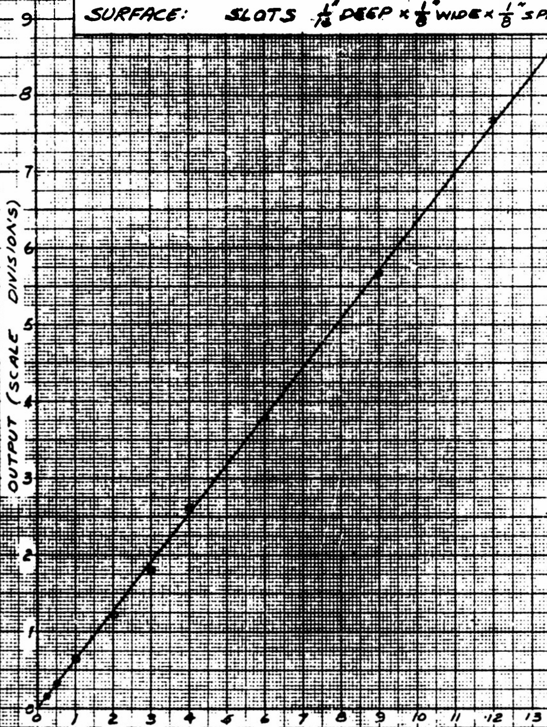
FIG. 25 ANEMOMETER CALIBRATION ROUGHNESS TEST
