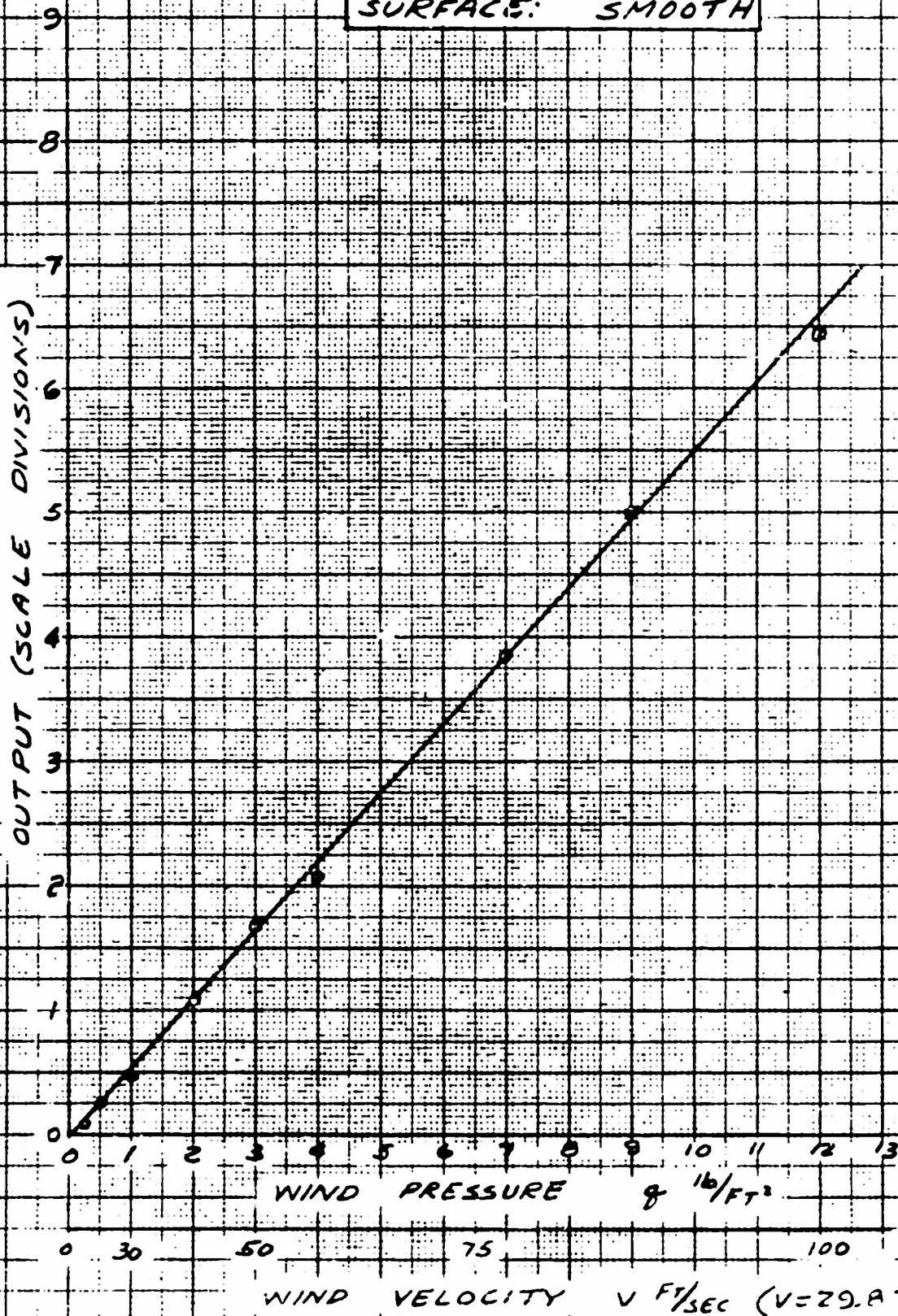
FIG 16 ANEMOMETER CALIBRATION ROUGHNESS TEST
