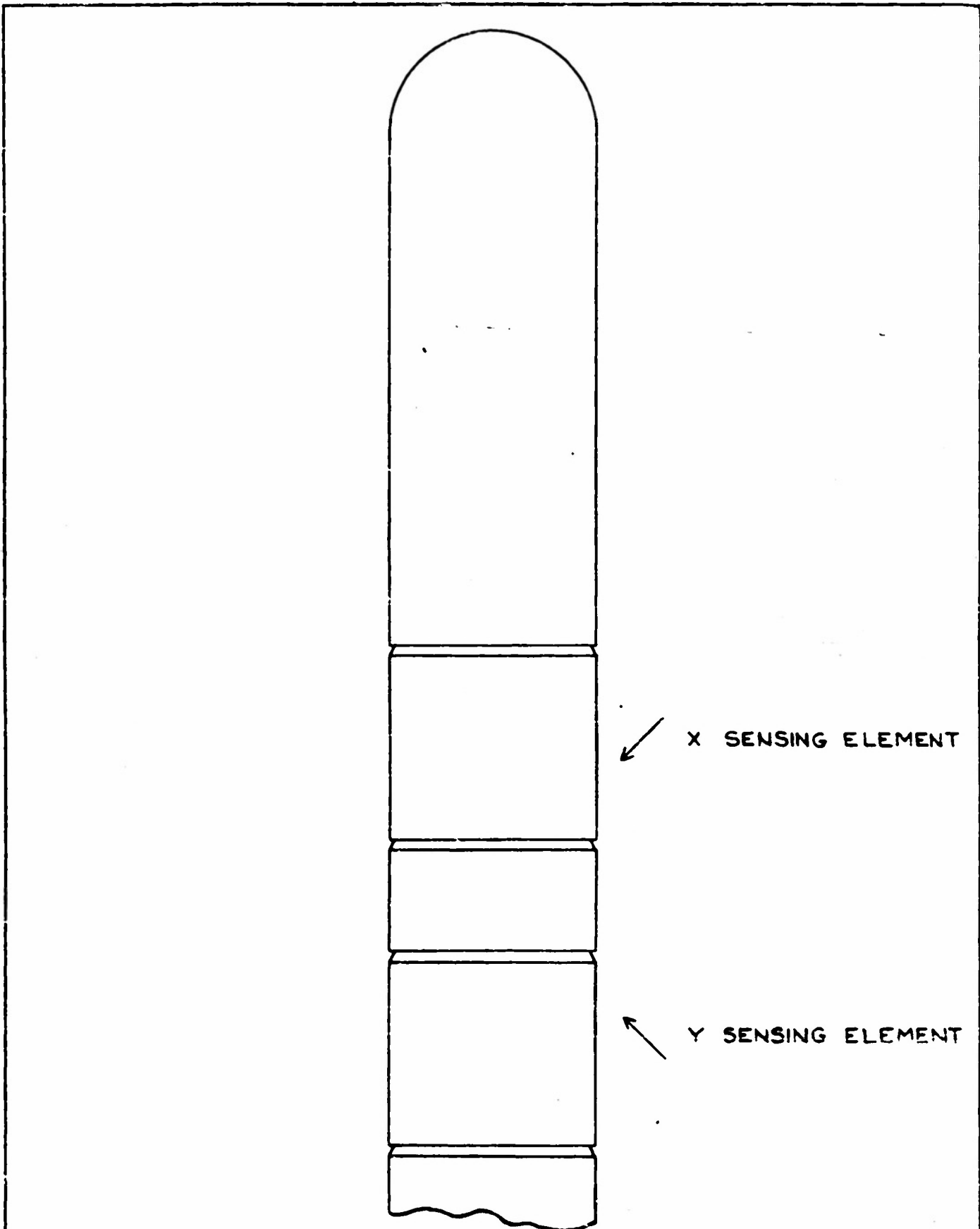
FIGURE 13 ANEMOMETER OUTLINE (1/2 SIZE)
