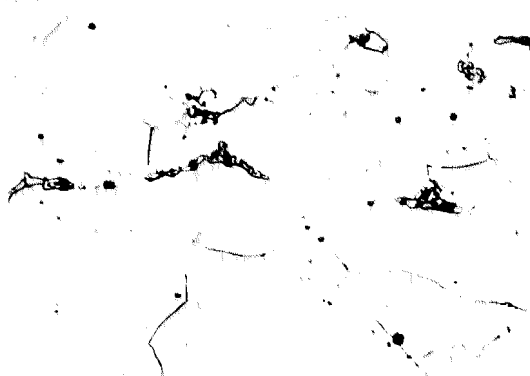
X1000 -B- PICRAL WINDSHIELD- SAME AREA AS A. LARGE CARBIDES AT GRAIN BOUNDARIES.
