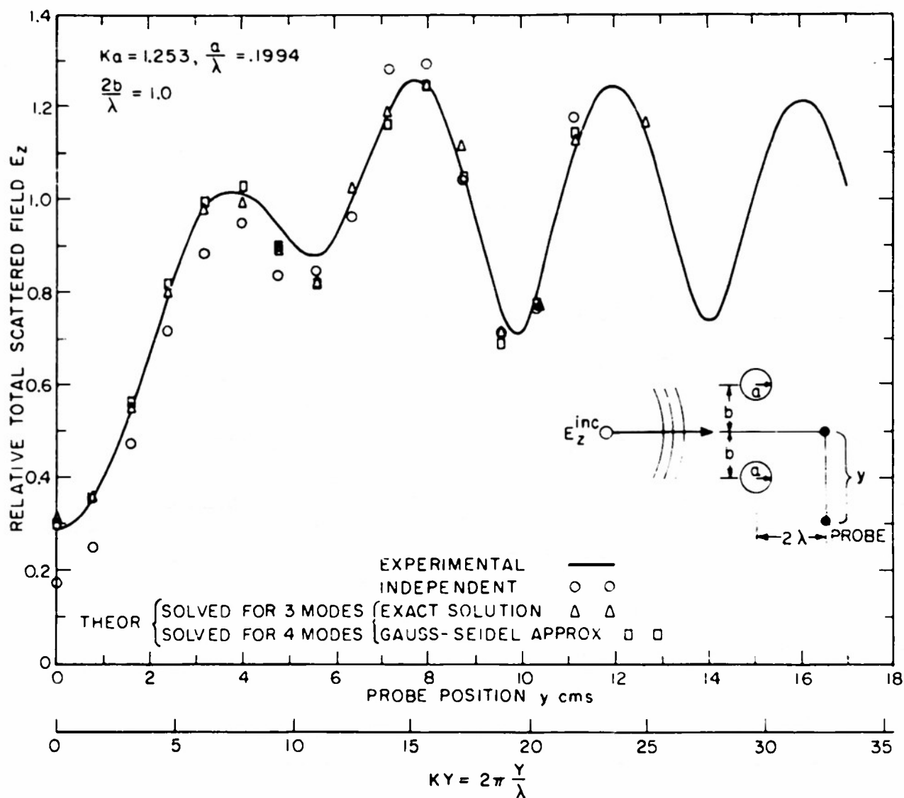
FIG. 15 EXPERIMENTALLY MEASURED DIFFRACTED FIELD FROM TWO CYLINDERS AND COMPARISON WITH VARIOUS THEORETICAL APPROXIMATIONS FOR Ka = 1.253 , AS A FUNCTION OF PROBE POSITION
