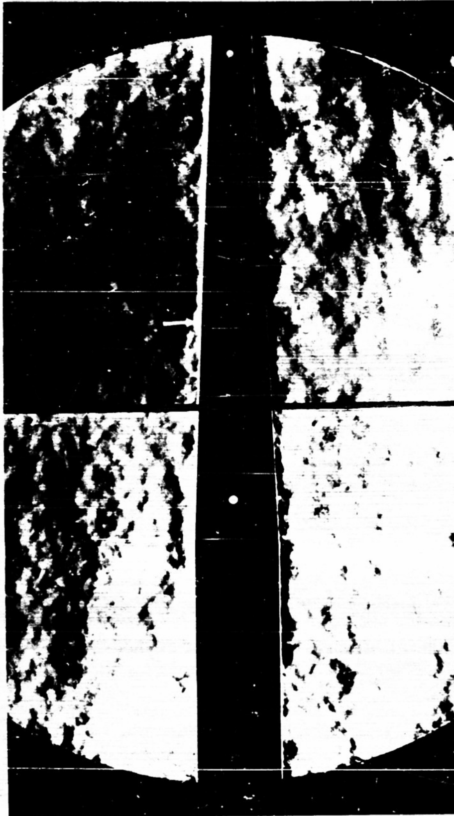
MACH 4.25, TUNNEL 2, Re \sim 1.6 \times 10^6 , ↓ INDICATES TRANSITION POINT
