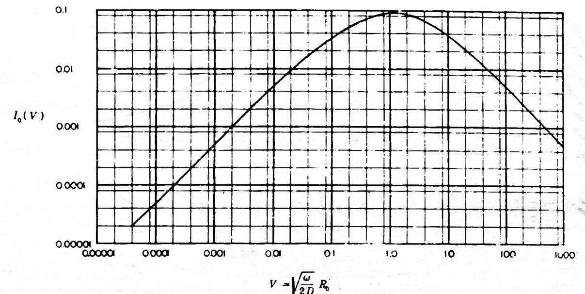
Figure 4 - Plot of I_0(V) = \int_1^\infty e^{-V(z-1)} \frac{\sin V(z-1)}{x^3} dx
