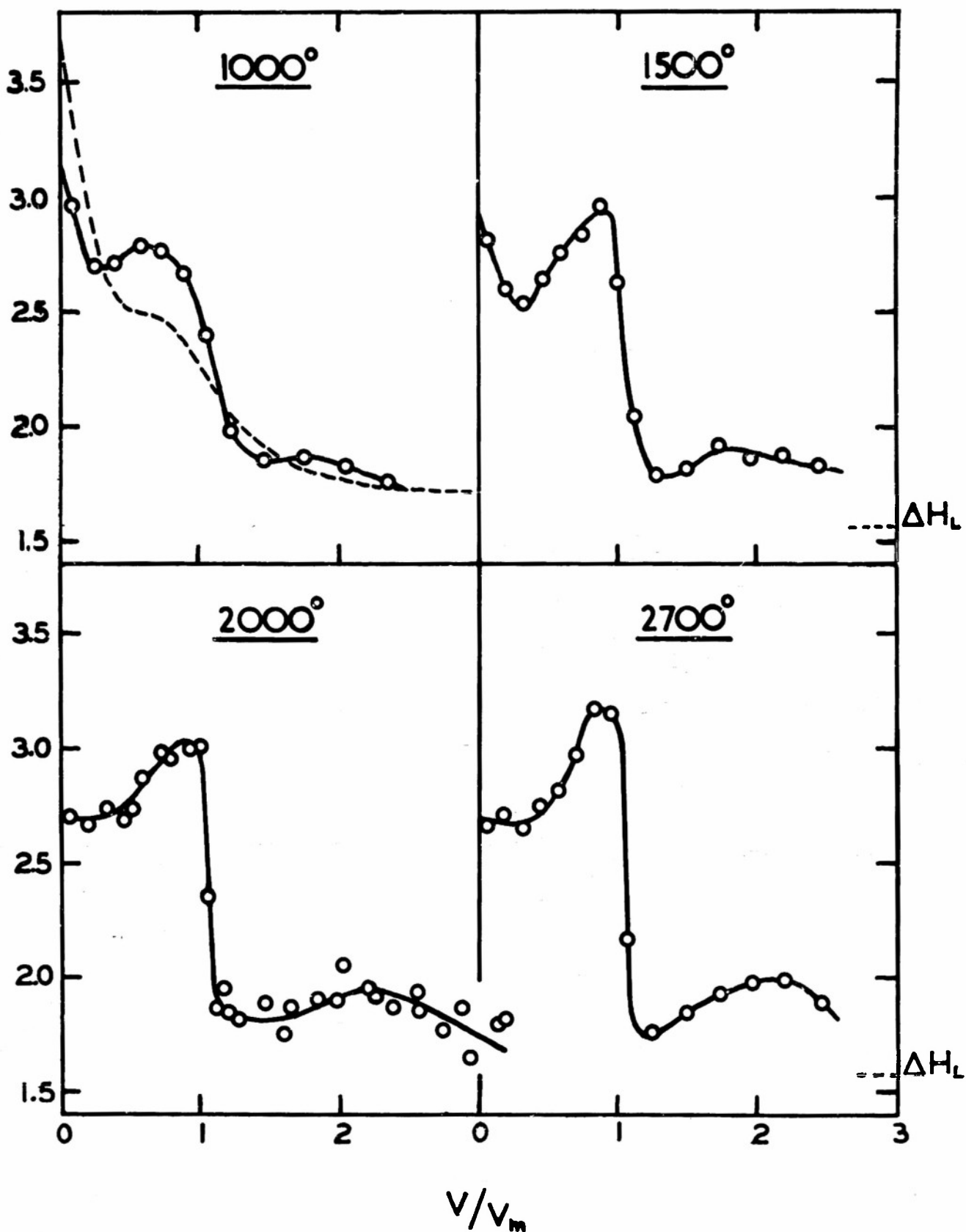
FIG. 2. HEATS OF ADSORPTION OF ARGON ON CARBON BLACKS AT -195^{\circ}\text{C} . DOTTED LINE REPRESENTS UNTREATED BLACK. TEMPERATURES OF GRAPHITIZATION ARE INDICATED.
