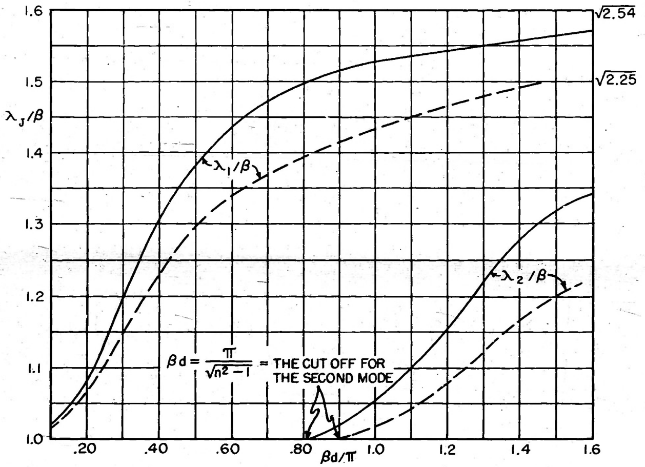
FIG. 4 \lambda_j/\beta VS. \beta d , FOR n^2 = 2.54 AND 2.25 , 0.10\pi \leq \beta d \leq 1.6\pi n^2 = 2.54 ———, n^2 = 2.25 - - - -
