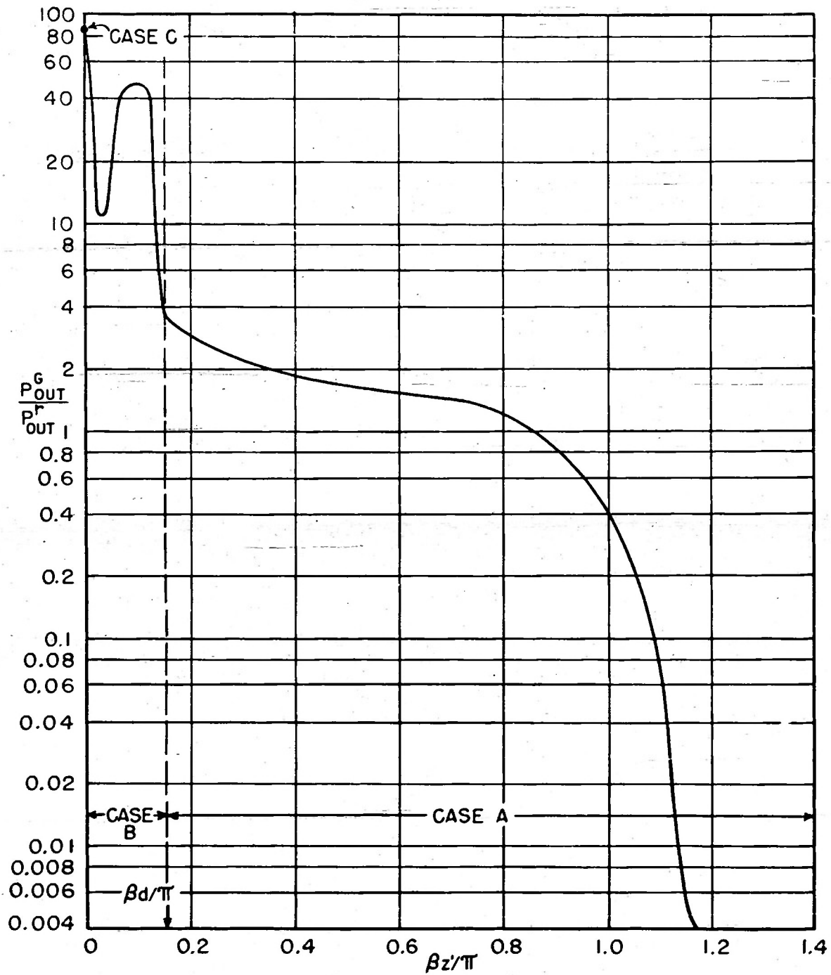
FIG. 20 \frac{P_{OUT}^G}{P_{OUT}^r} AS A FUNCTION OF \beta z' FOR \beta d = 0.15\pi n^2 = 2.54 THIS INCLUDES CASES A, B AND C AS \beta z' VARIES.
