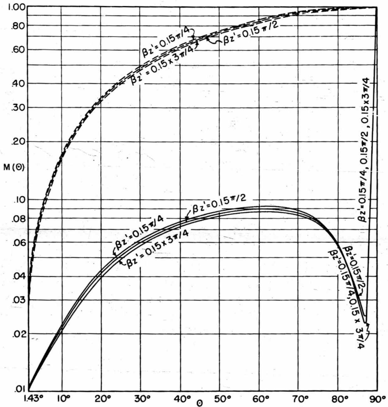
FIG. II FIELD PATTERNS FOR CASE B, \beta d = 0.15\pi , M(\theta) VS \theta WITH FIELD PATTERNS WITH \beta d = 0 FOR COMPARISON BR = 239 , n = 2.54 , \beta d = 0.15\pi —, \beta d = 0 --- \beta z' = 0.15 \frac{\pi}{4} , 0.15 \frac{\pi}{2} , 0.15 \times \frac{3\pi}{4}
