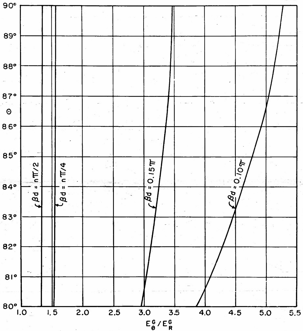
FIG. 15 E_{\theta}^G/E_R^G VS. \theta OVER THE RANGE OF SIGNIFICANT VALUES OF |E^G| FOR \beta d = n\pi/2, n\pi/4, 0.15\pi, 0.10\pi AND FOR n^2 = 2.54
