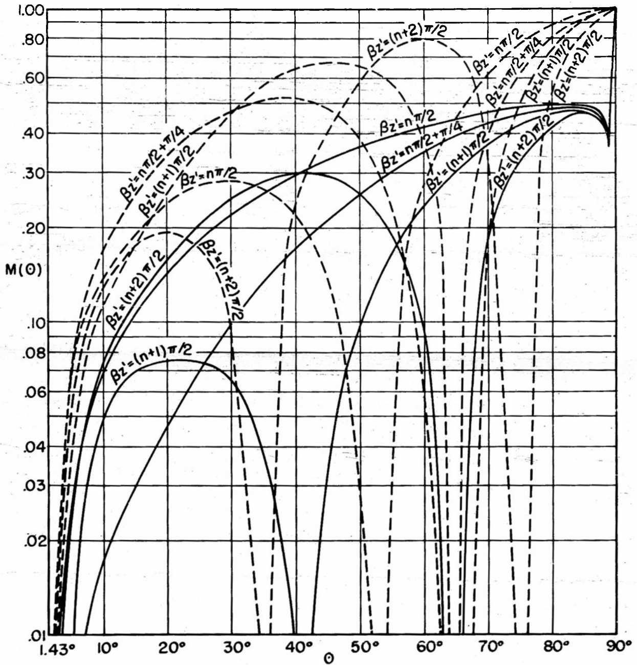
FIG. 9 FIELD PATTERNS FOR CASE A, \beta d = \frac{n\pi}{2} WITH FIELD PATTERNS WITH \beta d = 0 FOR COMPARISON \beta R_0 \approx 239 , n^2 = 2.54 , \beta d = \frac{n\pi}{2} —, \beta d = 0 ---, \beta z' = \frac{n\pi}{2} , \frac{n\pi}{2} + \frac{\pi}{4} , (n+1)\frac{\pi}{2} , (n+2)\frac{\pi}{2}
