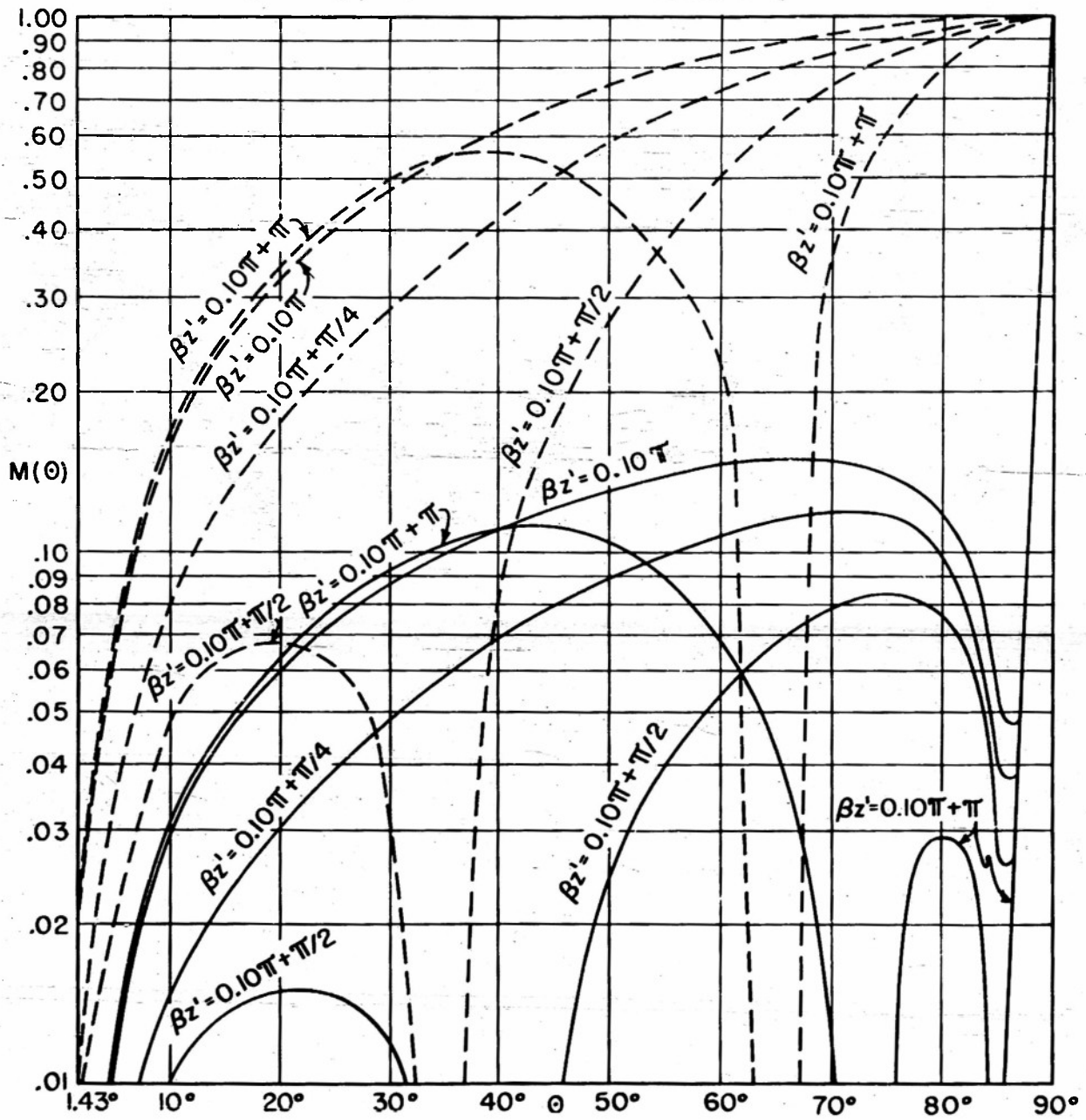
FIG. 6 FIELD PATTERNS FOR CASE A, \beta d = 0.10\pi , M(\theta) VS. \theta WITH FIELD PATTERNS WITH \beta d = 0 FOR COMPARISON. \beta R_0 \approx 239 , n^2 = 2.54 , \beta d = 0.10\pi ———, \beta d = 0 - - - - \beta z' = 0.10\pi, \pi/4 + 0.10\pi, \pi/2 + 0.10\pi, \pi + 0.10\pi
