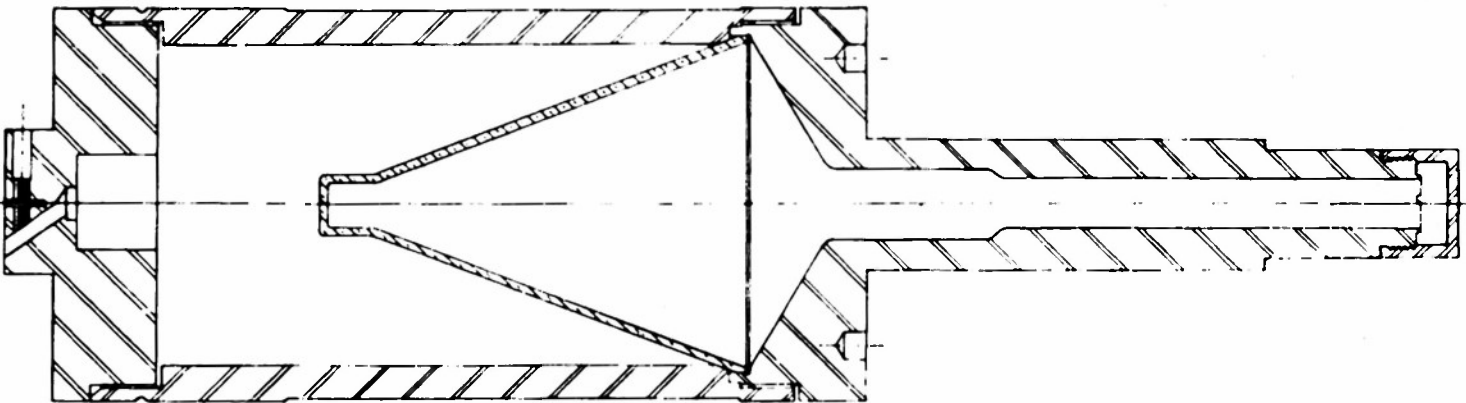
Fig. 4. Penetration Assembly. DRC321 Body, DR8398 Pressed Cone.
