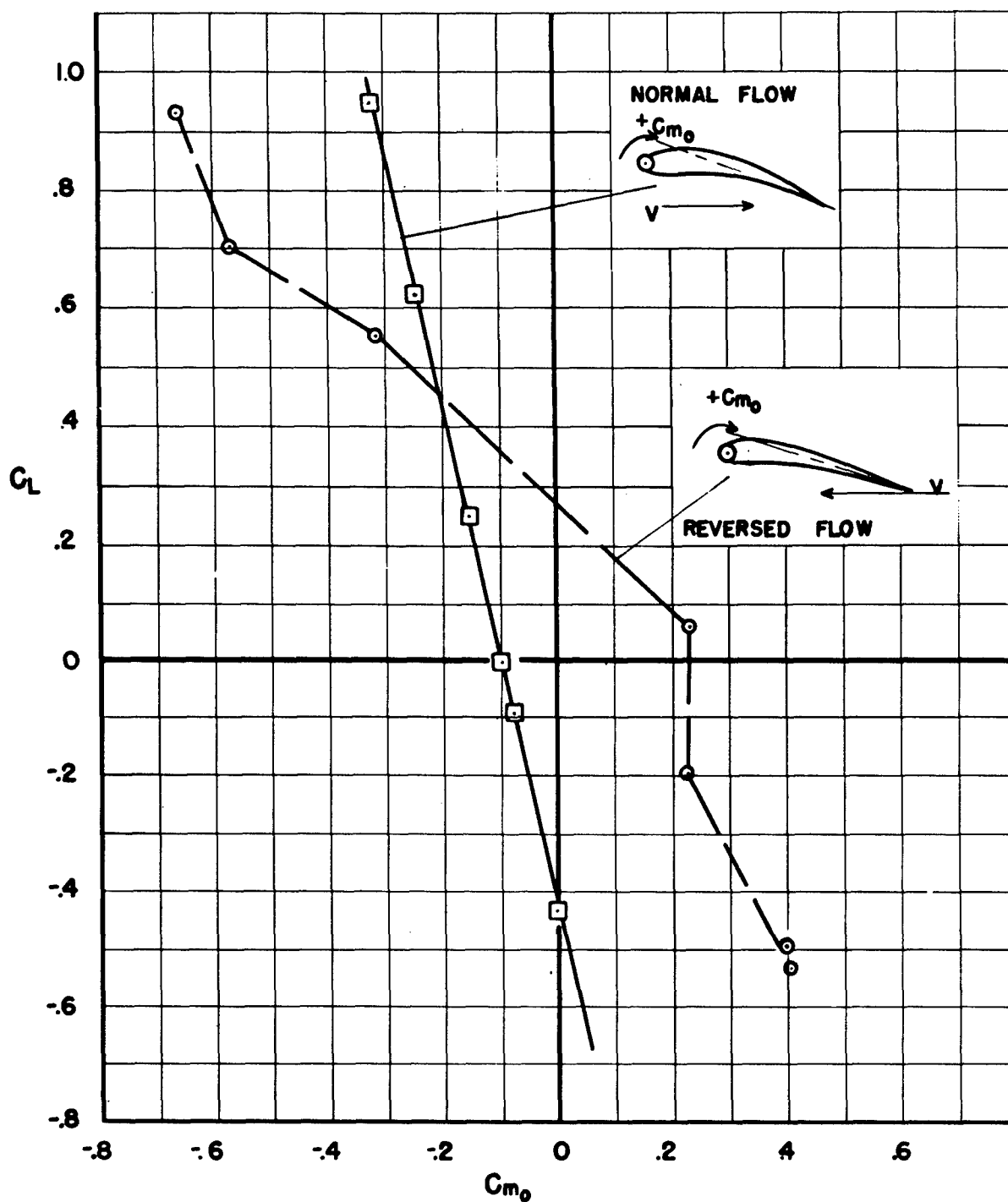
Figure 17b: Variation of Lift Coefficient With Moment Coefficient for a Goettingen 420 Airfoil of Aspect Ratio 5 in Normal and Reversed Flow.
