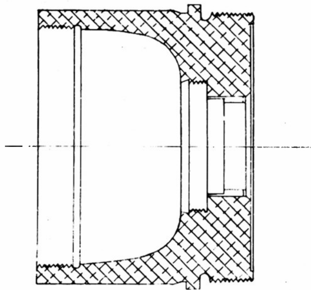
Fig. 2. Projectile Chamber. Firestone Drawing No. DRC442.
