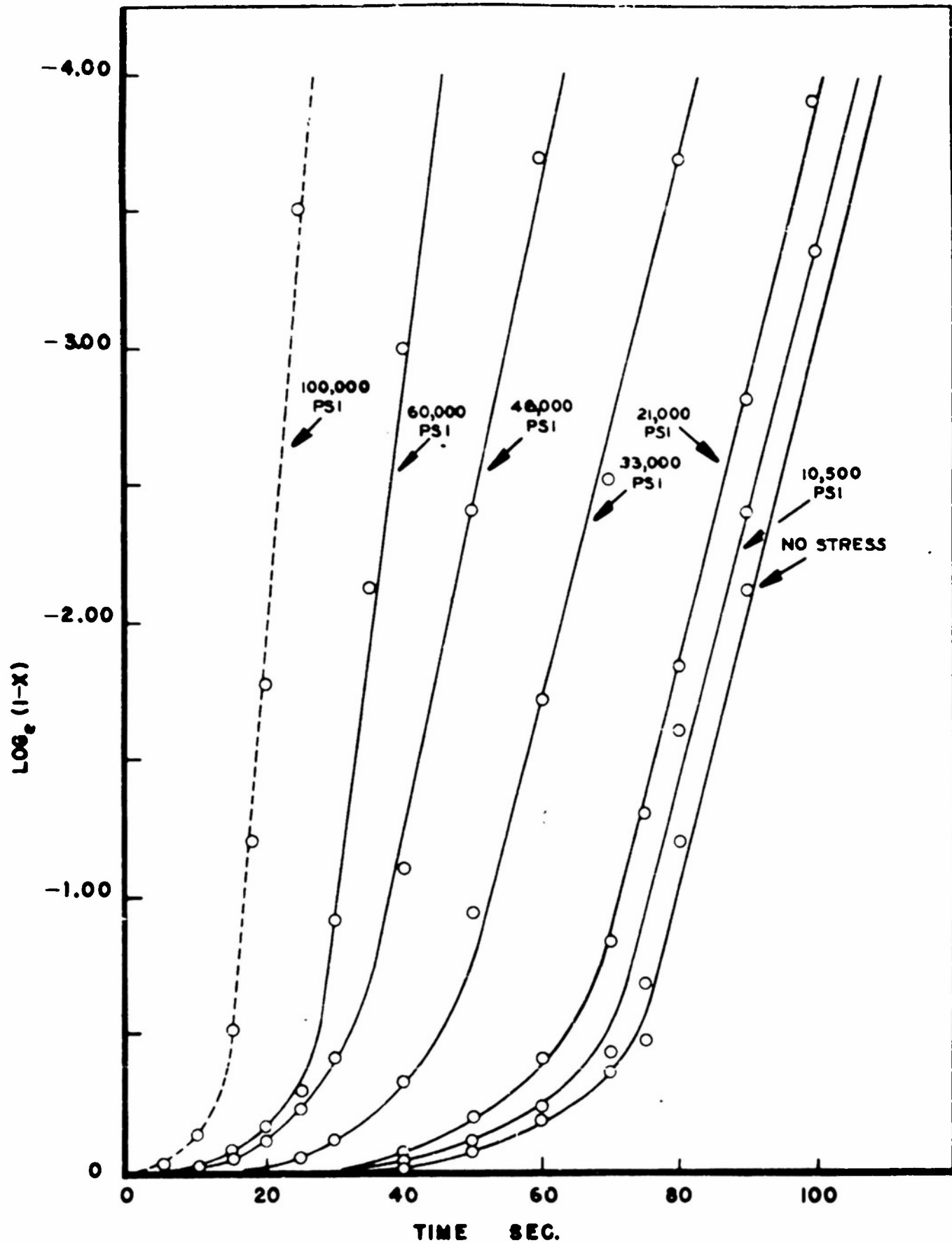
FIG. 13 RELATIONSHIP SHOWING THE VARIATION IN THE RATE OF DECOMPOSITION OF RESIDUAL AUSTENITE WITH APPLIED STRESS IN AISI 1088 STEEL, ISOTHERMALLY TRANSFORMED AT 700° F
