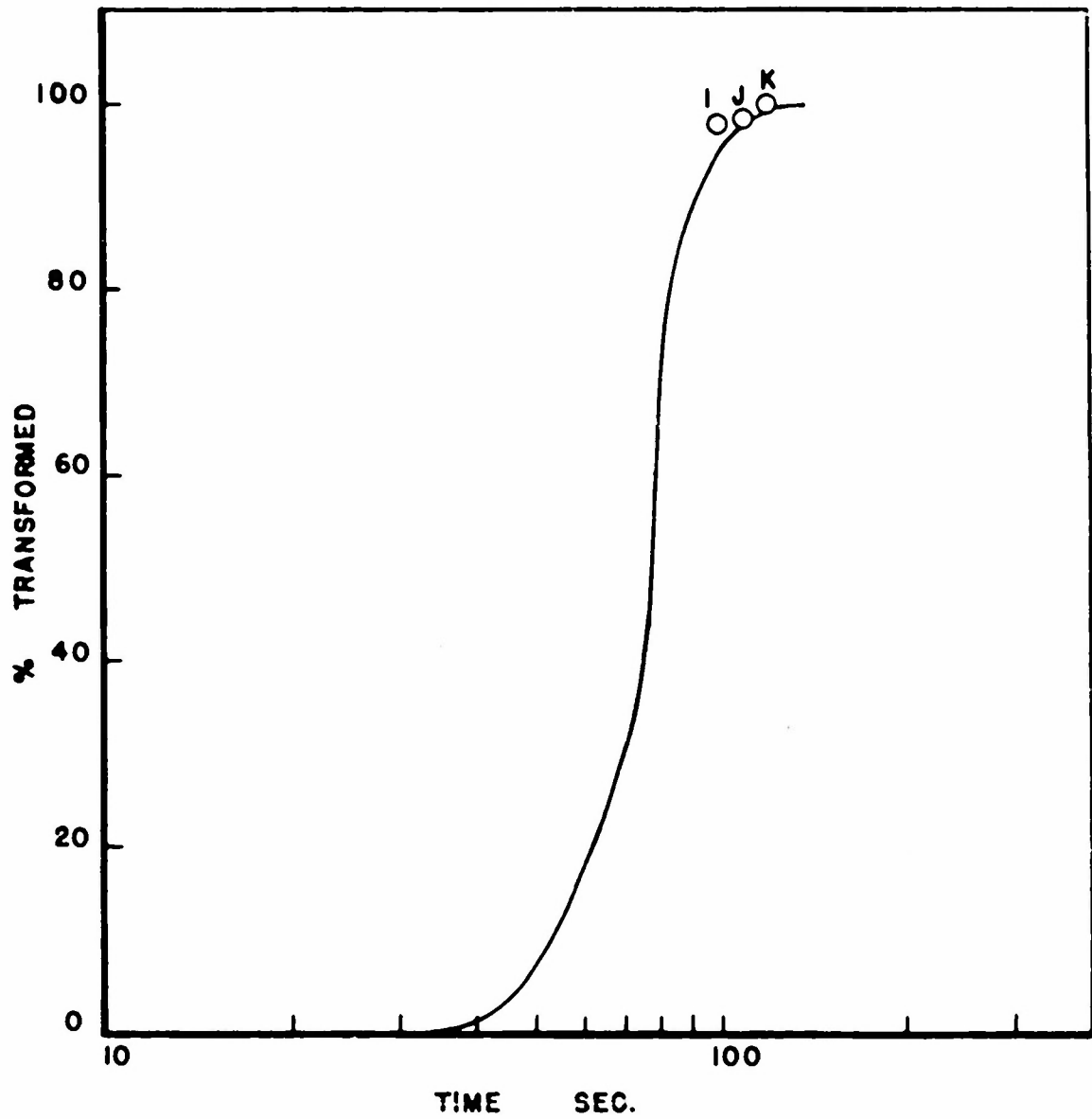
FIG. 9 AISI 1085 STEEL, ISOTHERMALLY TRANSFORMED AT 700° F UNDER NO APPLIED STRESS
