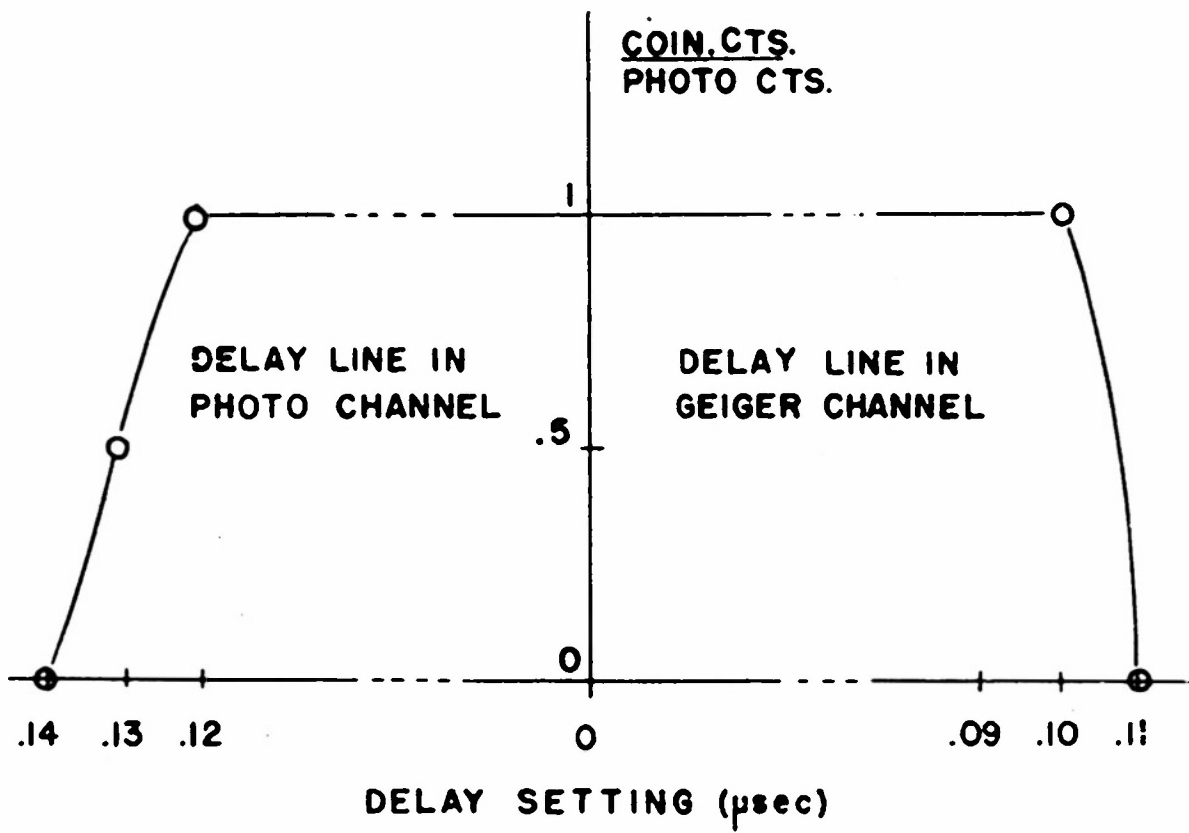
RESOLUTION OF COINCIDENCE CIRCUIT
