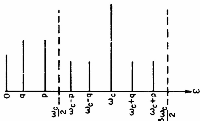
FIGURE 2.8 FREQUENCY SPECTRUM OF FIRST ORDER MODULATOR
