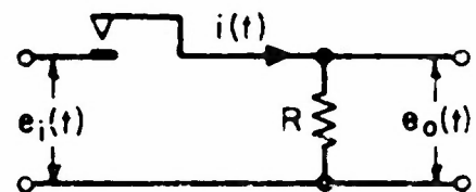
FIGURE 2.6 FIRST ORDER MODULATOR USING KEYED PARAMETER
