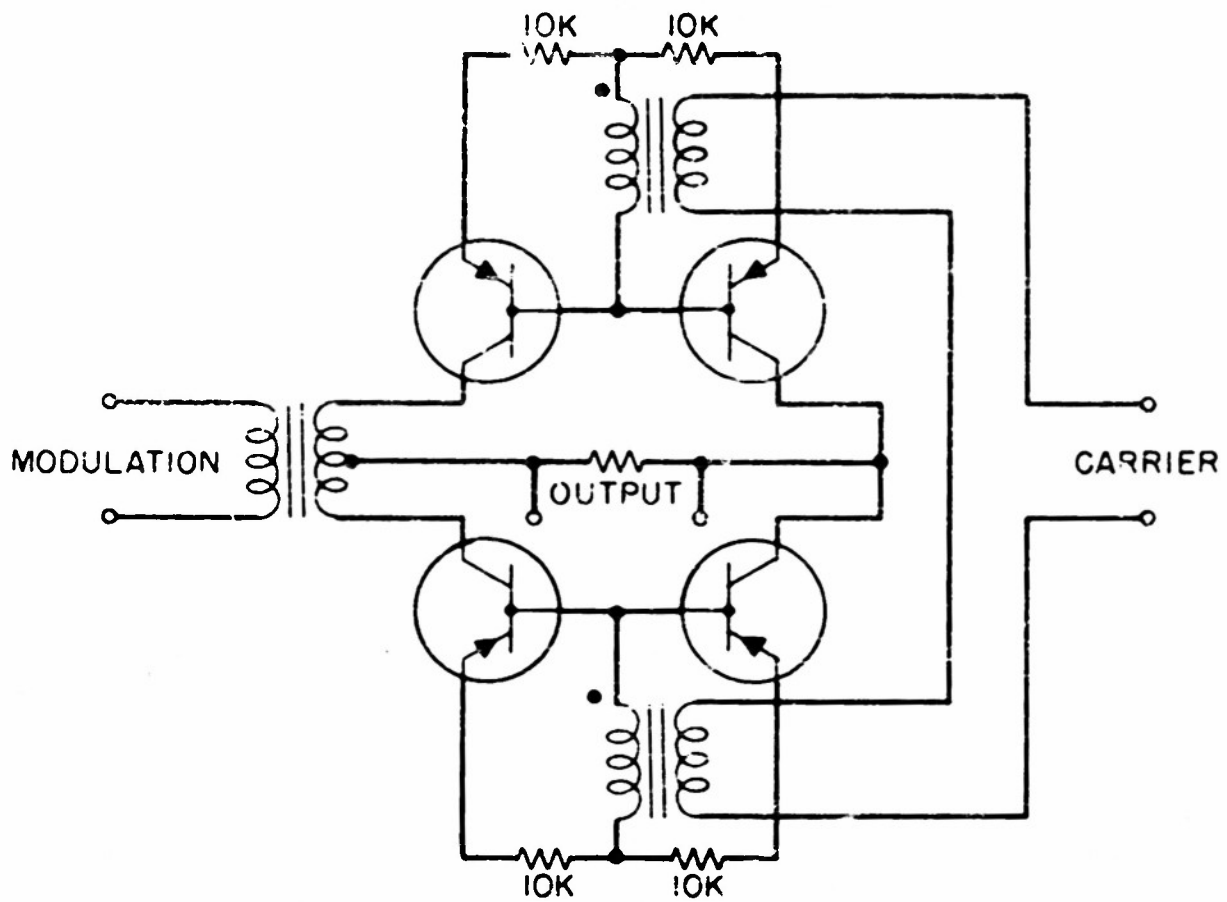
FIGURE 3.22 FULL WAVE SCHREINER DUAL
