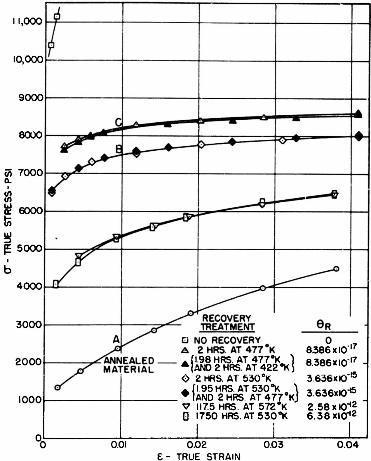
FIG. 2 EFFECT OF RECOVERY ON THE TENSILE CURVES AT 298 °K OF HIGH PURITY ALUMINUM PRESTRAINED 15 % AT 78 °K.
