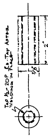
SWAY BRACE BUSH. C.R.S. FULL SCALE
