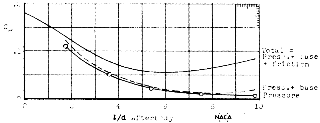
Figure 8.- Qualitative breakdown of afterbody drag for models of reference 8. R_b/R_m = 0.458 ; M = 1.4 .
