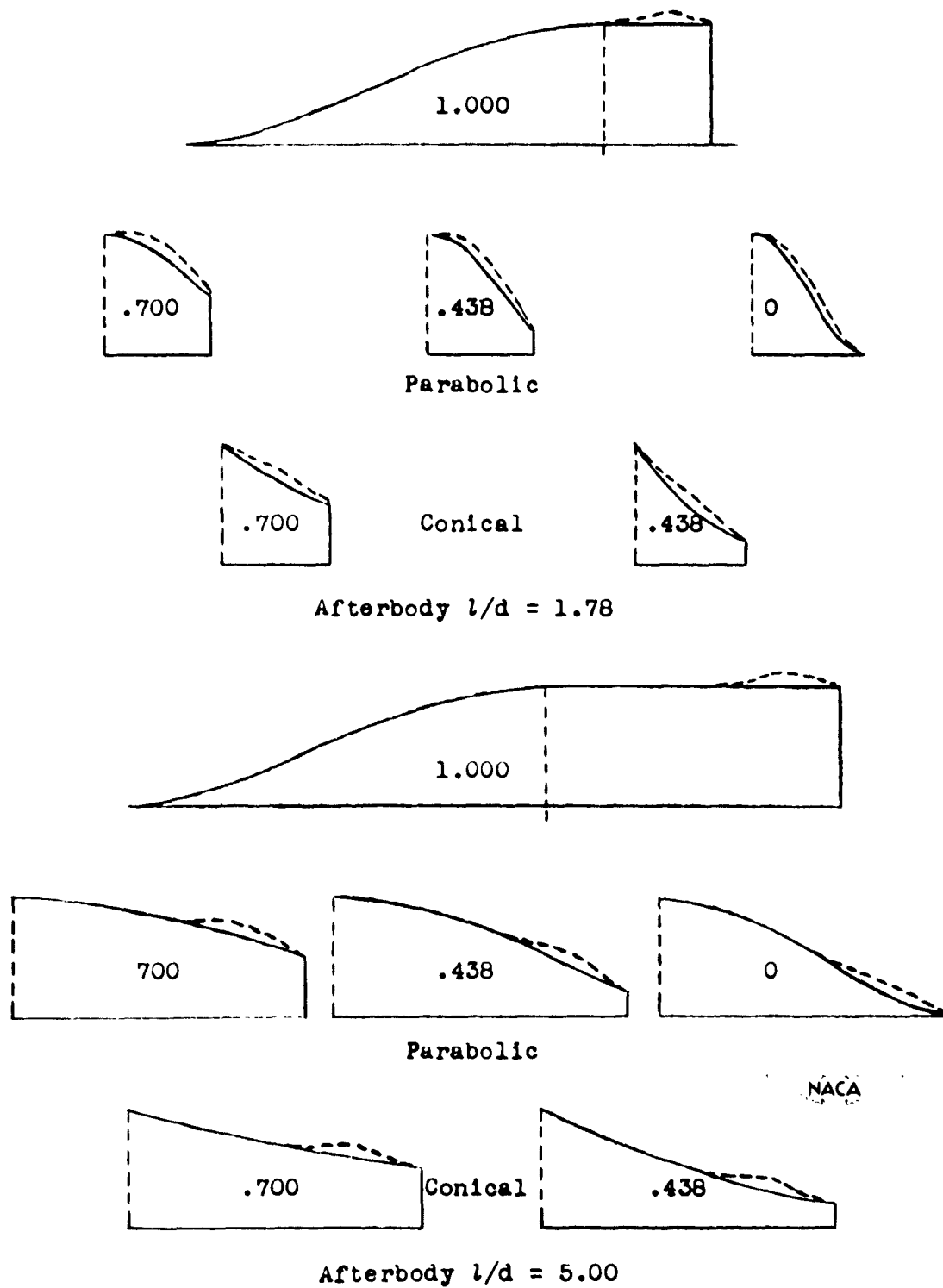
Figure 11.- Longitudinal area distributions.
