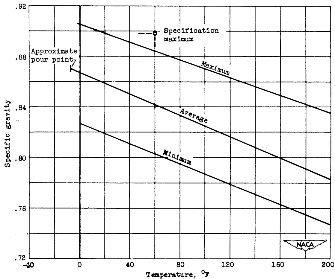
Figure 3. - Continued. Variation of specific gravity with temperature.
