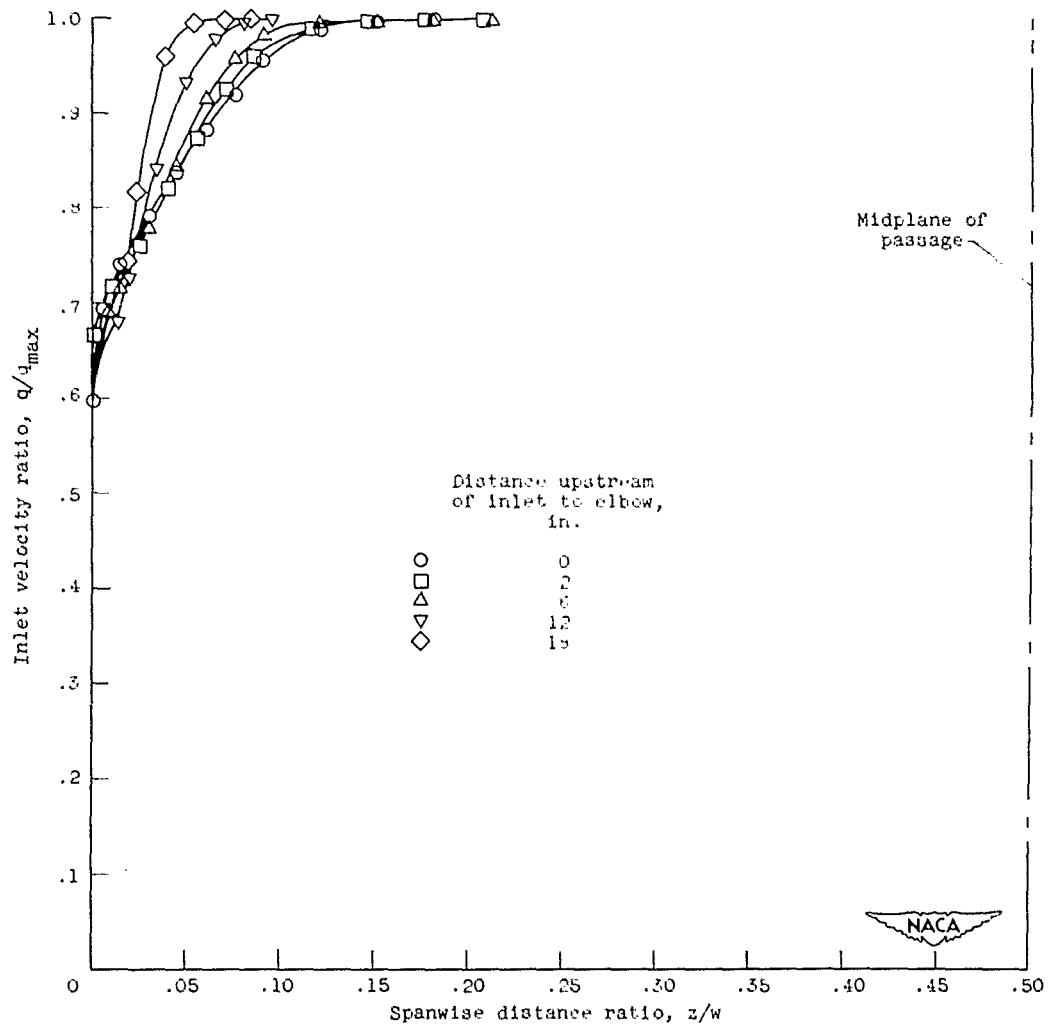
(a) 0.5-Inch spoiler.
