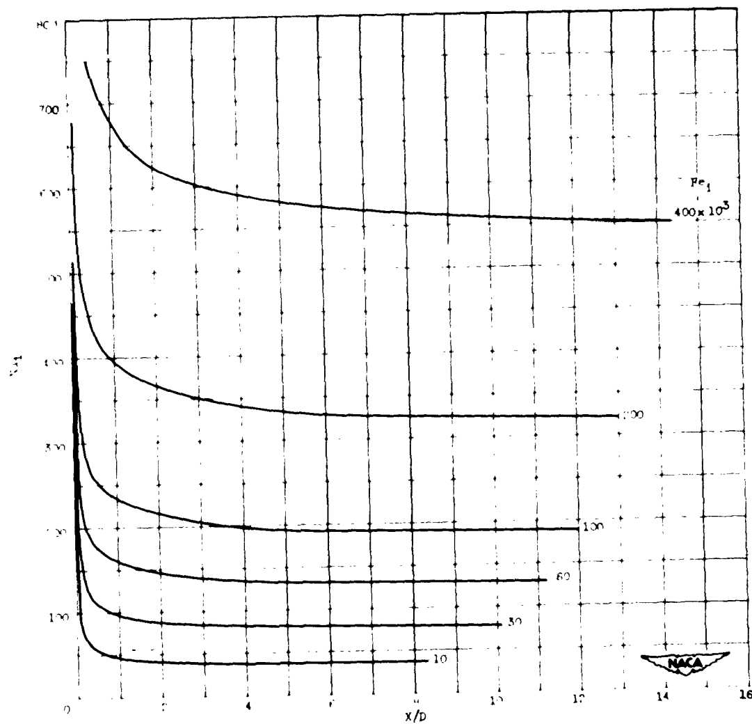
Figure 14. - Variation of Nusselt number with X/D and Reynolds number for gas flowing between parallel flat plates. Pr = 0.73 . Uniform heat flux, uniform initial temperature distribution, and fully developed velocity distribution.
