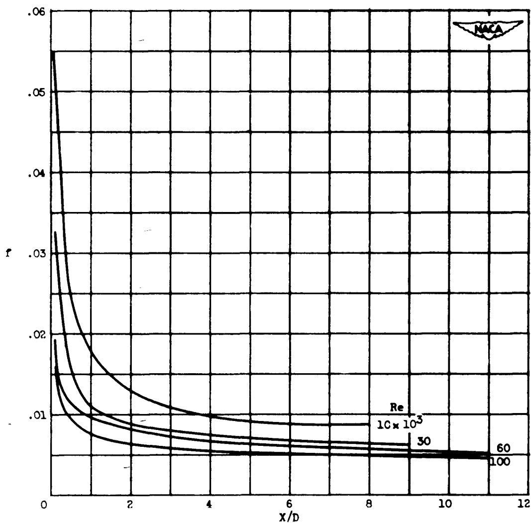
Figure 32. - Variation of friction factor based on static-pressure gradient with X/D and Reynolds number for flow between parallel flat plates. Constant properties.
