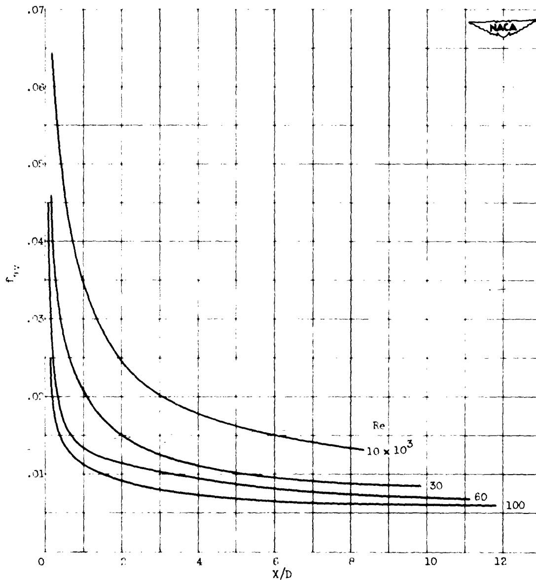
Figure 33. - Variation of average friction factor based on static-pressure drop with X/D and Reynolds number for flow between parallel flat plates. Constant properties.
