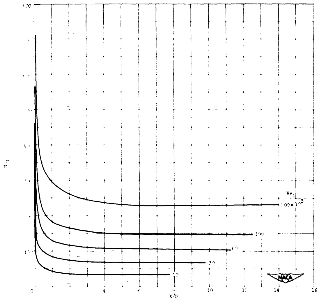
Figure 14. - Continued. Variation of Nusselt number with X/D and Reynolds number for gas flowing between parallel flat plates. Pr = 0.73 . Uniform heat flux, uniform initial temperature distribution, and fully developed velocity distribution.
