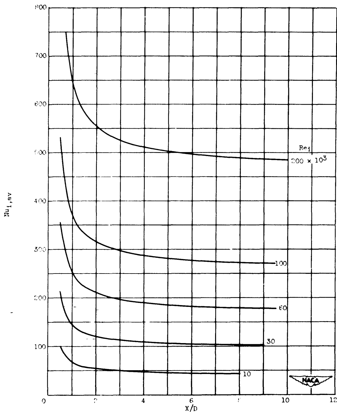
Figure 16. - Concluded. Variation of average Nusselt number defined by equation (25) with X/D and Reynolds number for gas flowing between parallel flat plates. Pr, 0.73 . Uniform heat flux, uniform initial temperature distribution, and fully developed velocity distribution.
