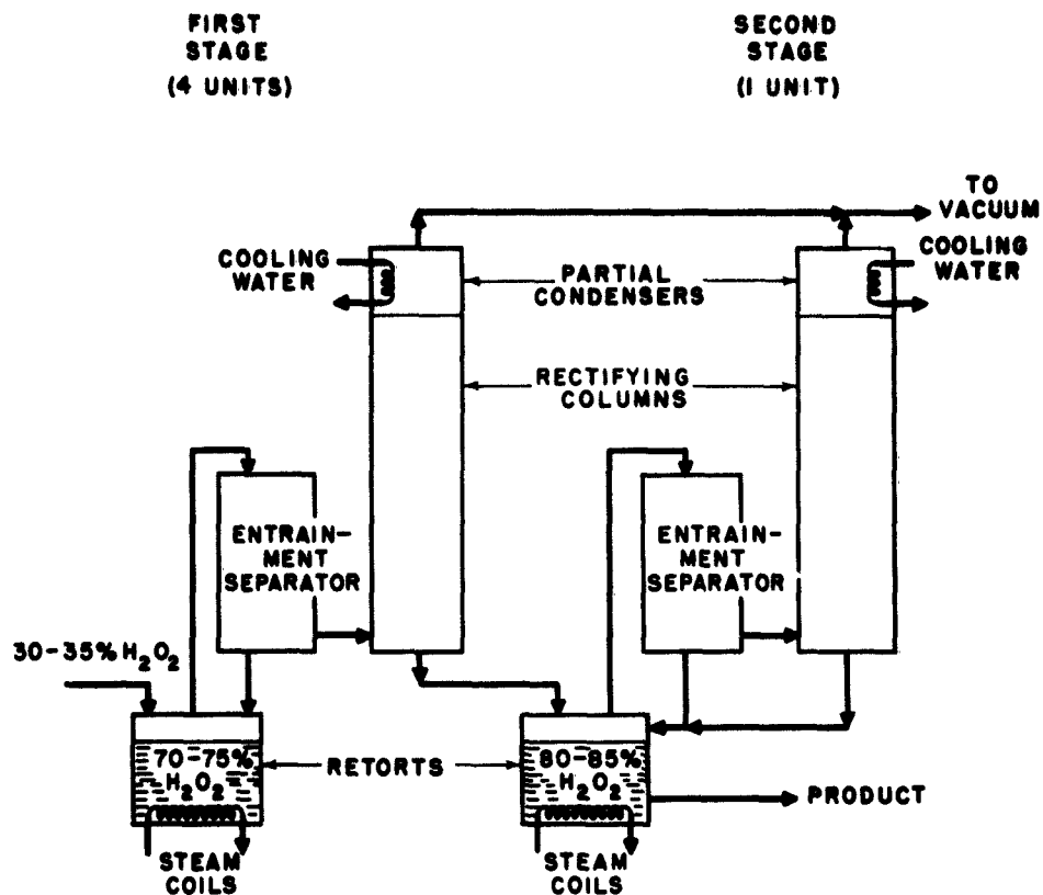
FIG. 1- FLOWSHEET FOR CONCENTRATION OF HYDROGEN PEROXIDE, E.W.M. PROCESS.
