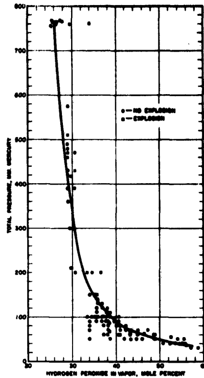
FIG. 7-EFFECT OF TOTAL PRESSURE ON IGNITION LIMIT SEMI-OPEN INITIATION
