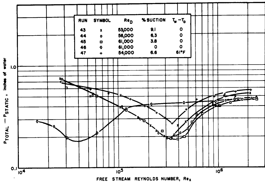
FIG. 17 THE EFFECT OF HEATING ON TRANSITION. THE EFFECT OF BOUNDARY LAYER SUCTION RATE ON THE ADIABATIC PERFORMANCE OF THE SYSTEM FOR THE SAME Re_D IS ALSO SHOWN.
