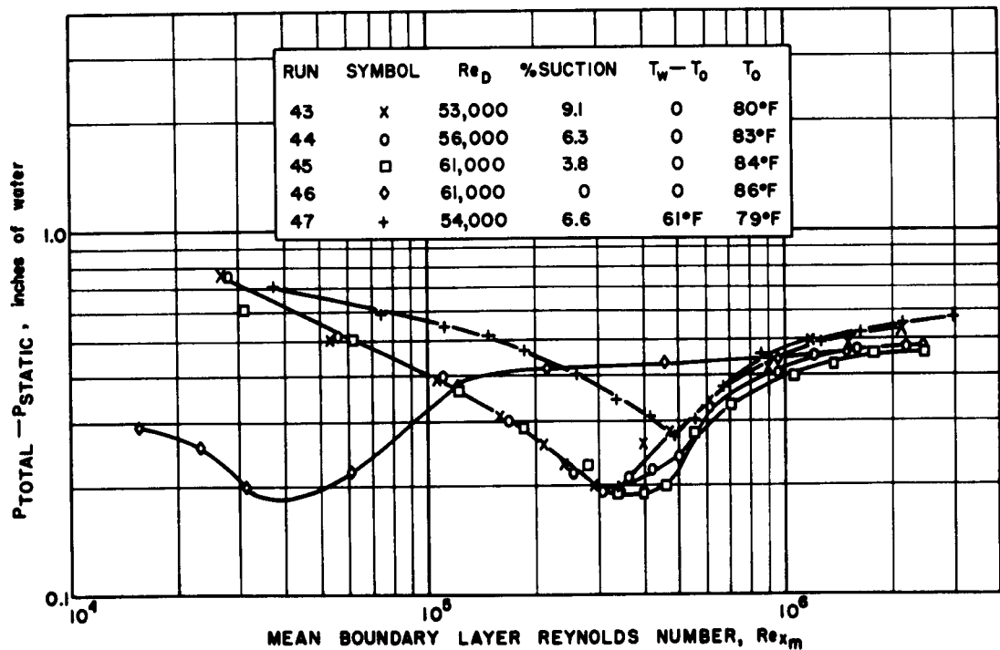
FIG. 18 THE EFFECT OF HEATING ON TRANSITION. SAME AS FIG. 17, EXCEPT THAT THE MEAN BOUNDARY LAYER REYNOLDS NUMBER IS USED IN PLACE OF THE FREE STREAM REYNOLDS NUMBER.
