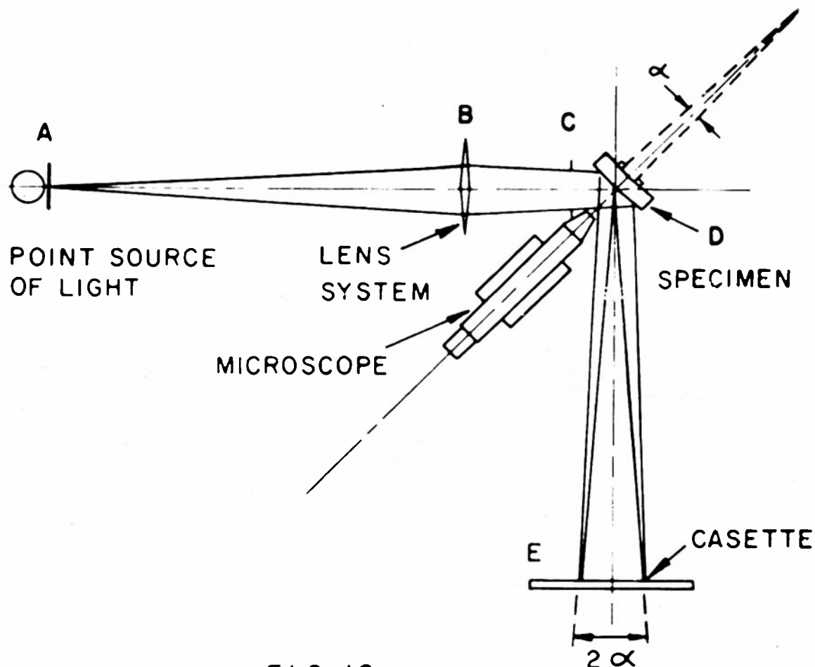
FIG. 16 SCHEMATIC DIAGRAM OF OPTICAL GONIOGRAPH
