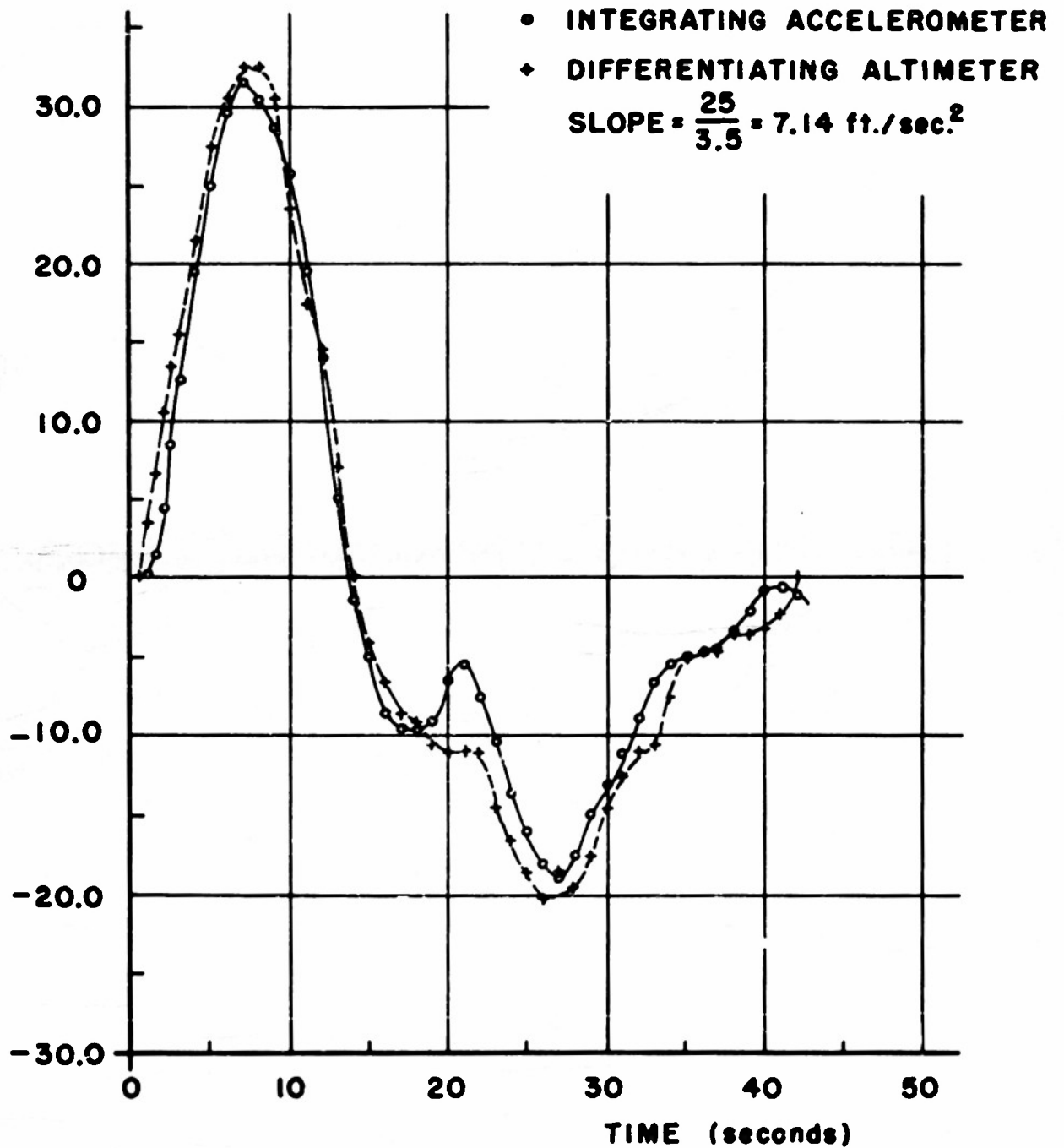
FIGURE 11. RUN 1969; 3-18-53 at 2:30 p.m. H_p = 3000 \text{ ft.}
