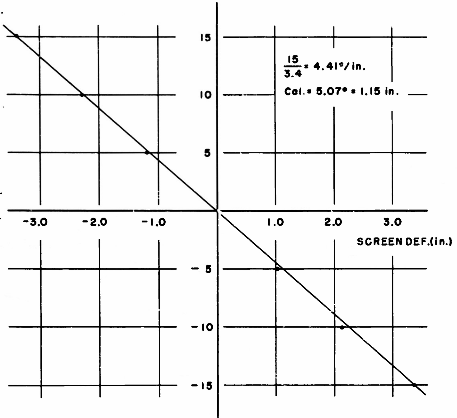
FIGURE 8. CALIBRATING C-1 GYRO IN LABORATORY ON 5-116 SCREEN.
