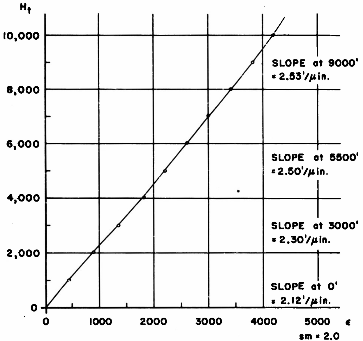
FIGURE 5. PRESSURE ALTITUDE vs. STRAIN OUTPUT, ELECTRIC ALTIMETER.
