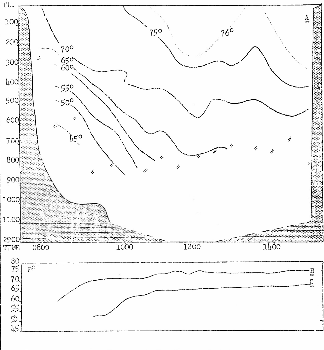
Figure 5. A TEMPERATURE-DEPTH PROFILE B&C TEMPERATURES AT 305 AND 625 FEET Data from Cruise T-304 Miami to Cat Cay January 4, 1953.
