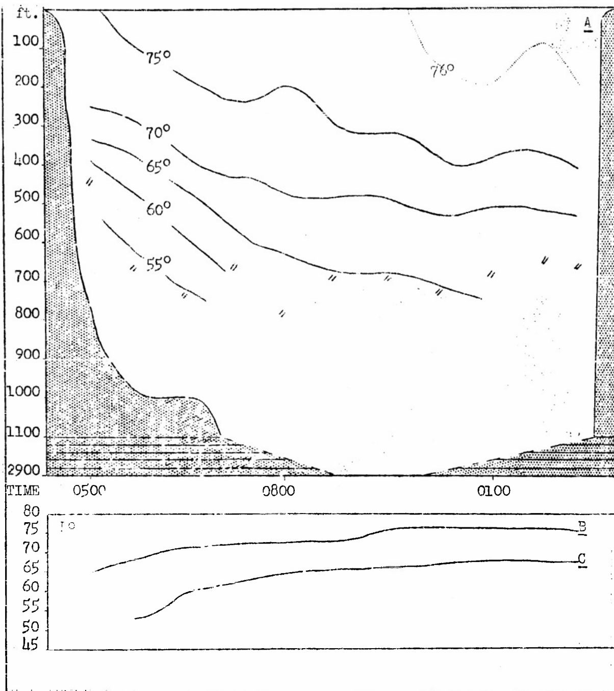
Figure 8. A TEMPERATURE-DEPTH PROFILE B&C TEMPERATURES AT 100 AND 200 METERS Data from Cruise T-307 N. Bimini to Miami January 21, 1953.
