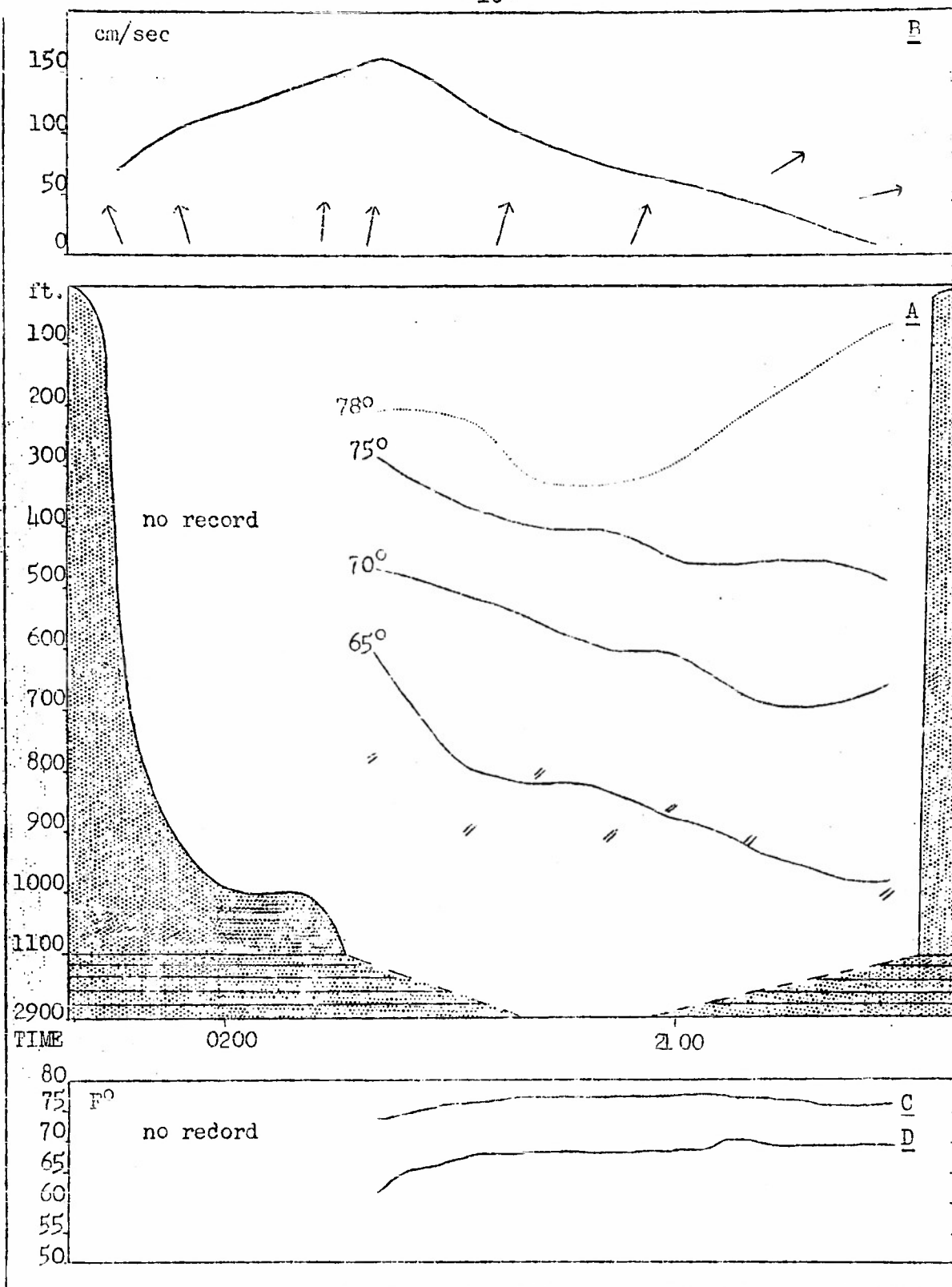
Figure 12. A TEMPERATURE-DEPTH PROFILE B CEK VECTORS C&D TEMPERATURES AT 100 AND 200 METERS Data from Cruise T-315 Cat Cay to Miami March 12, 1953.
