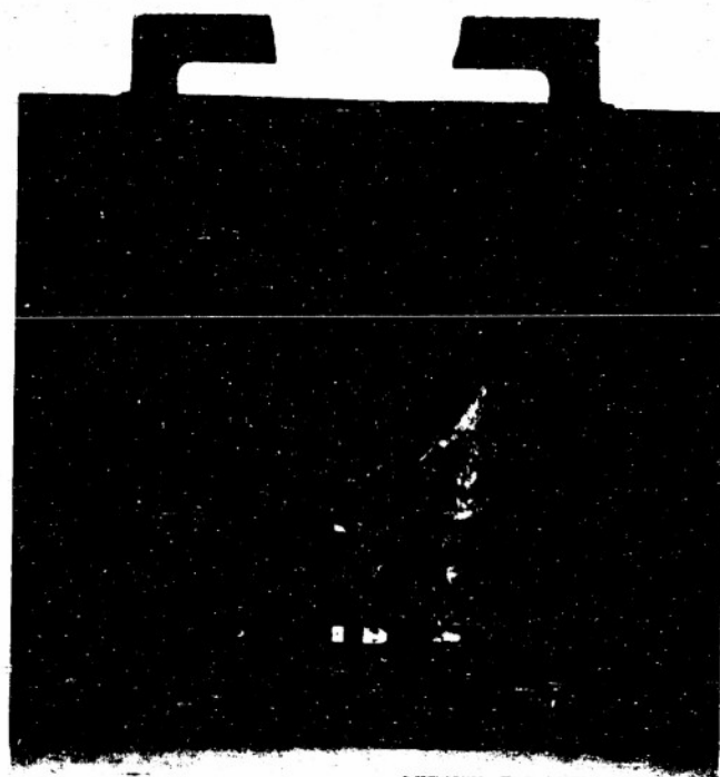
Plate 11 SK beam 3E welded with preheat, tested at -115^{\circ}\text{F} . Complete fracture at deflection of 0.47 in. Early test using welded angles to hold loading block, fracture outside
