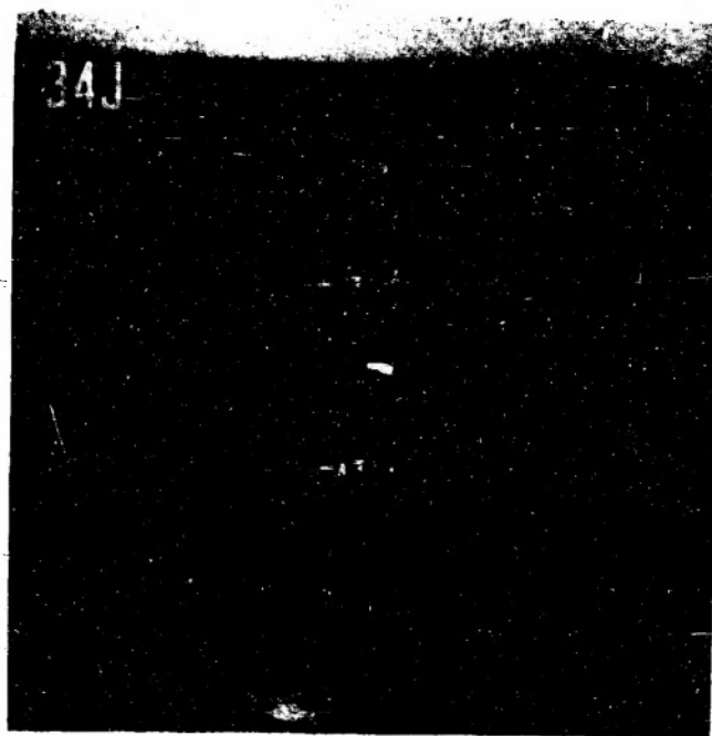
Plate 10 SK beam 5E1 stress relieved and tested at -118^{\circ}\text{F} . Complete fracture at deflection of 0.60 in.
