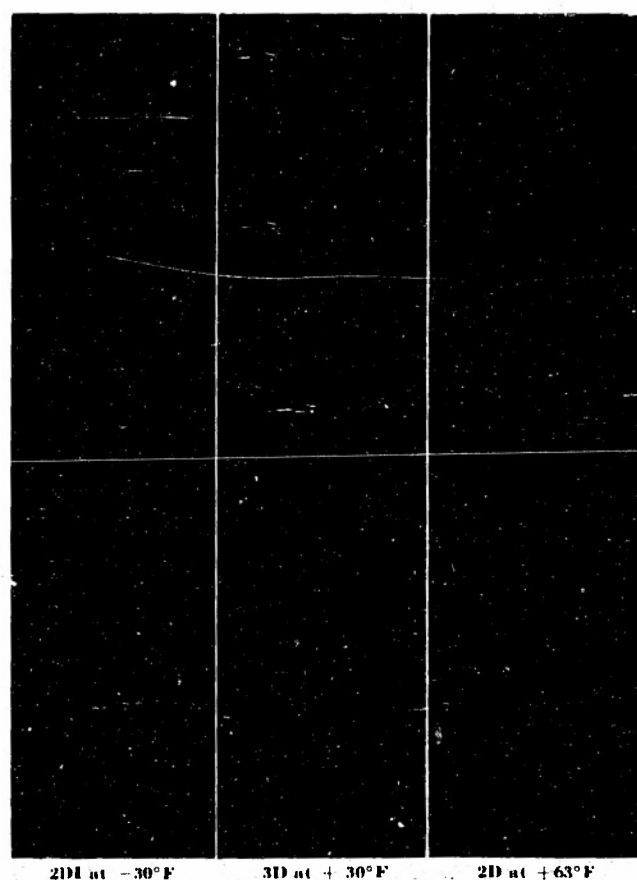
Plate 19 Fractures in unwelded and notched Beams, FK series
