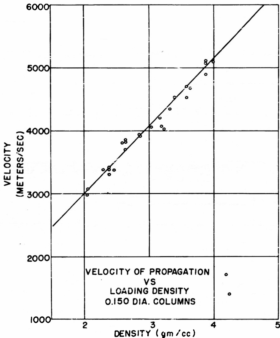
FIG. 8 EXPLOSIVE REACTIONS OF MERCURY FULMINATE
