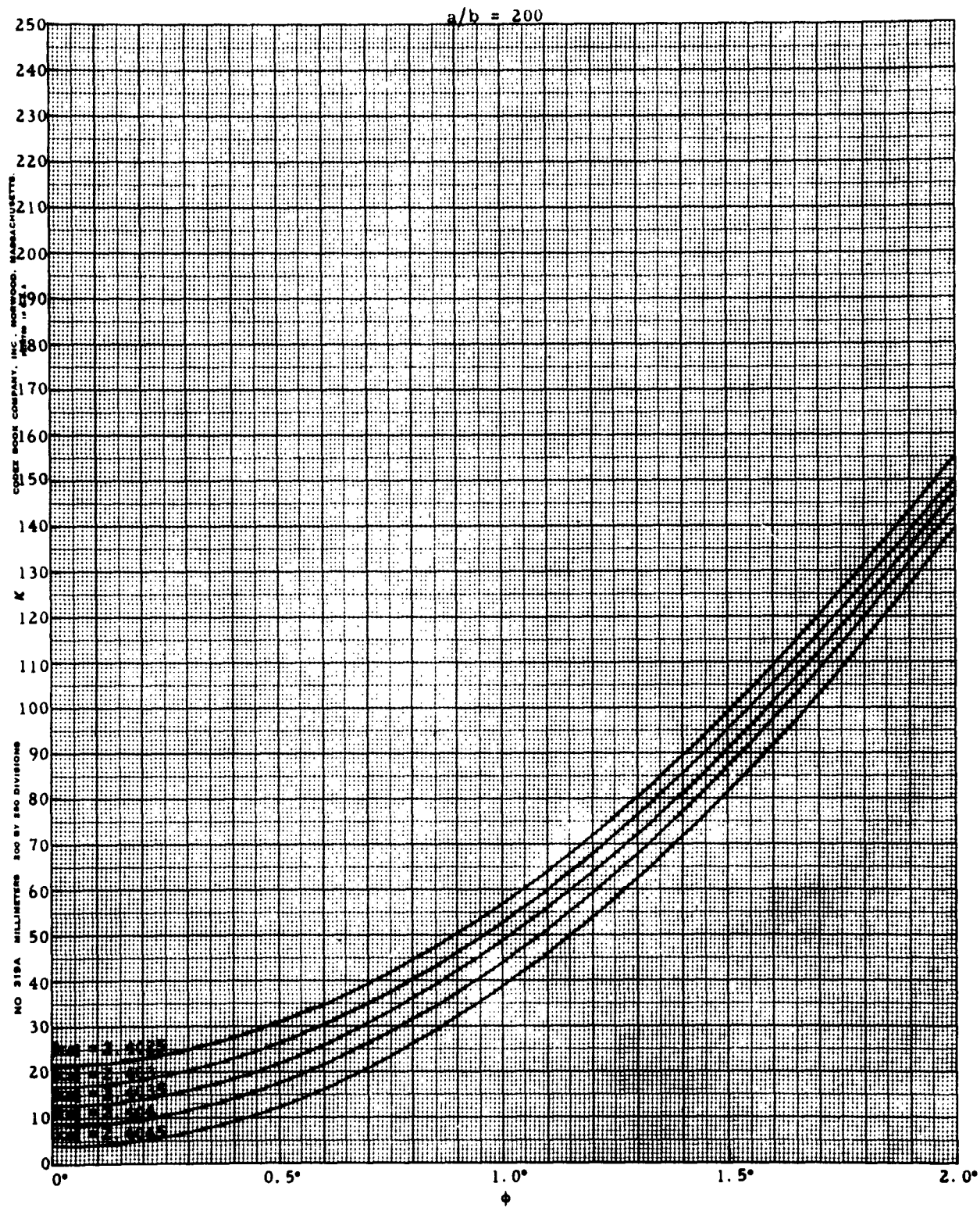
Fig. 11 \kappa vs \phi for a/b = 200
