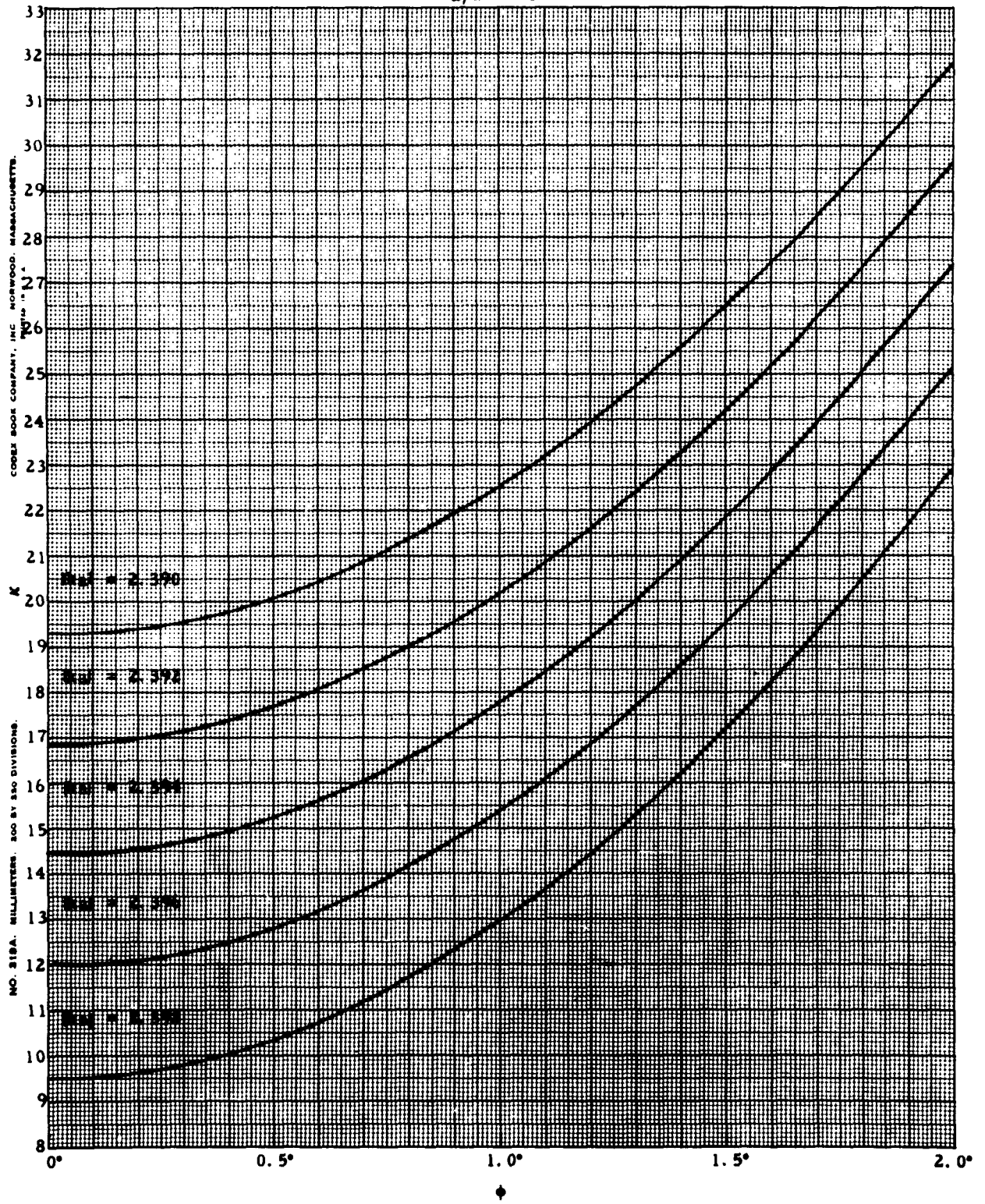
Fig. 7 \kappa vs \phi for a/b = 75
