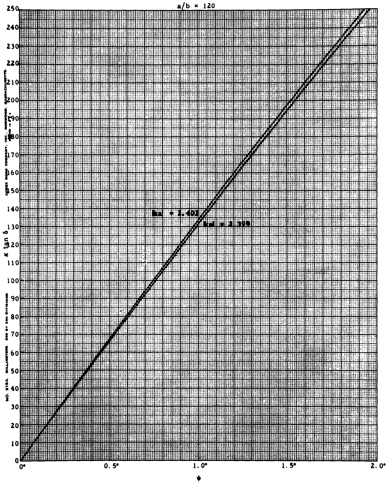
Fig. 15 \kappa \tan \delta \cos \phi for a/b = 120
