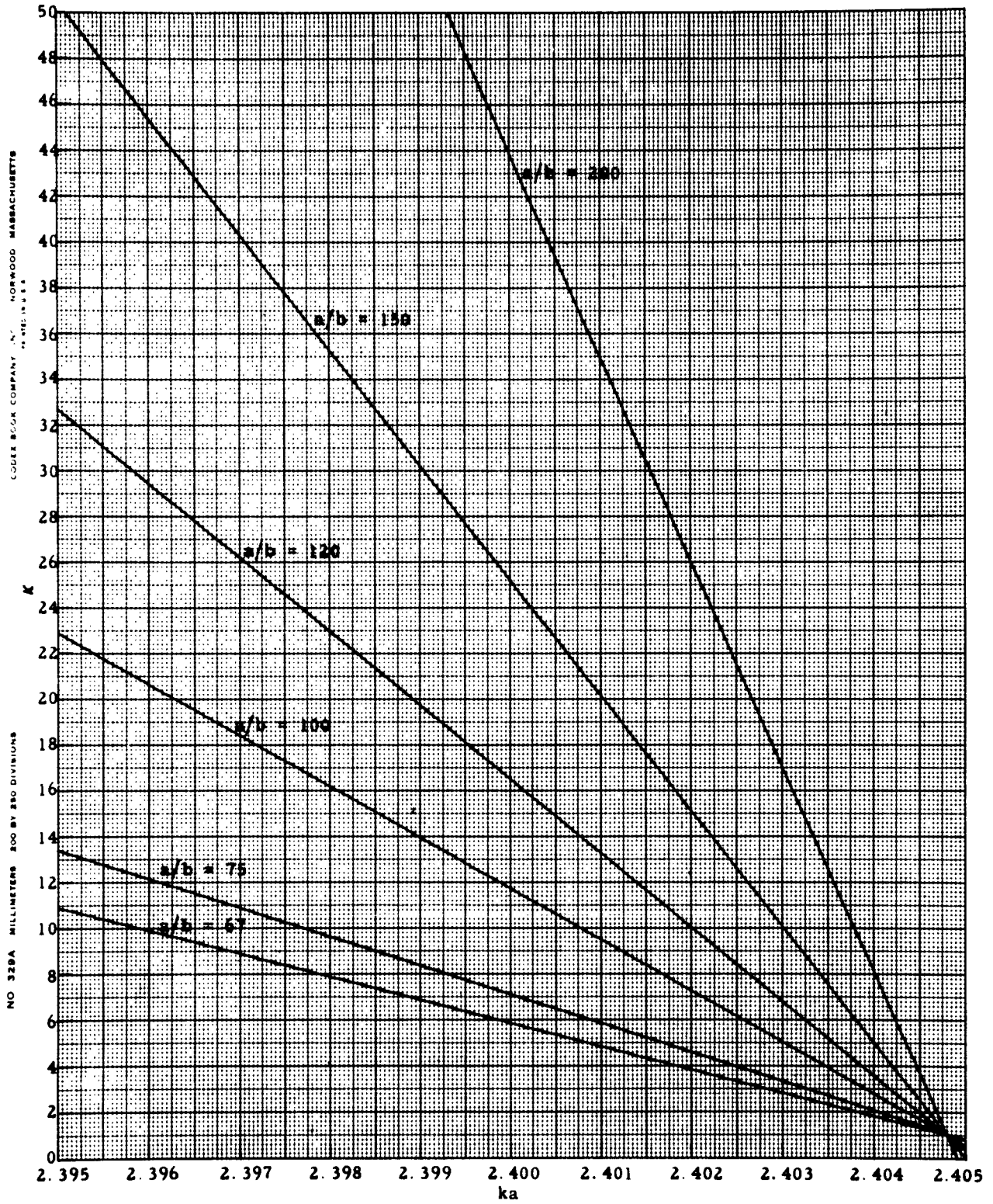
Fig. 1 κ vs ka obtained from Eq. (14)
