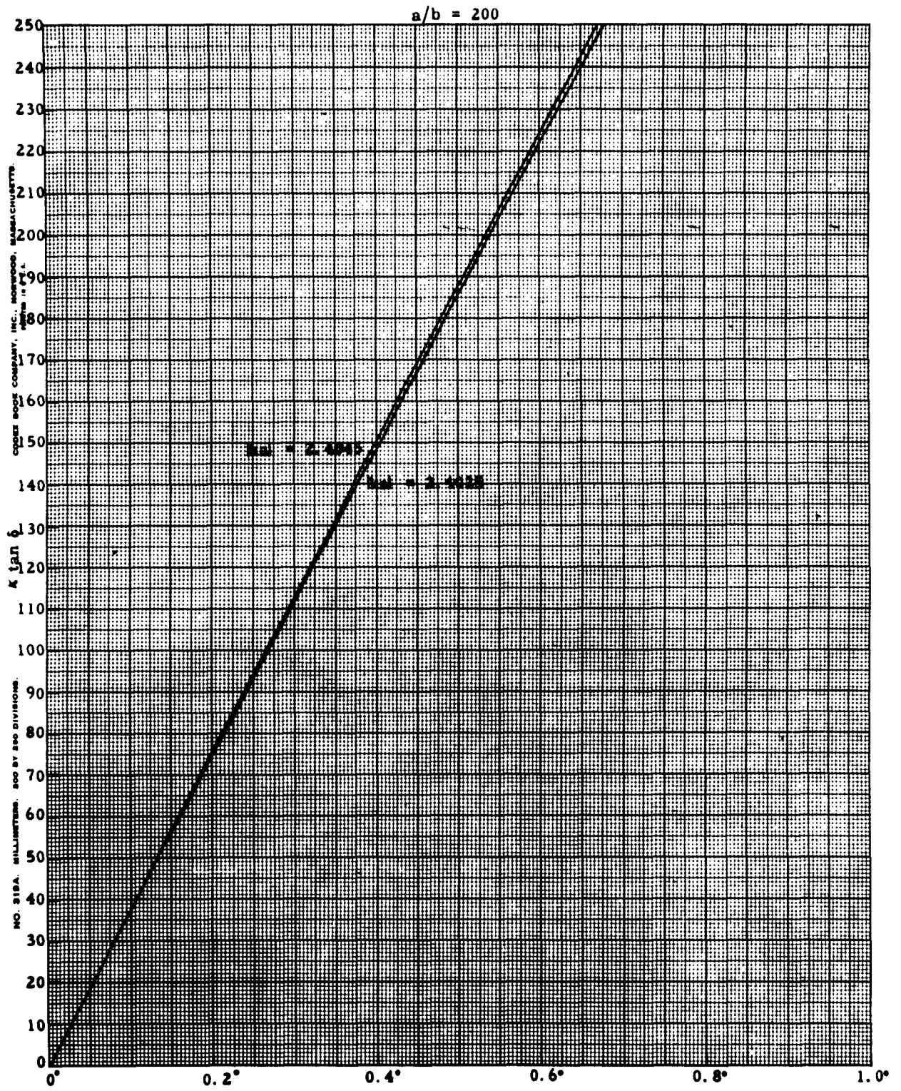
♦ Fig. 17 \kappa \tan \delta \cos \phi for a/b = 200
