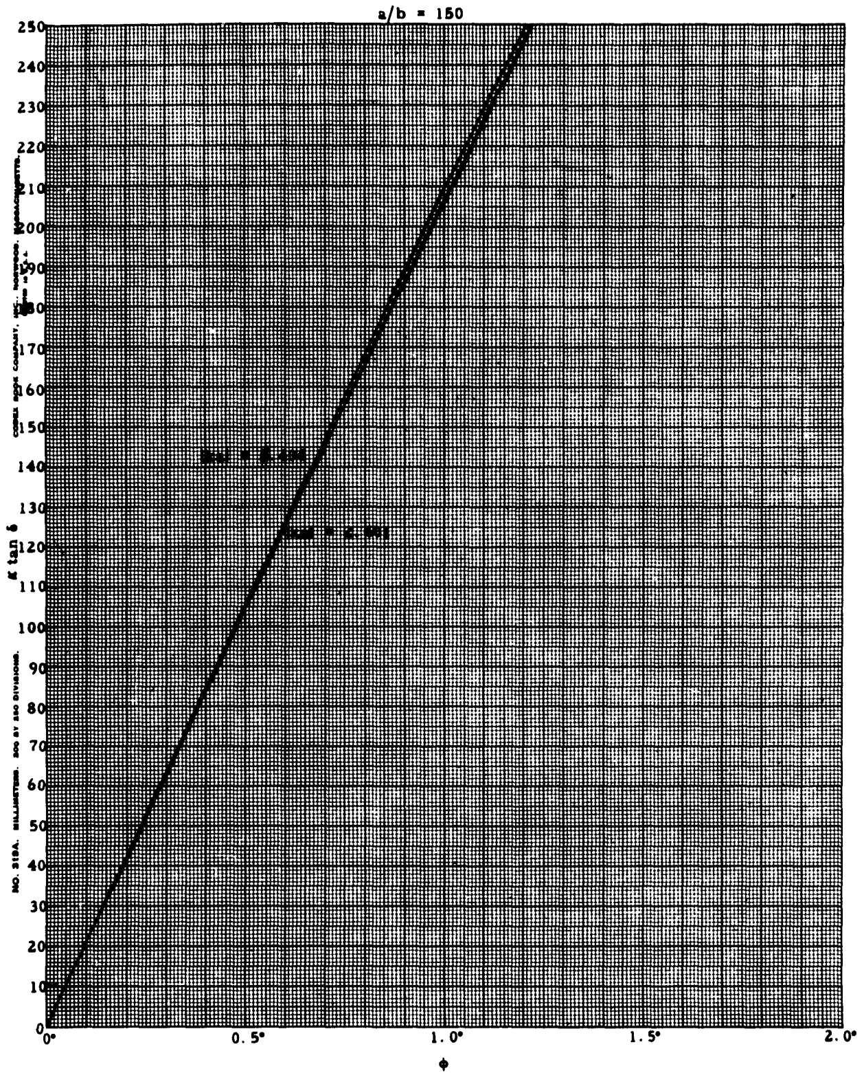
Fig. 16 \kappa \tan \delta \cos \phi for a/b = 150
