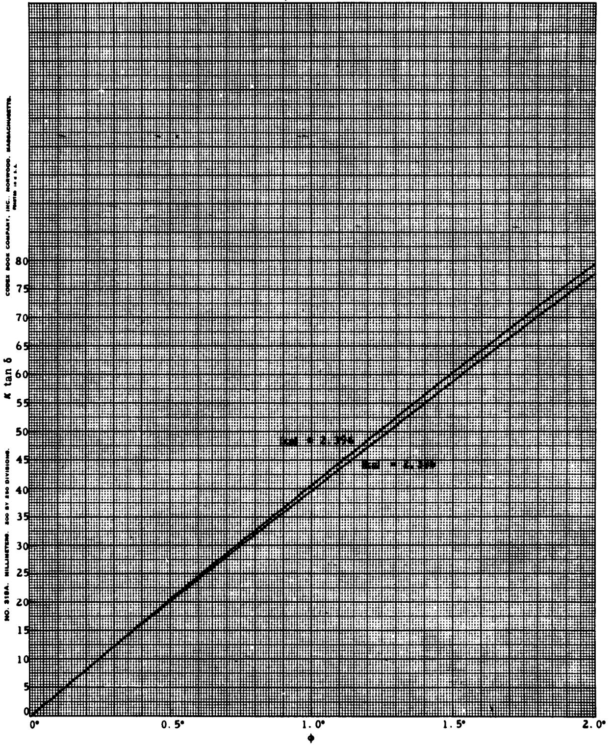
Fig. 12 \kappa \tan \delta \cos \phi for a/b = 67
