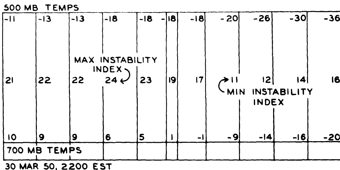
Fig. 35. Thermal cross section illustrating the instability index value and the "profile" of indices along the axis perpendicular to the 700-mb northwest flow. (The indices shown are from the axis in Fig. 33.)
