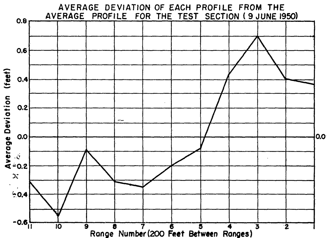
FIG. 5-AVERAGE PROFILE AND DEVIATION-LEADLINE DATA
