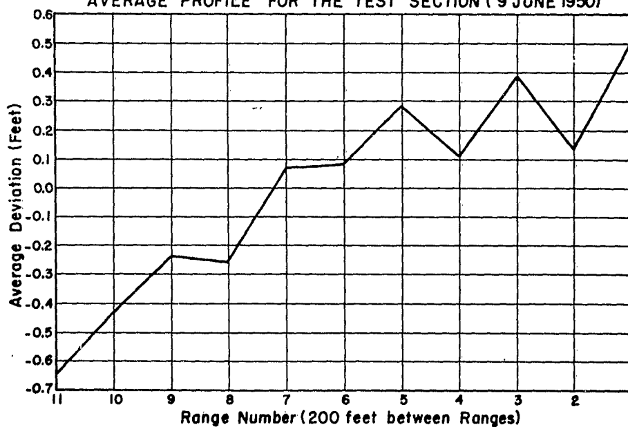
FIG. 4 - AVERAGE PROFILE AND DEVIATION-SONIC DATA
