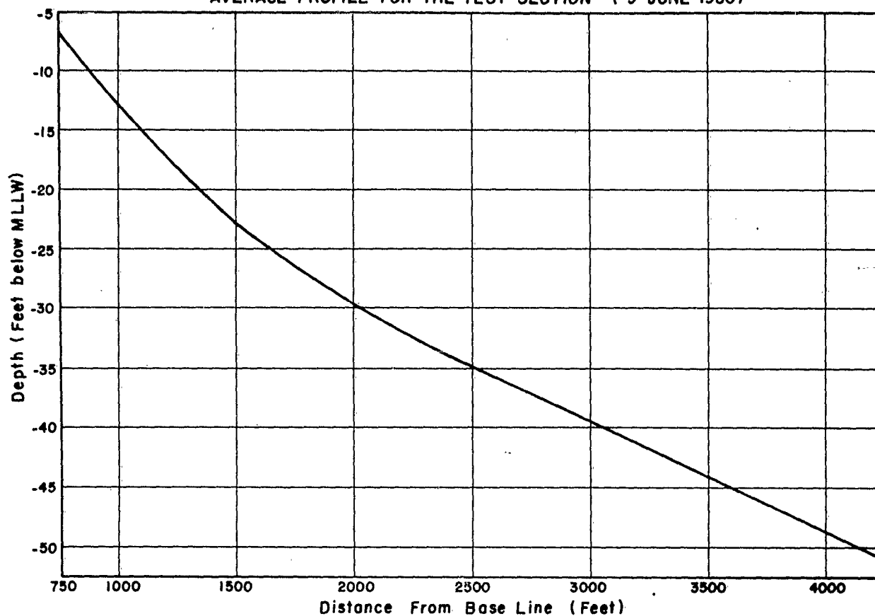
AVERAGE PROFILE FOR THE TEST SECTION ( 9 JUNE 1950)
