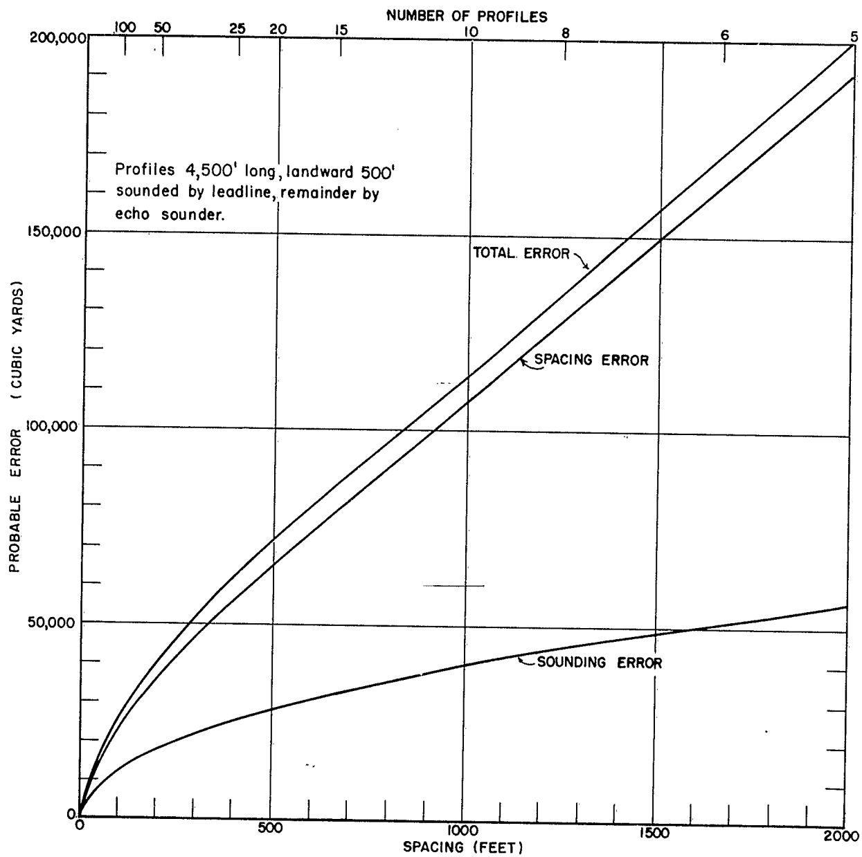
FIG. 8 - PROBABLE VOLUME ERRORS FOR 10,000-FOOT BEACH
